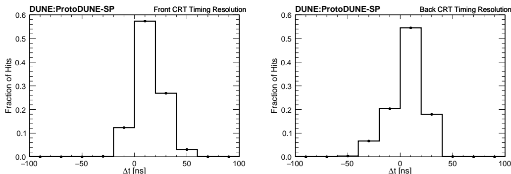
Figure 53. Timing resolution for CRT reconstructed hits on the front CRT modules (left) and on the back CRT modules (right) from data taken in November 2018.
