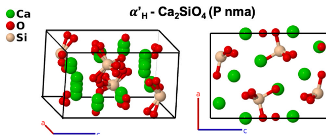
Fig. 4. Crystal structure of \alpha'_H -C 2 S (ICSD: 82997) structure data from [60].
