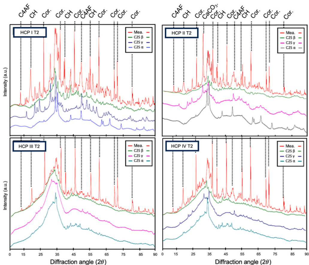
Fig. 5. XRPD pattern of HCPs after thermal activation at T2 (600°C), measured pattern in red (Mea.) and calculated profiles for C 2 S-α, C 2 S-β, C 2 S-γ. Other crystalline peaks identified are C4AF, CH, Cor. = corundum (internal standard), CaCO 3 .
