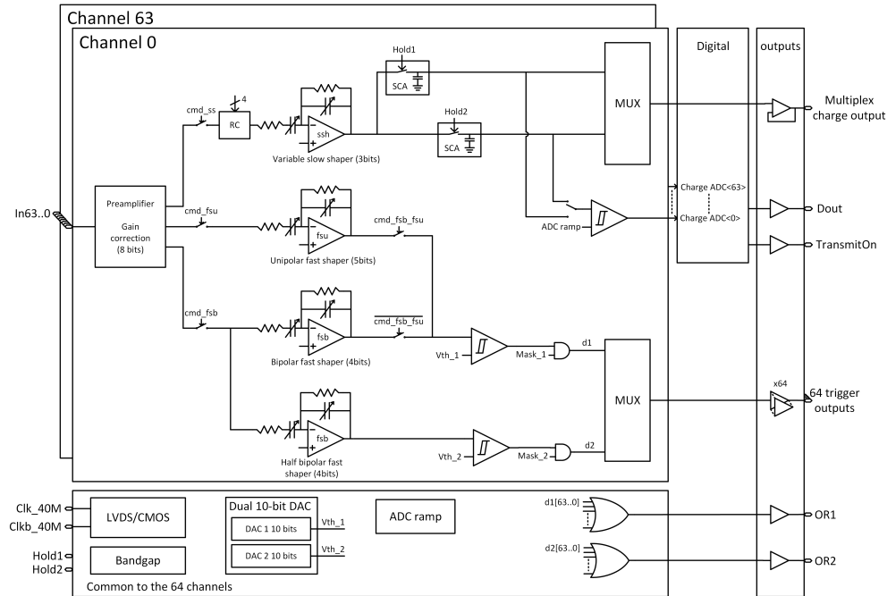
Figure 2.3: MAROC block scheme.
