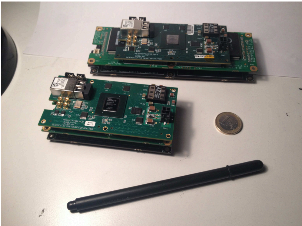
Figure 2.10: RICH electronics assemblies view.
