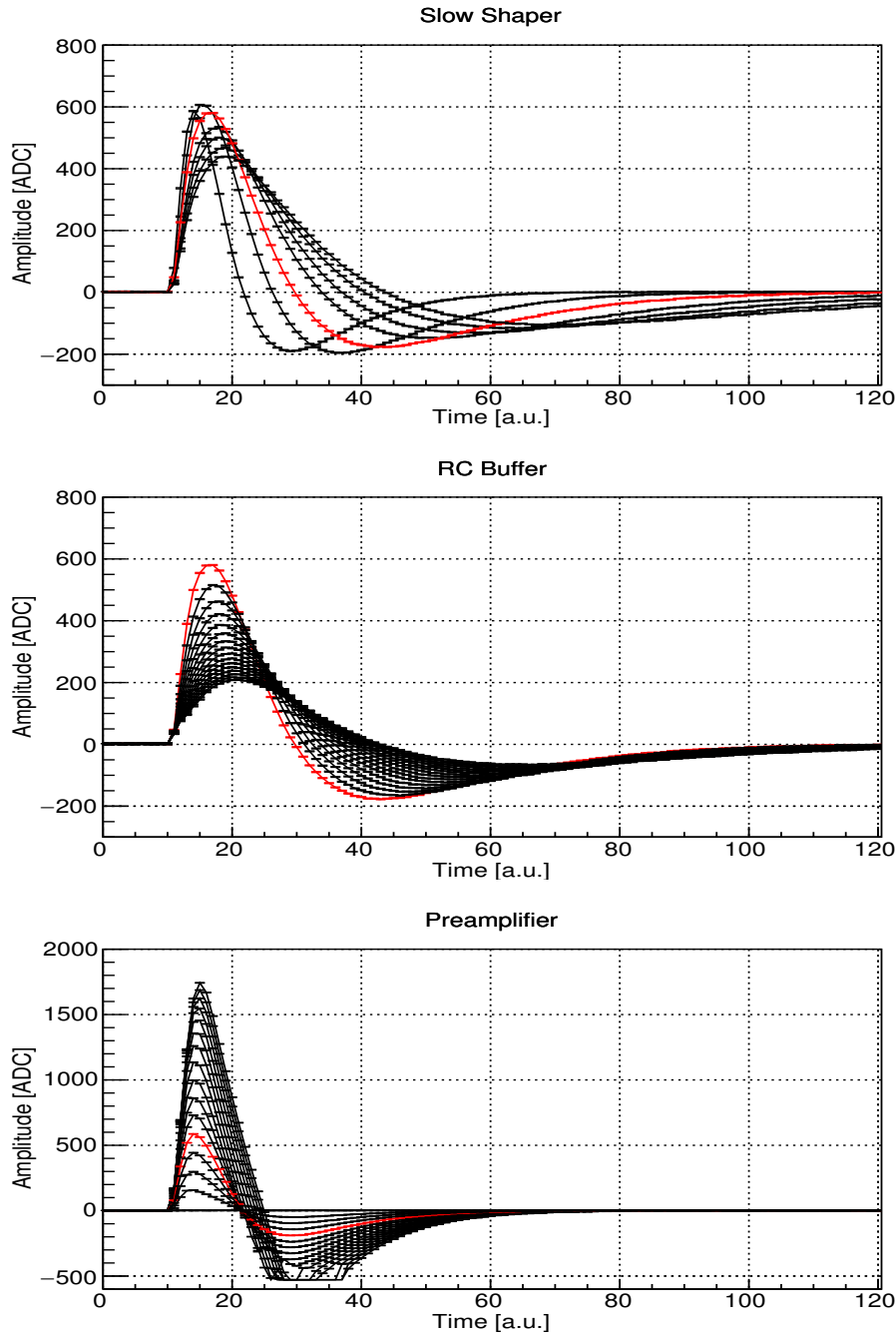
Figure 3.11: Reconstructed waveforms for different shaping parameter of the MAROC slow channel. Injected charge pretty high i.e. 825 fC to highlight the lost of shaper linearity for high preamplifier gain (bottom plot) and the possibility to attenuate using the RC buffer (central plot). In red the adopted choice guarantees an adequate linearity on the ADC data. Time is in clock tick units (8 ns).
