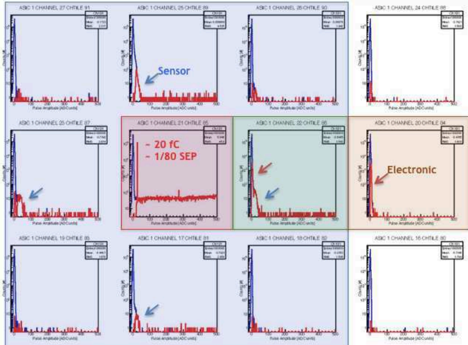
Figure 4.8: Optical and Electronic crosstalk.
