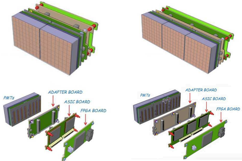
Figure 2.1: MAPMT tile assembly mechanical drawing (2014).
