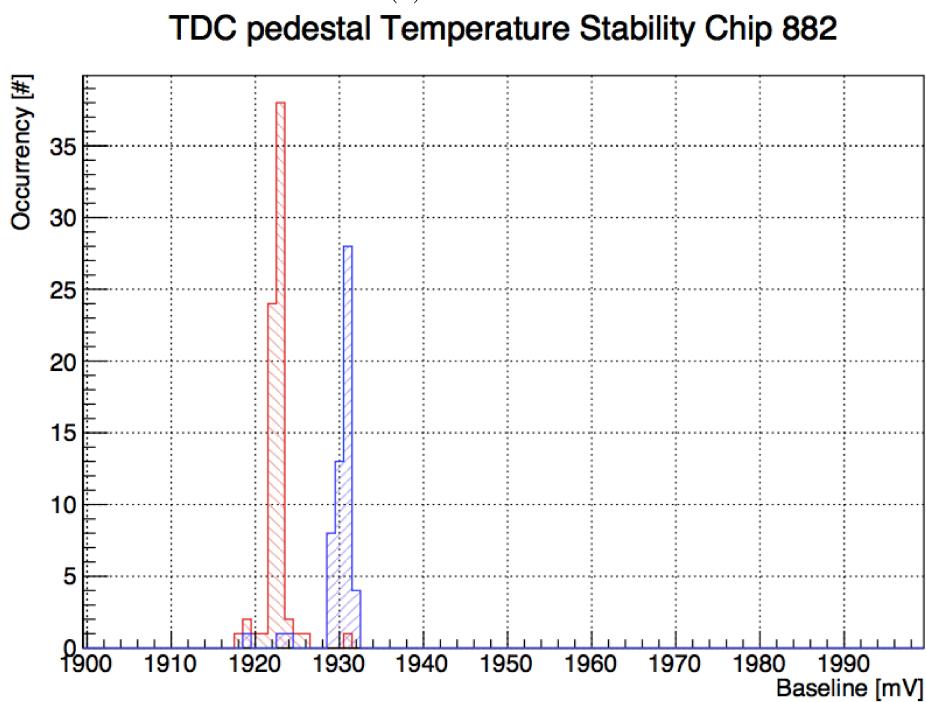
(b) TDC baseline
