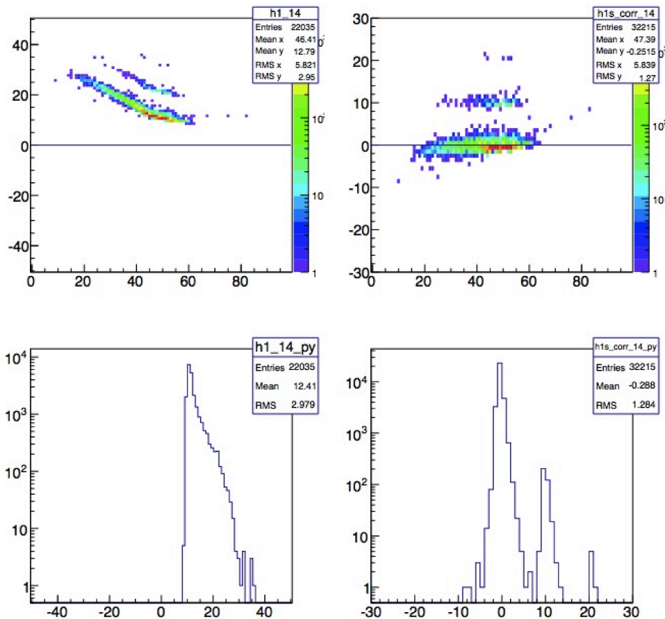
Figure 4.6: Time walk correction. Hit distribution before and after correction (bottom) in nanosecond units. Top plots show the hit time as a function of the duration i.e. the charge. The minor delayed spots are delayed laser emission as was verified independently with an oscilloscope.
