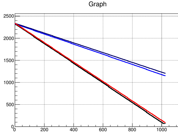
Figure 3.2: Characterization of MAROC 10 bit DAC, common to the 64 channels and used to generate the voltage level for signal discriminating. The plot presents the output voltage in millivolts as a function of the DAC word for two chips. The different DAC operating modes have different colors, in blue the FINE mode, in red the COARSE full range mode.
