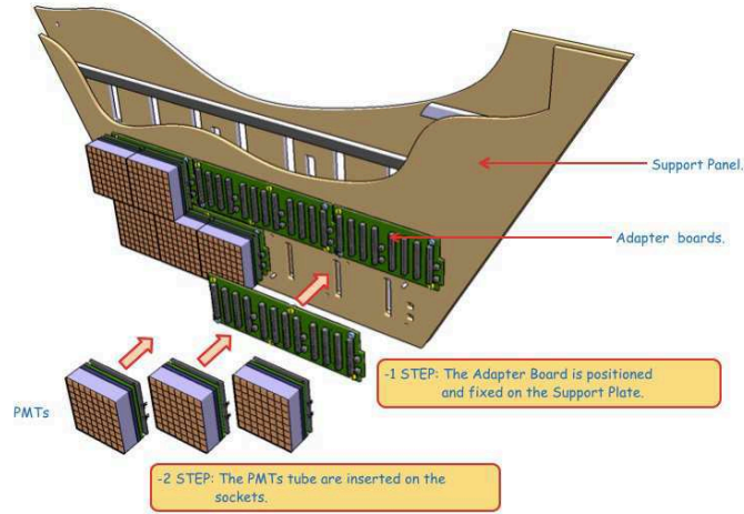
Figure 1.11: Electronic panel mounting sequence (simplified).
