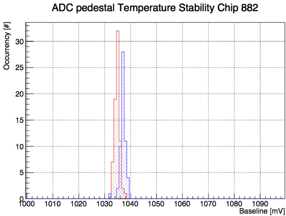
(a) ADC baseline
