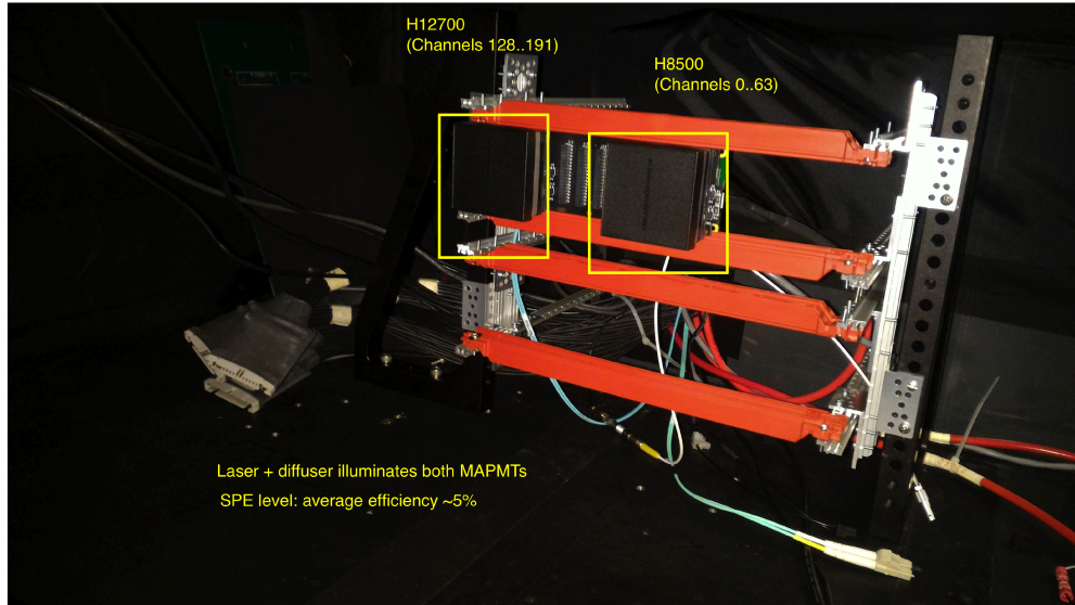
Figure 4.1: Laser characterization setup.
