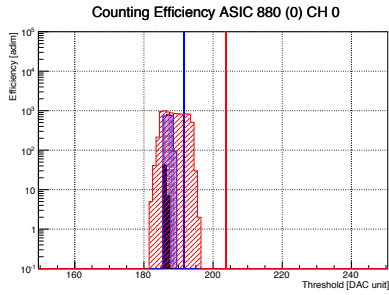
(a) Pedestal counts distribution for a single channel as a function of the threshold for three different gains.
