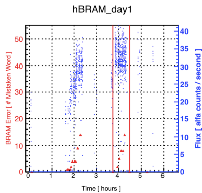
Figure 5.14: Day 1 irradiation profile.
