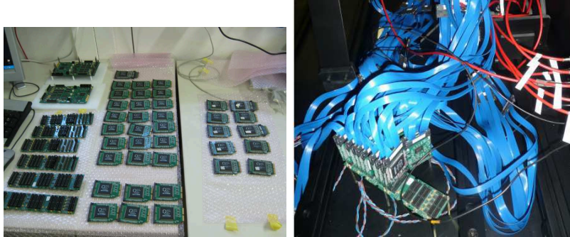
Figure 5.4: Left plot: the various components of the MAROC3 electronics. Right plot: the assembled setup installed in the RICH prototype box.
