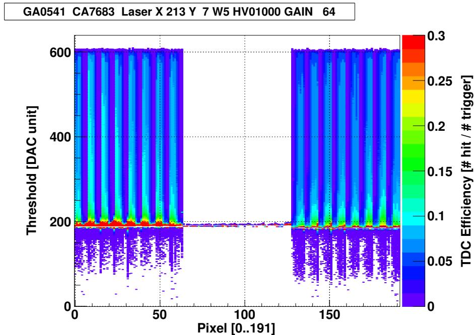
Figure 4.3: Laser detection efficiency as a function of the individual pixel of the MAPMT ( x -axis) and of the common MAROC threshold y -axis. No preamplifier gain correction is applied to equalize pixels, G = 64 correspond to unitary gain for all the channels. TDC data (July 2016, JLAB).
