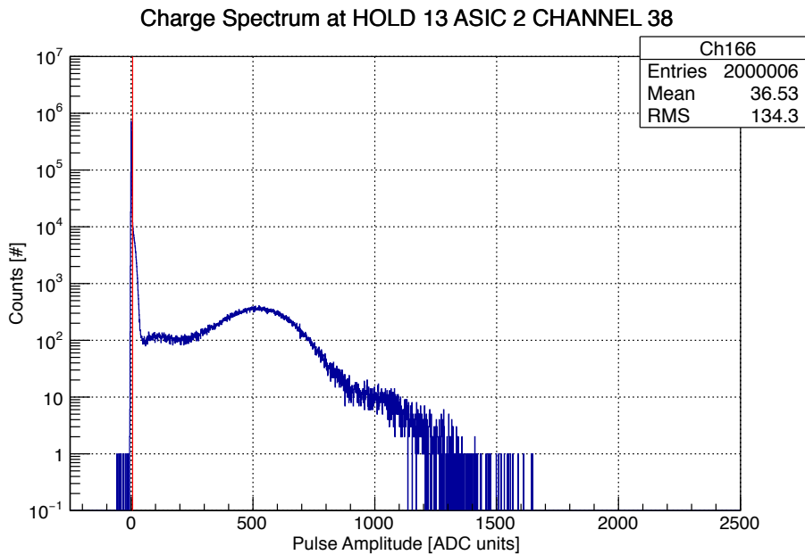
(b) H12700 individual pixel pulse amplitude spectrum
