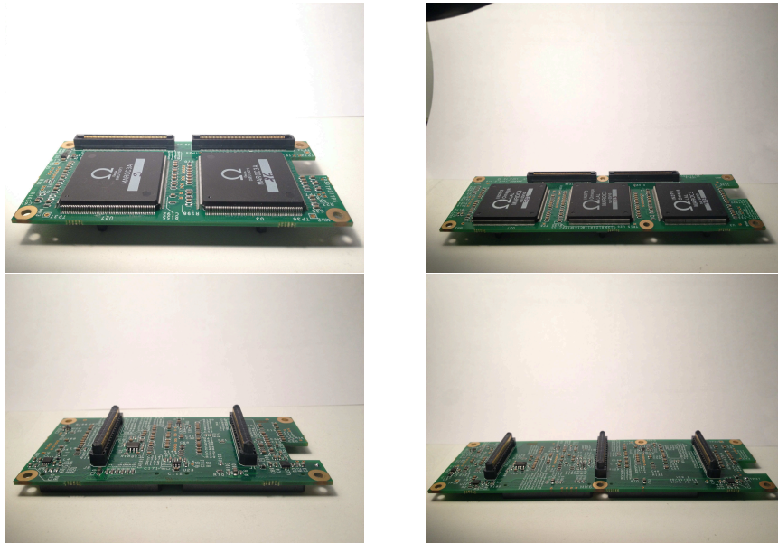
Figure 2.4: MAROC boards layout view.
