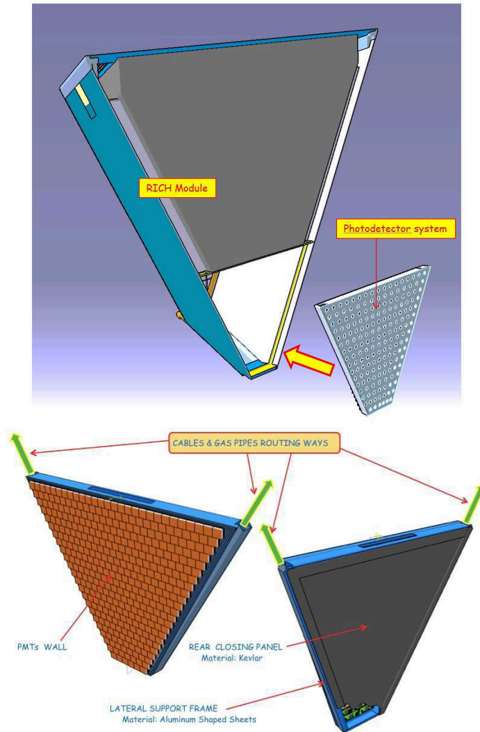
Figure 1.10: Electronics panel supporting the active area of the RICH detector. Sensors and Electronics are in the acceptance. Power and data cabling as well as and gas pipes routing is realized along later raceway in the shadow of the forward detector frame.
