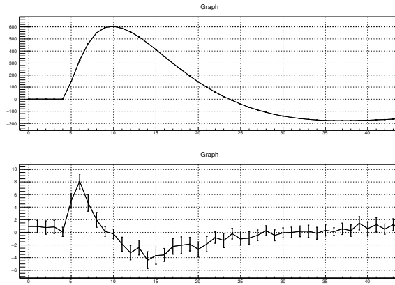
Figure 3.15: Crosstalk measurement using ADC waveform reconstruction mode. Amplitude in ADC units and time in clock ticks units (8 ns).
