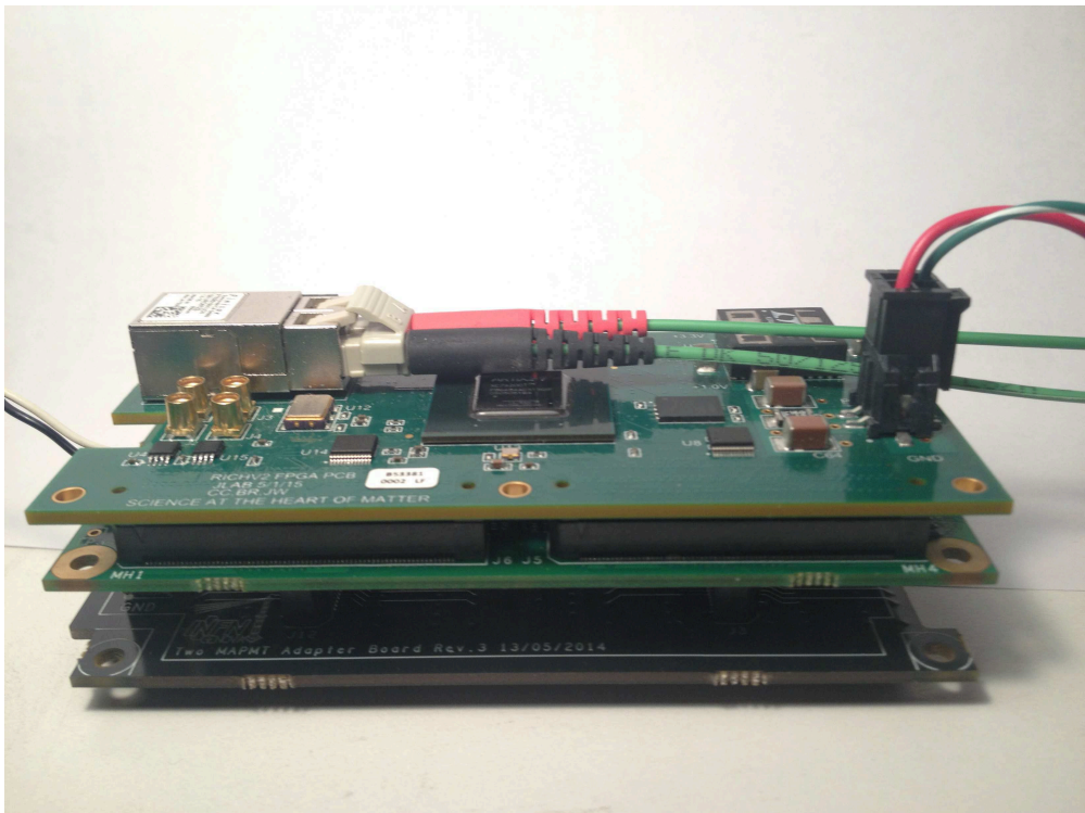
Figure 2.8: RICH electronics tile, 128 readout channels variant.
