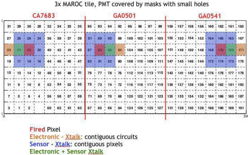
Figure 4.7: Crosstalk setup.
