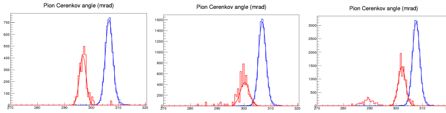
Figure 5.10: Pion Cherenkov angle distributions (in mrad, blue histograms) compared with those from events with gas Cherenkov signal below threshold (red histograms), for P = 6, 7, 8 GeV/c beam (from left to right).
