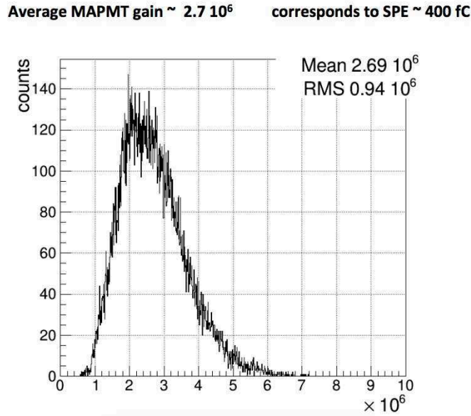
Figure 3.9: Histogram of the amplification gain of the 391 MAPMTs used for the first RICH sector construction. A single photo electron (SPE) produces on average 400 fC pulses.
