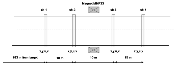
Figure 2.6: The Straw Tracker layout.
