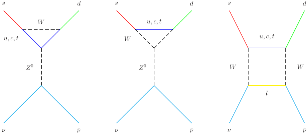
Figure 1.3: Graphs for s \rightarrow d\nu\bar{\nu} in the Standard Model.
