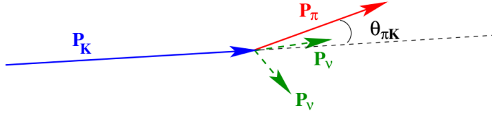
Figure 1.6: Kinematics of the decay under study.
