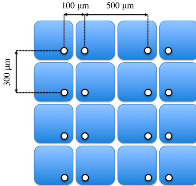
Figure 3.4: Bump pads arrangement scheme.
