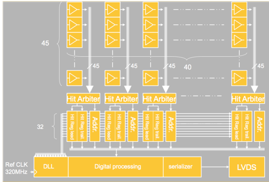
Figure 3.7: EoC architecture block diagram.
