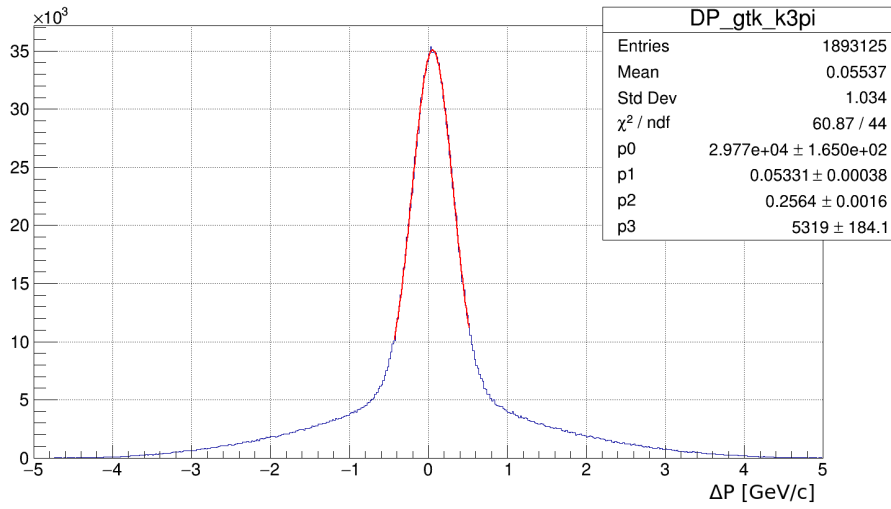
Figure 5.9: Difference in reconstructed momenta ( |p_{GTK}| - |p_{K3\pi}| ).
