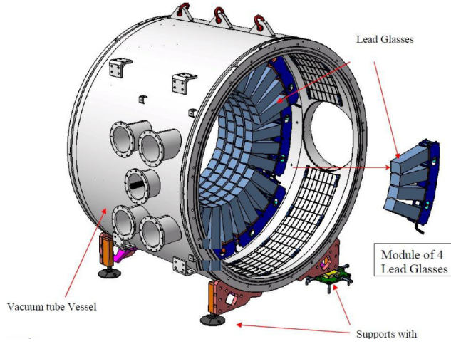
Figure 2.5: LAV: Complete station layout.
