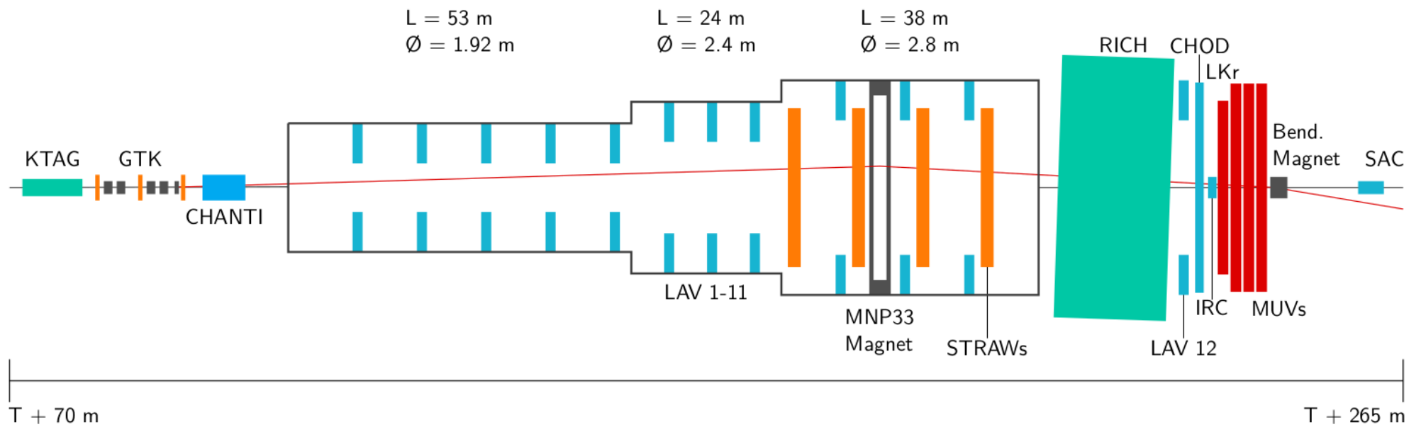
Figure 2.1: Longitudinal view of the NA62 experimental setup.
