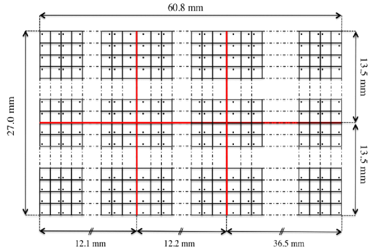
Figure 2.4: Layout of the GigaTracker sensors.
