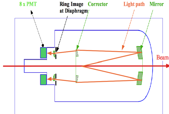
Figure 2.2: Schematic layout of KTAG detector.
