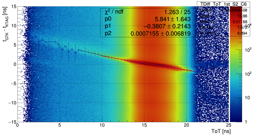
Figure 5.3: Example of a time-walk fit.
