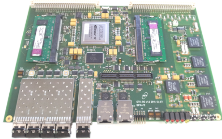
Figure 3.9: The GTK-RO motherboard.
