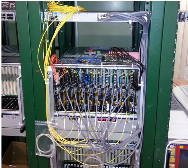
Figure 4.7: VME crate with first 10 GTK-RO boards installed in Bldg. 918’s PC Farm room at the end of October 2014.
