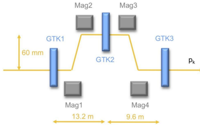
Figure 2.3: Layout of the GigaTracker stations.
