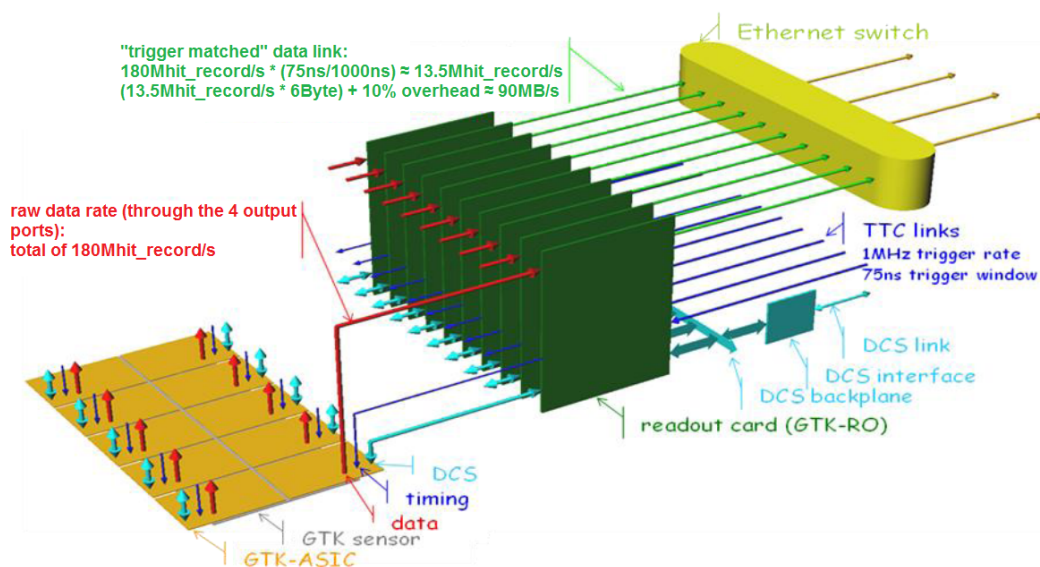
Figure 3.10: GTK read-out block diagram.
