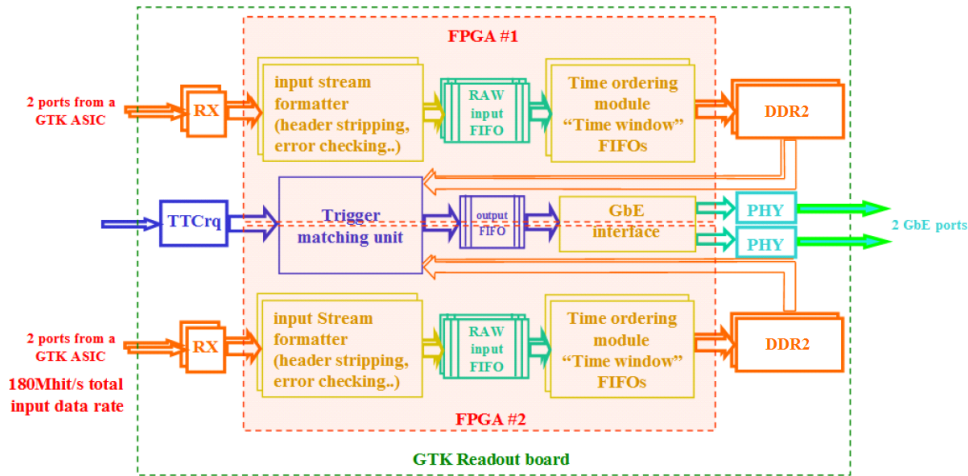
Figure 3.11: GTK read-out board block diagram.
