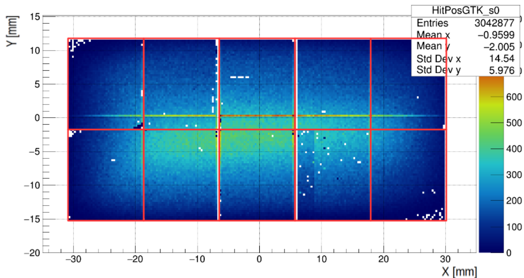
Figure 5.13: Matched GigaTracker hit map. In red the boundaries of the TDCpix chips are displayed. One can note an inefficient band (quarter chip) in the 4th chip from the left on the bottom.
