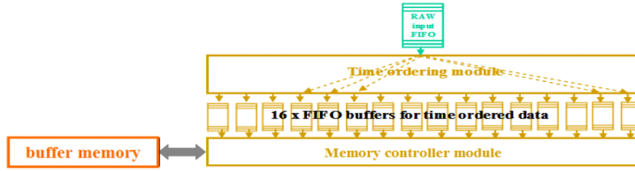
Figure 3.12: Block diagram of time ordering.
