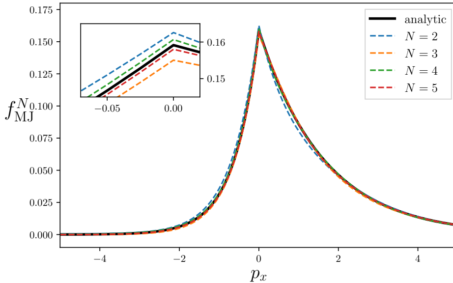
Figure 2.1: Comparison of the analytic Maxwell Jüttner distribution in (2 + 1) dimensions against approximations at various orders N , computed using an orthogonal polynomial basis. The distributions are shown as functions of \mathbf{p} = (p_x, 0) , having fixed all the other parameters to m = 0 , T = 1 , n = 1 and \beta = |U^i|/U^0 = 0.5 .
