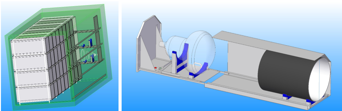
Figure 17: Left Conceptual picture of the container with the shelf system including 36 drawer boxes. Right Schematic view of the final design of the drawer system (for illustrative reasons one side of the drawer box is not depicted).
