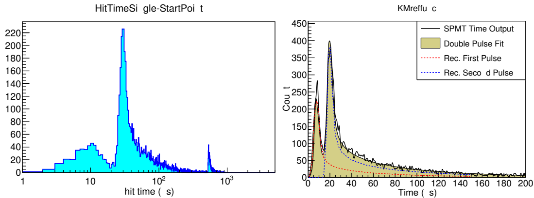
Figure 10: Left: sample of hit time distribution after TOF correction. double signal pile-up shape should be observed. The third signal in around 500 ns comes from the Michel electron. Right: sample of Multi-pulse fitting. The time difference of both signal is 11 ns.
