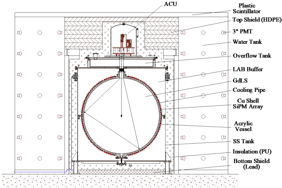
Figure 32: Schematic view of the T O detector, which consists of a Central Detector (CD) and an outer shielding and veto system. The CD consists of 2.8 ton gadolinium-doped LS filled in a spherical acrylic vessel and viewed by 10 \text{ m}^2 SiPMs, a spherical copper shell that supports the SiPMs, 3.45 ton buffer liquid, and a cylindrical stainless steel tank insulated with 20 cm thick Polyurethane. The outer shielding includes 1.2 m thick water in the surrounding tanks, 1 m High-Density Polyethylene on the top, and 10 cm lead at the bottom. The water tanks, instrumented with Photomultipliers, and the plastic scintillator on the top comprise the active muon veto system. The triangle and central axis inside the detector show the reach of the calibration.
