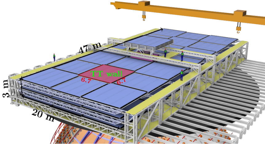
Figure 13: The JUNO Top Tracker.
