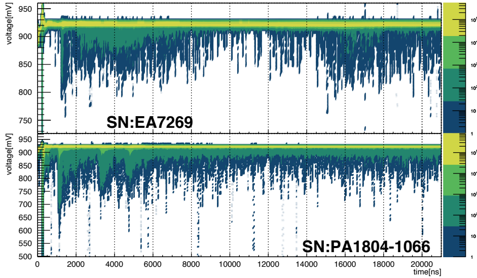
Figure 21: Two dimensional plot of the afterpulse waveforms, for a dynode PMT with serial number of E 7269 (upper) and a MCP PMT with serial number of P 1804-1066 (lower)
