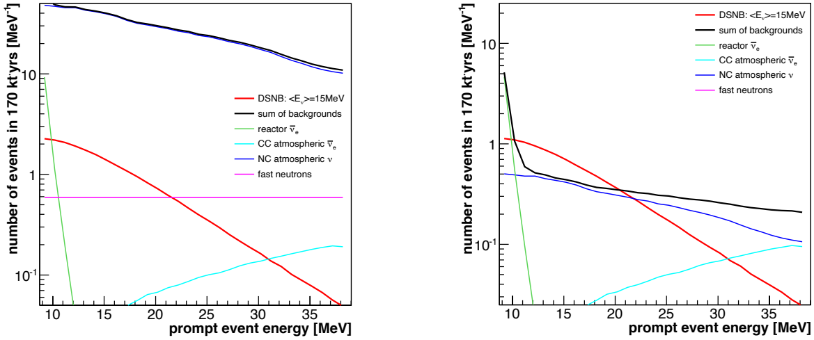
Figure 5: Prompt ( e^+ ) energy spectra for the DSNB signal ( \langle E_\nu \rangle = 15 MeV) and backgrounds as expected for JUNO. Left After basic selection cuts, the background from atmospheric-neutrino NC reactions dominates over the whole range of the observation window from 10 to 30 MeV. Right When applying pulse shape discrimination, atmospheric neutrino NC and fast neutron backgrounds are greatly reduced. The DSNB signal dominates in the range from 11 to \sim 22 MeV.
