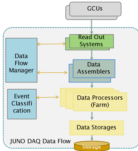
Figure 28: The D Q data flow consisting of four levels of scalable and distributed data processing including the readout systems, data assemblers, data processors, and data storages, and two centralized data processing including the data flow manager and the event classification.
