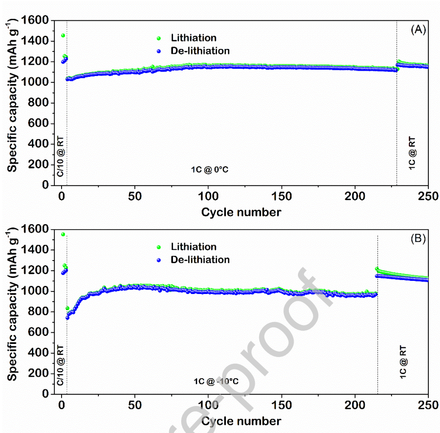
Fig. 7. Long cycling behaviour of the nanostructured Ge anode at the current rate of 1C in the 0.01–1.5 V voltage range at 0°C (A) and -10°C (B).
