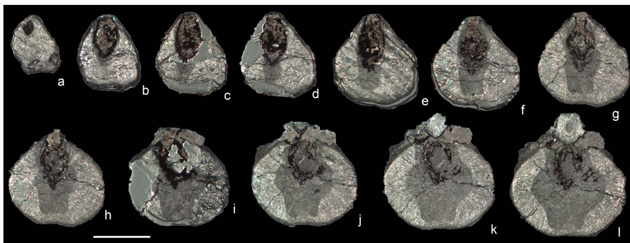
Fig. 12 - Transcaucasathyris lata (Grunt in Ruzhentsev & Sarytcheva, 1965), serial sections of the specimen MPUM12279. Distance from the umbo: a) 0.6 mm, b) 1 mm, c) 1.2 mm, d) 1.3 mm, e) 1.4 mm, f) 1.6 mm, g) 1.7 mm, h) 1.8 mm, i) 1.9 mm, j) 2 mm, k) 2.1 mm, l) 2.2 mm. Scale bar corresponds to 2 mm.
