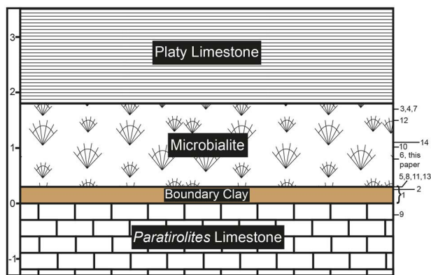
Fig. 6 - (color online) Graphic scheme showing the different positions of the PTB at Abadeh published by the authors cited in the text. The numbers refer to the different papers as in Tab. 3.
