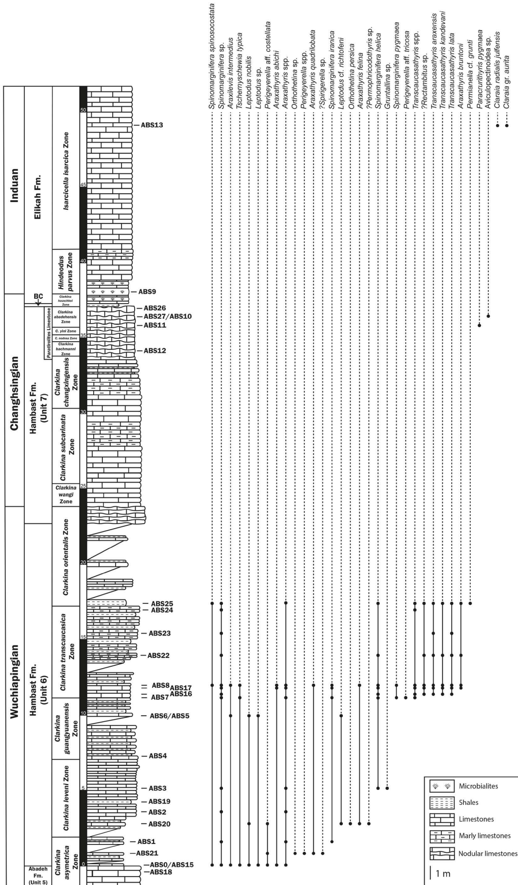
Fig. 5 - Composite stratigraphic section at Abadeh.
