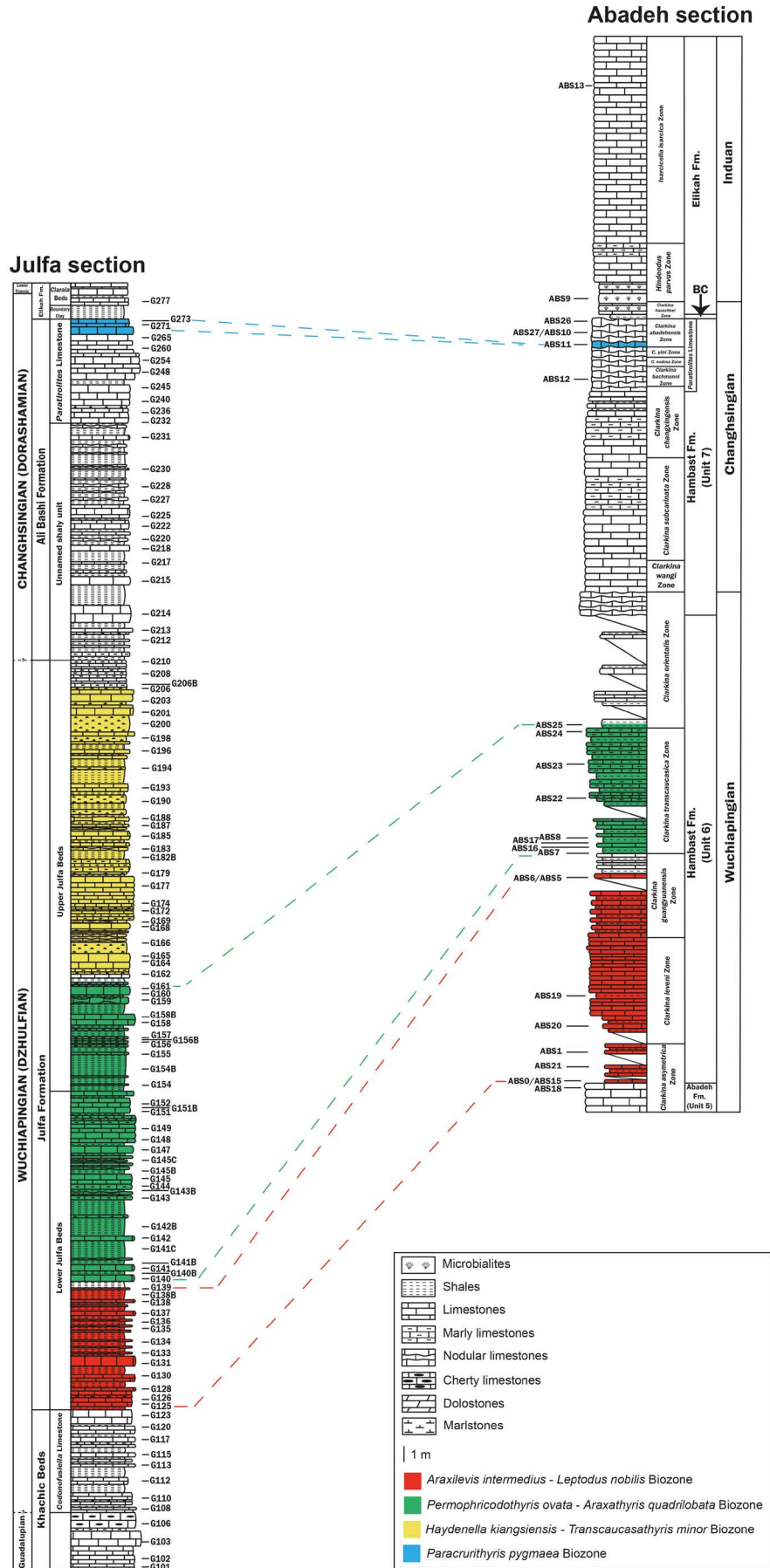
Fig. 9 - Correlation of Julfa and Abadeh sections.
