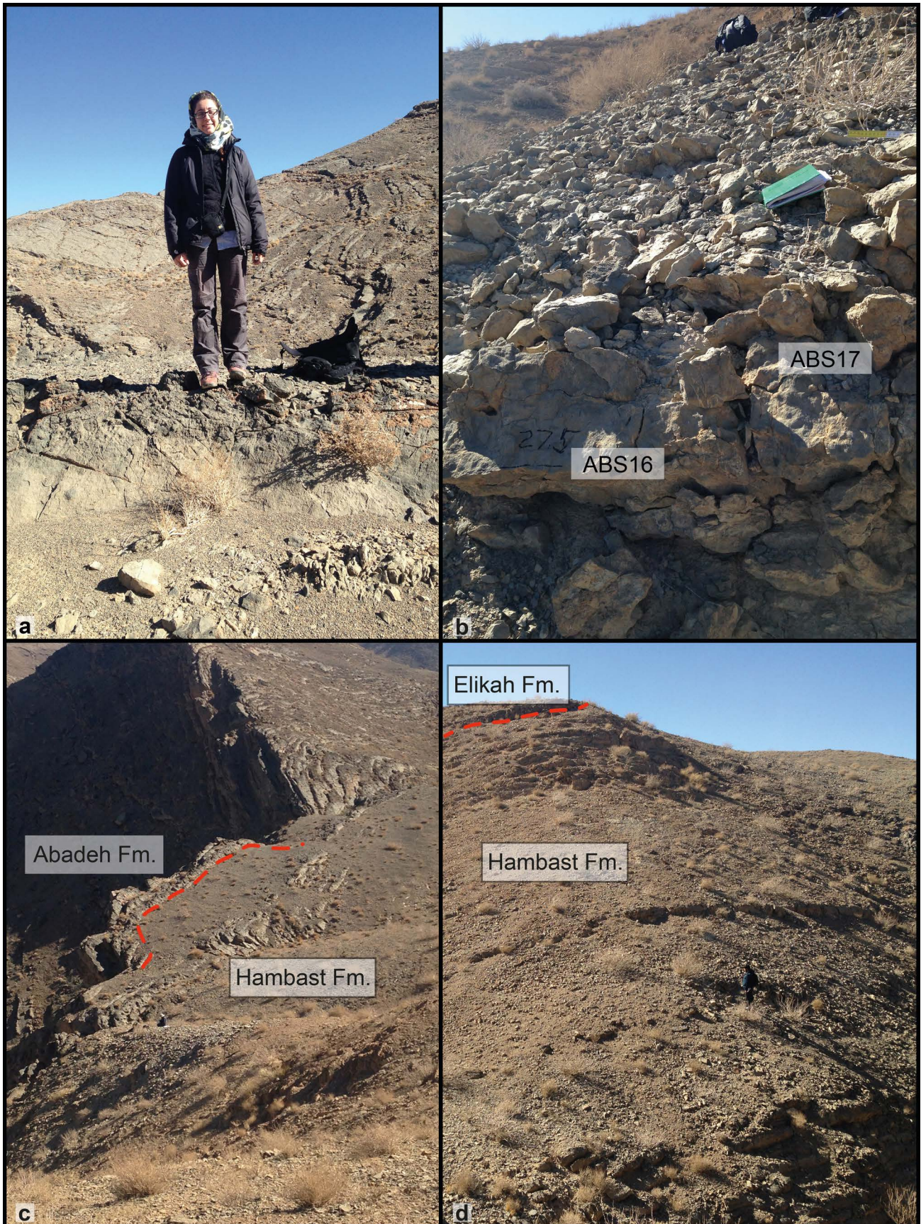
Fig. 3 - (color online) a) Dr. Gaia Crippa standing above the top of the Abadeh Formation. b) Grey limestones, position of samples ABS16 and ABS17. c) Gully section, poorly outcropping and covered by scree. d) Saddle section.
