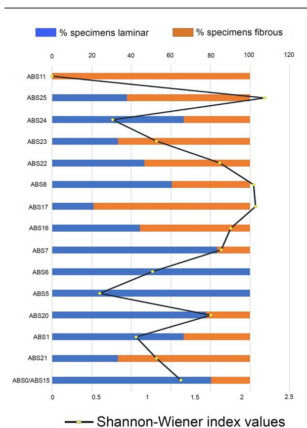
Fig. 8 - (color online) Graph showing the alternation in prevalence of laminar vs fibrous shell microstructural type.
