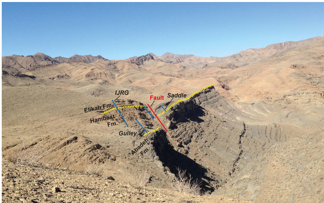
Fig. 2 - (color online) Position of the two measured logs at Abadeh.
