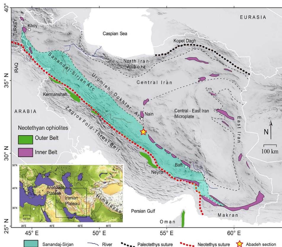
Fig. 1 - (color online) Distribution of the Neotethyan ophiolite belts in Iran. The Inner Belt is also called “Coloured Mélange”. Modified from Hassanzadeh & Wernicke (2016).
