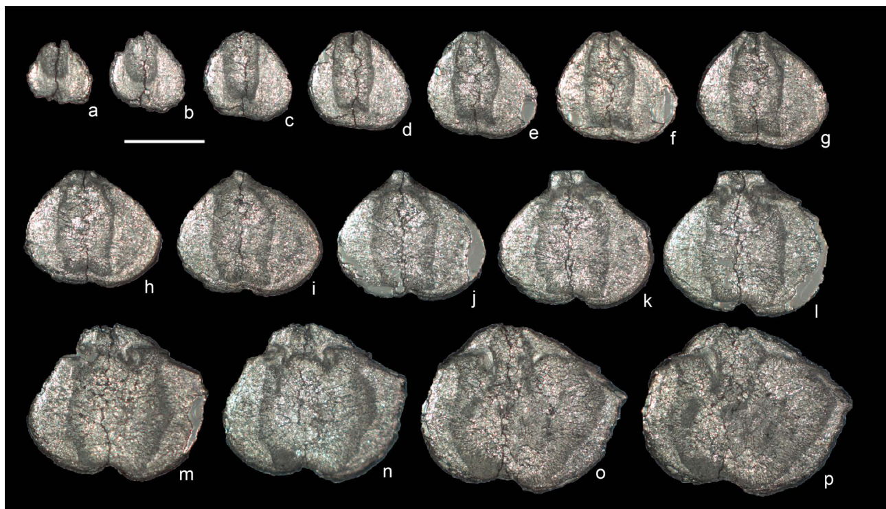
Fig. 10 - Araxathyris abichi (Arthaber, 1900), serial sections of the specimen MPUM12230. Distance from the umbo: a) 0.1 mm, b) 0.2 mm, c) 0.3 mm, d) 0.4 mm, e) 0.5 mm, f) 0.6 mm, g) 0.7 mm, h) 0.8 mm, i) 0.9 mm, j) 1 mm, k) 1.1 mm, l) 1.2 mm, m) 1.3 mm, n) 1.4 mm, o) 1.7 mm, p) 1.8 mm. Scale bar corresponds to 2 mm.
