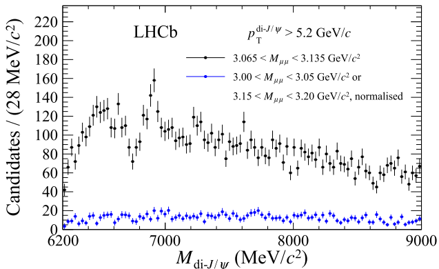
Fig. 2. Invariant mass spectrum of J/\psi -pair candidates passing the p_{\text{T}}^{\text{di-}J/\psi} > 5.2 \text{ GeV}/c requirement with reconstructed J/\psi masses in the (black) signal and (blue) background regions, respectively.
