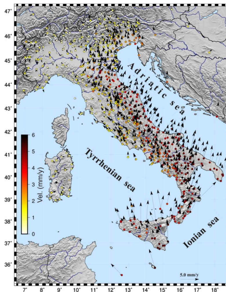
Figure 14. Horizontal velocity field in the Italian peninsula, derived by GPS data, with respect to a fixed Eurasian plate in the ITRF2014 reference frame [237]. The colours of station sites indicate velocity following the chromatic scale on the left. The description of the GPS network and data analysis is given by [250–252].
