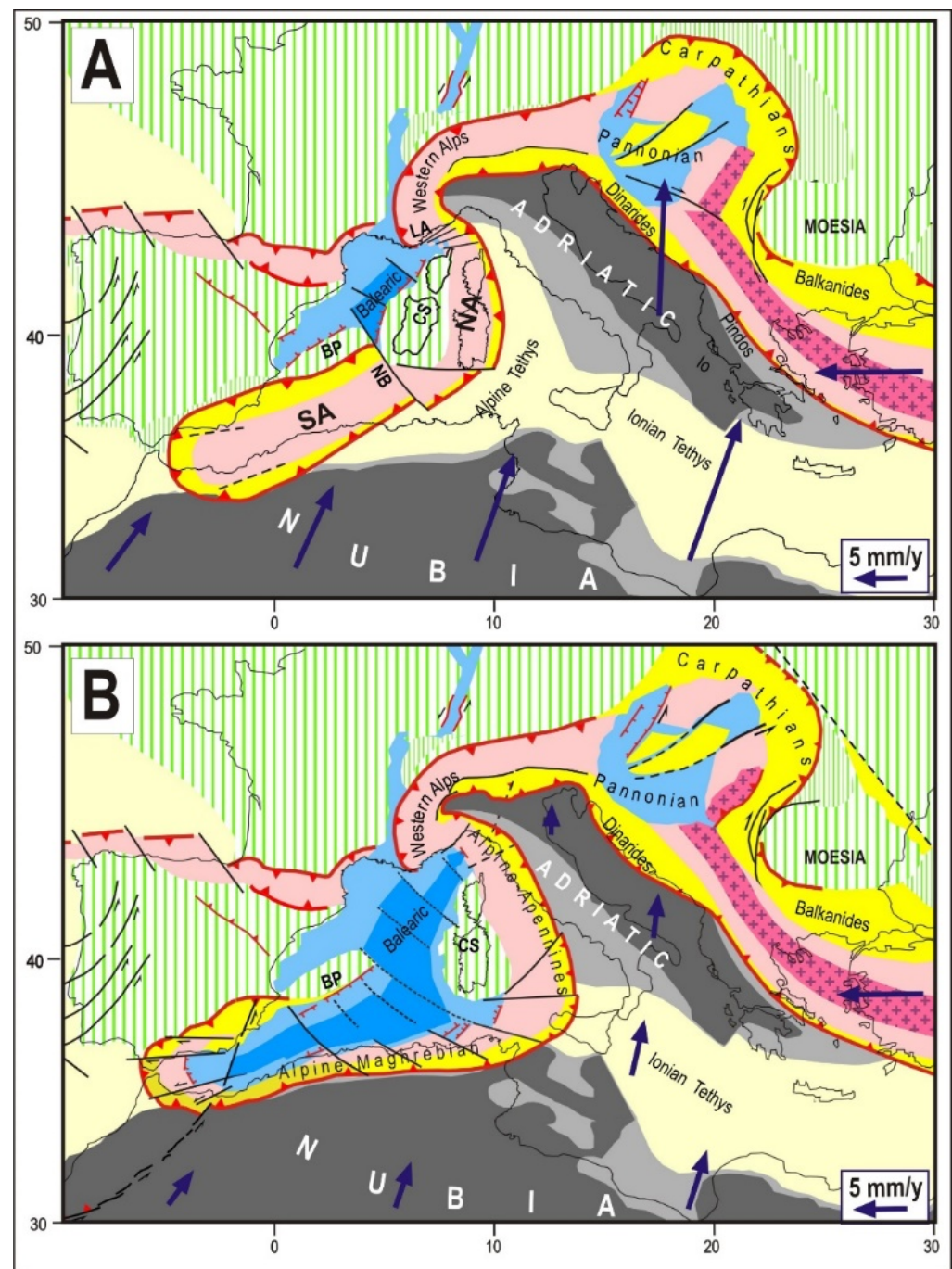
Figure 4. (A) Early Miocene. The Northern Arc (NA, Alpine–Iberian–Apennine belt) underwent a greater rotation with respect to the Southern Arc (SA, Alpine–Iberian–Maghrebian belt), allowed by the North Balearic dextral shear zone (NB). BP = Balearic Promontory, CS = Corsica–Sardinia, Io = Ionian thinned continental zone, LA = Ligurian Alps. (B) Middle–Late Miocene. After long migration and considerable bending (induced by the Nubia–Eurasia convergence) the Arc reached a configuration with two almost perpendicular segments. The Corsica–Sardinia block reached its final location, after the collision of the Northern Arc with the Adriatic continental domain (Middle Miocene). The Southern Arc stopped its migration against the continental Nubian domain (Upper Miocene). Colours and symbols as in Figure 1.
