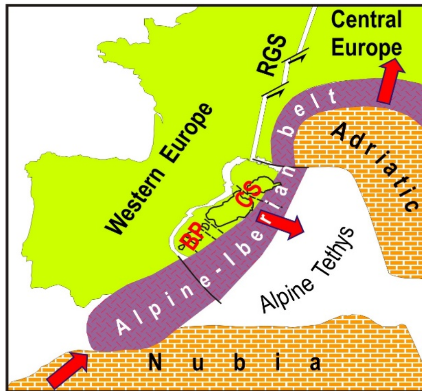
Figure 3. After the collision of the Alpine–Iberian belt with the continental African domain, the Northeastward push of Nubia was transmitted to Central Europe, causing the formation of a sinistral transtensional fault system, running from Western Europe to the Rhine Graben System (RGS). BP = Balearic promontory, CS = Corsica Sardinia.
