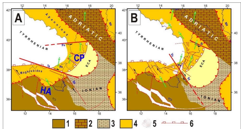
Figure 15. Tectonic sketch of the Calabria–Peloritani (CP) and Hyblean–Adventure (HA) wedges before and after the collision of Northern Calabria with the Adriatic continental domain. (1) Nubian continental domain; (2) Adriatic continental domain; (3) Ionian oceanic domain; (4) Orogenic belts; (5) Volcanism; (6) Outer fronts of the Alpine belt. (A) Early Pleistocene configuration. The lateral escape of the CP wedge (evidenced by yellow) is guided by the Taormina (Ta) and Palinuro (Pa) faults. NH = Northern Hellenides; Sy = Syracuse; Pe = Peloritani. (B) Post-middle Pleistocene tectonic setting; after the collision of Northern Calabria with the continental Adriatic domain, the extrusion trend of the CP wedge changed significantly due to the activation of two new lateral guides (Sibari (Si) and Vulcano–Syracusa (Vu-Sy) faults, e.g., [146,182,199]). The lateral guides of the CP and HA wedges are evidenced by red boldface lines. Green arrows indicate the kinematic pattern (with respect to Eurasia) which is compatible with the observed Quaternary deformations (e.g., [10,27,32]) and with the present velocity field (Figure 14). Other symbols as in Figure 1.
