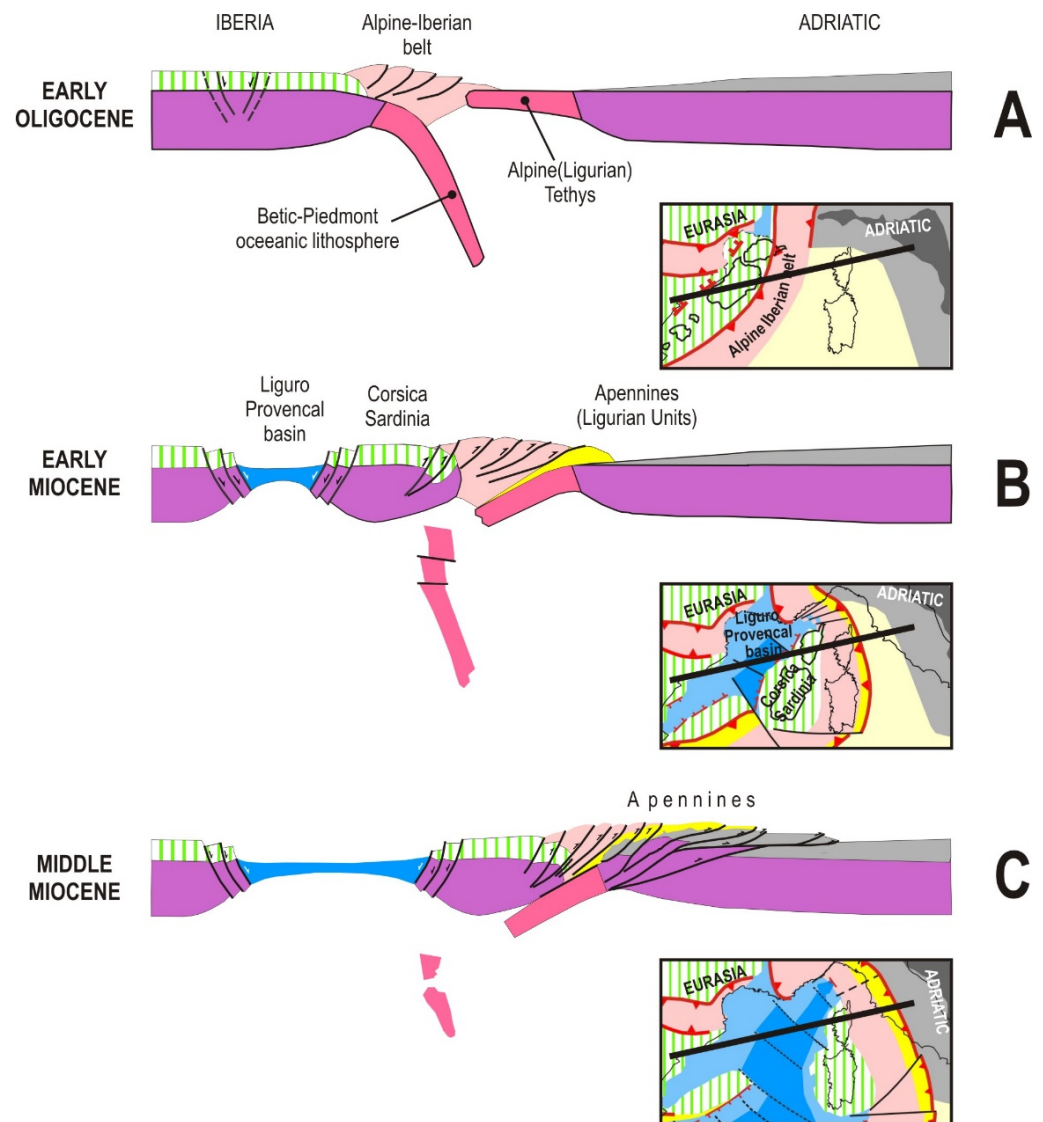
Figure 6. Tentative reconstruction, of the main tectonic processes that developed since the Oligocene along an East–West section crossing the Western Mediterranean region: (A) The old oceanic lithosphere which lay along the eastern side of Iberia is completely consumed and the Alpine–Iberian accretionary belt is formed. Crustal sinistral transtension, induced by the push of Nubia on the Alpine–Iberian belt affects the eastern margin of Iberia (see Figure 3). (B) Due to belt-parallel compression the Arc (Corsica–Sardinia–Balearic Promontory fragment and the Alpine–Iberian belt) undergoes an eastward displacement/bending, at the expense of the eastern Alpine Tethys. In the wake of the migrating Arc, crustal extension forms the Northern Balearic (Liguro–Provençal) basin, whereas the old eastward dipping slab is undergoing progressive disruption. Accretionary activity along the outer front of the migrating Arc led to the formation of the Apennine belt. (C) The stop of the Arc against the continental Adriatic domain causes the end of crustal extension in the Liguro–Provençal basin.
