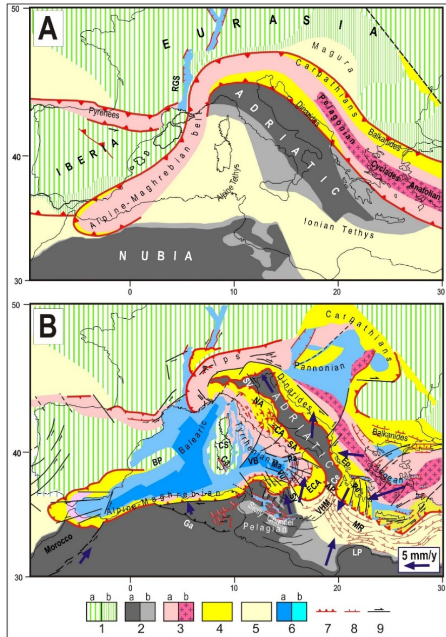
Figure 1. (A) Oligocene paleogeographic configuration. (B) Present tectonic setting. (1a,b) Continental and thinned continental Eurasian domains. (2a,b) Continental and thinned continental African/Adriatic domains (3a,b) Tethyan belt, constituted by ophiolitic and metamorphic units and crystalline massifs (4) Other orogenic belts (5) Oceanic domains (eastern Alpine and Ionian Tethys) (6a,b) Zones affected by intense or moderate crustal thinning (7,8,9) Compressional, tensional and strike-slip features. Ap = Apulian escarpment, BP = Balearic Promontory, CA = Central Apennines, Ca = Campidano graben, Ce = Cephalonia fault system; CS = Corsica-Sardinia block, ECA = External
