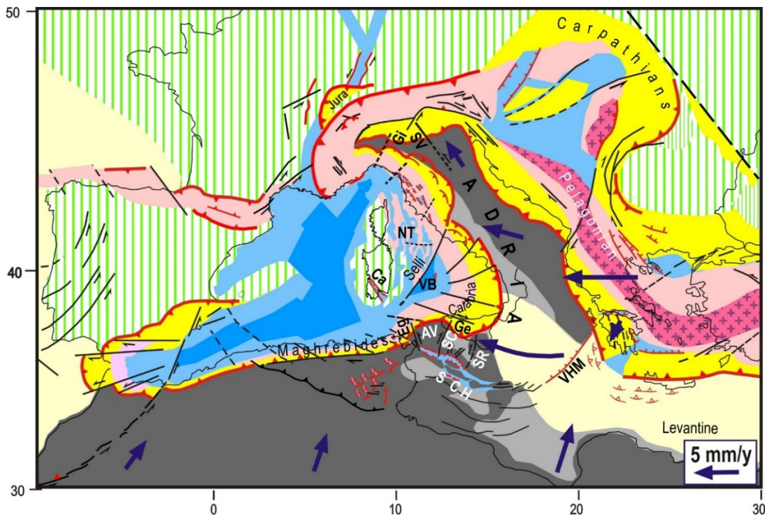
Figure 7. Middle Pliocene tectonic setting. The westward push of the Anatolian–Aegean–Pelagionian system causes the decoupling of the Adria plate from Nubia by the activation of the Victor Hensen–Medina–Sicily Channel fault system. Once decoupled, Adria underwent a clockwise rotation and a minor NW ward motion. The rotation determined major E–W shortening in the Pelagian zone as well as in the Alpine–Maghrebian and Alpine–Apennine zones, whereas the NW displacement of Adria caused the activation of the Schio–Vicenza fault system in the northern Adriatic domain. AV = Adventure wedge, Ca = Campidano graben, CT = Central Tyrrhenian, Eg = Egadi fault, Ge = Gela nappe, Gi = Giudicarie fault system, NT = Northern Tyrrhenian, SCH = Sicily Channel, SC = Sciacca fault, SR = Scicli–Ragusa fault, SV = Schio–Vicenza fault, VB = Vavilov basin, VHM = Victor Hensen–Medina fault. Colours and symbols as in previous evolutionary maps.
