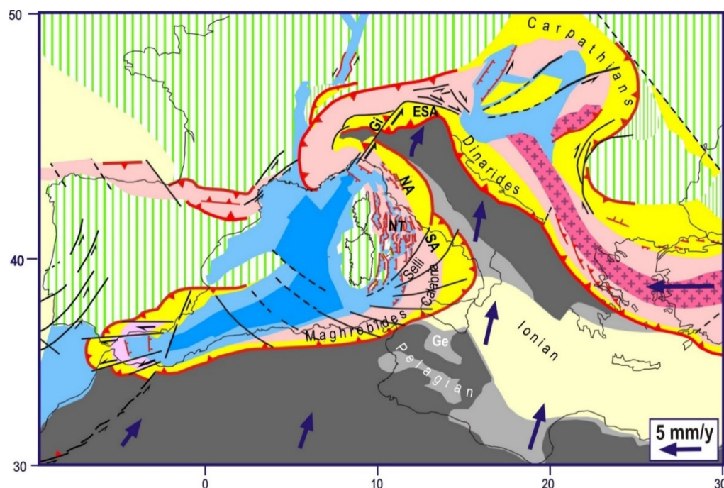
Figure 5. Late Miocene. The reactivation of the Giudicarie fault system (Gi), around the Tortonian, allowed the main Adriatic domain to move roughly NE ward with respect to its northwestern edge. The consequent divergence between the main Adriatic domain and the fixed Corsica-Sardinia block induced crustal extension in the interposed sector of the Alpine–Apennine belt, forming the Northern Tyrrhenian basin (NT). ESA = Eastern Southern Alps; NA = Northern Apennines; SA = Southern Apennines.
