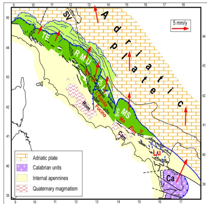
Figure 12. Dragged by the Adriatic plate, the eastern part of the Apennine belt (green) has undergone belt parallel shortening, which has caused the formation of oroclinal arcs and significant uplift. Ben = Benevento, Ca = Calabria, Cam, Rom = Campanian and Roman magmatic provinces, Ir = Irpinia, LA = Lazio-Abruzzi wedge, Lu = Lucania Apennines, Ma = Matese, MS = Molise-Sannio wedge, No-Cf = Norcia-Colfiorito fault system, OA = Olevano-Antrodoto thrust front, RMU = Romagna-Marche-Umbria wedge, SV = Schio-Vicenza fault, SVO = Sangro-Volturno thrust front, TE = Toscana-Emilia wedge. The buried external folds in the Northern Apennines are light green. Red arrows indicate the kinematic pattern, compatible with the Pleistocene deformation pattern and geodetic data (Figure 10). Other symbols as in Figure 1.
