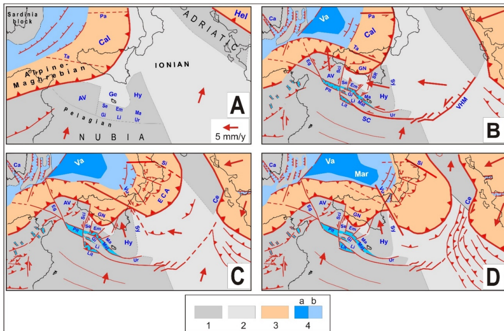
Figure 8. Tentative reconstruction of the tectonic processes that developed in the Hyblean–Adventure domain, in the
