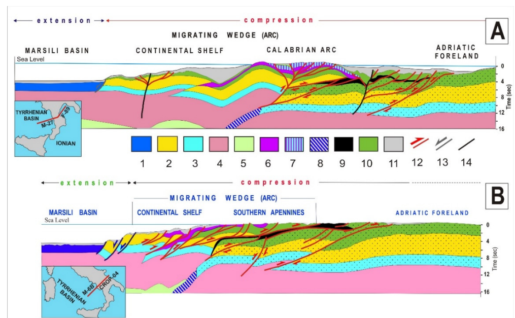
Figure 11. (A) CROP section from the Marsili basin to Adriatic foreland through Northern Calabria (modified after [49]). (1) Oceanic crust; (2) upper continental crust; (3) lower continental crust; (4) Lithospheric mantle; (5) Asthenospheric mantle; (6) remnants of the Alpine Tethys; (7) Kabyló–Calabrides units; (8) Ionian Tethys oceanic slab; (9) Ionides; (10) pre-Pliocene sedimentary cover; (11) Pliocene–Quaternary sediments; (12,13,14) major thrust, normal and strike-slip faults developed during the formation of the Tyrrhenian basin. Dots mark the Adriatic crustal units (from Mantovani et al., 2007, modified). (B) CROP cross section from the Southernmost Tyrrhenian (Marsili basin) to the Adriatic foreland, through the Southern Apennines (modified after [150]).
