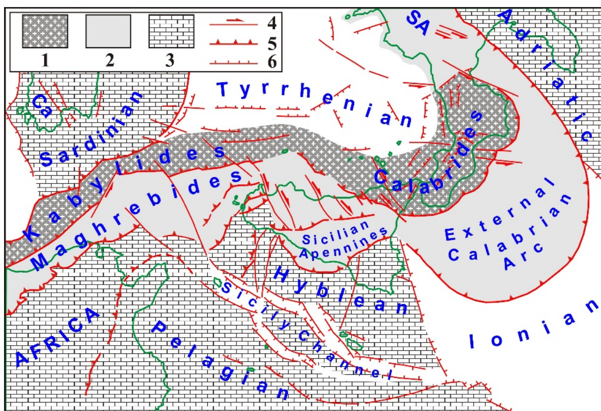
Figure 9. Shape of the Kabyliides–Calabrides (1) and Maghrebides (2) belts (modified after [174,175,182]), (3) foreland domains, (4,5,6) strike-slip, compressional and tensional features. In white the basins. Ca = Campidano graben, SA = Southern Apennines.
