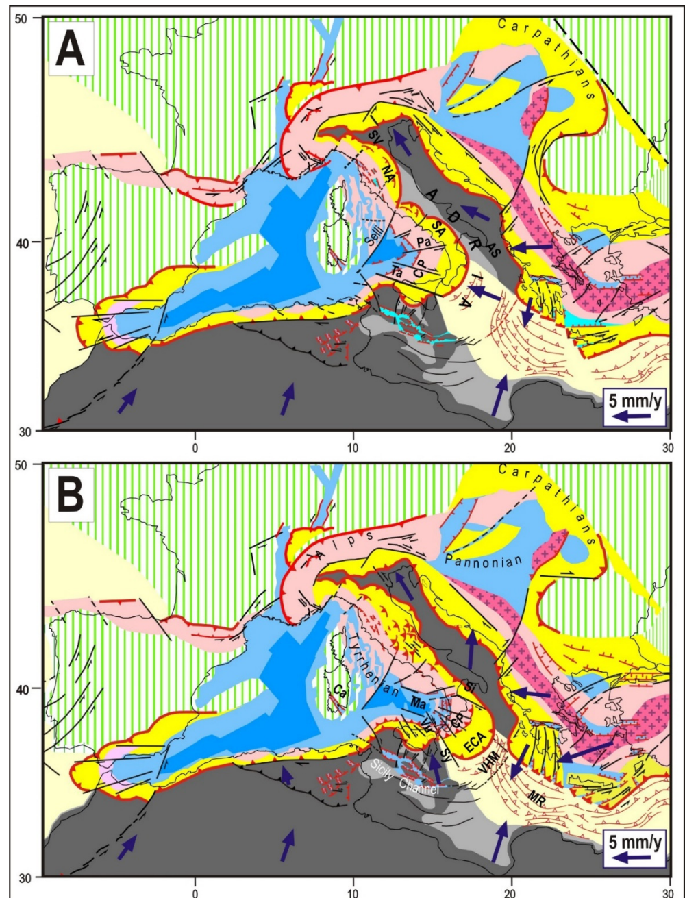
Figure 10. (A) Early Pleistocene tectonic setting. Since the suture of the Southern Apennine consuming boundary the lateral escape of the Alpine–Apennine material has only involved the Calabria–Peloritani (CP) wedge, which has extruded roughly southeastward at the expense of the Ionian oceanic domain. Stressed by E–W compression, the southern Adriatic platform has undergone upward flexure, accelerating the formation of the Apulian Swell (AS). Accretionary activity along the outer Calabrian front has formed the External Calabrian accretionary belt (ECA), whereas crustal extension has developed in the wake of the migrating Arc, forming the Marsili basin (Ma). In this strong compressional context, the CP wedge has undergone fast uplift, bowing and fragmentation. Pa = Palinuro fault, Ta = Taormina fault. (B) Late Pleistocene tectonic setting. The potential gravitational energy accumulated by the southern Adriatic in the previous phase has triggered the northward displacement of Adria. Since the collision of the extruding CP wedge with the Adriatic continental domain, the escape trend of such wedge changed by activating new lateral guides, the Sibari (Si) and Vulcano–Syracuse (Vu–Sy) faults. MR = Mediterranean ridge. Colours and symbols as in Figures 1 and 5.
