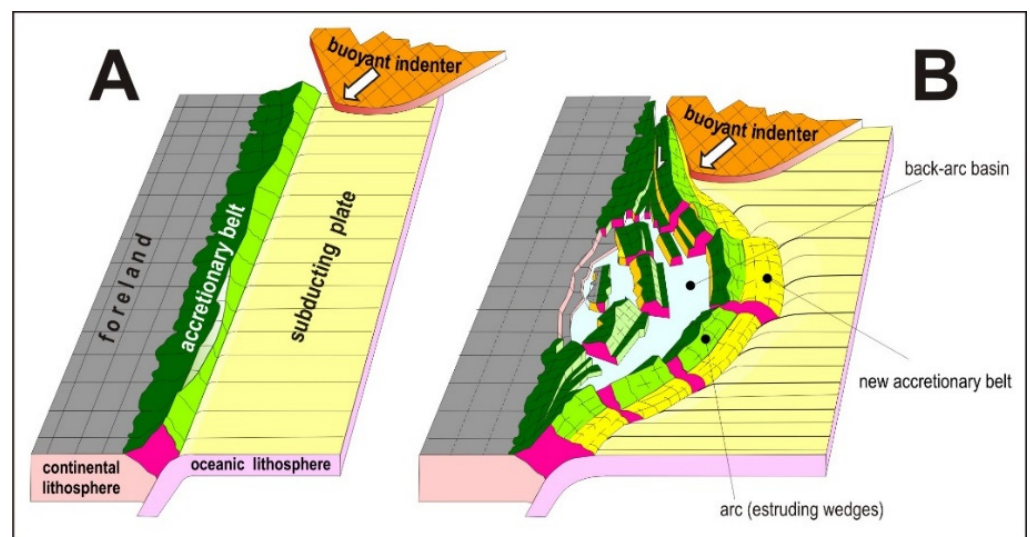
Figure 2. Sketch of the tectonic process that is supposed to generate TABA systems. (A) An orogenic belt, flanked by an oceanic domain, is longitudinally stressed by a continental indenter. (B) The stressed structure detaches from the foreland and undergoes uplift and oroclinal bending, through the lateral escape of crustal wedges. The extruded orogenic material overthrusts the oceanic domain inducing its downward flexure and consequent sinking. The separation of the migrating and bowing Arc from the overriding plate induces crustal extension in the interposed zone (Back Arc basin), whereas accretionary activity occurs at the front of the extruding Arc. See [33,34] for laboratory modeling of that process.
