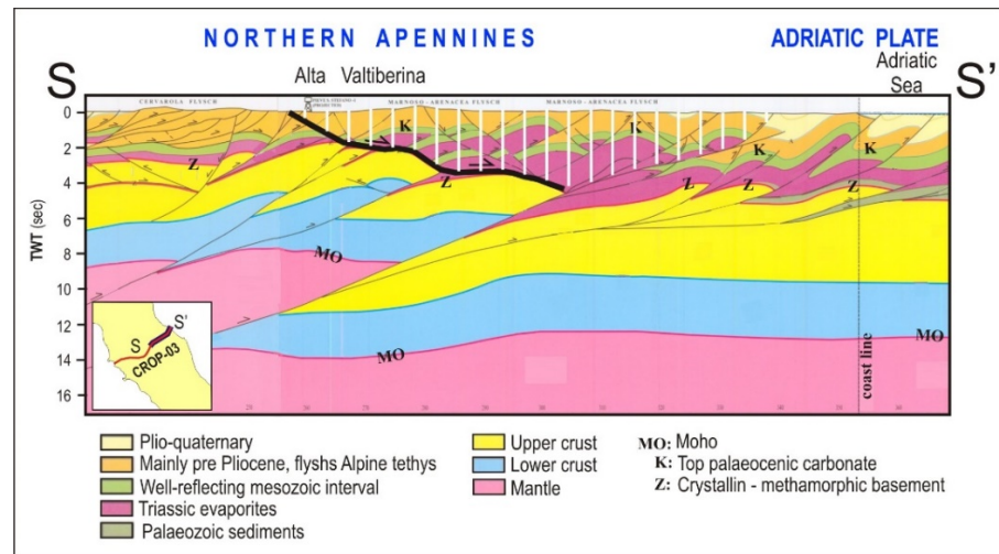
Figure 13. Eastern sector (see inset) of the CROP-03 cross-section ([41,112] modified). The white vertical strips evidence the RMU sedimentary wedge, which is decoupled from its basement by the Valtiberina fault (thick black line). This decoupling has been favored by the presence of Triassic evaporites. The eastward migration of the RMU wedge (driven by belt parallel compression) induces extension in the inner zone and thrusting at the outer front, where the wedge overthrusts the Adriatic domain (see text for explanations).
