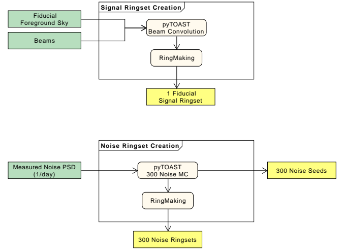
Fig. B.1. Signal and noise ring-set creation pipelines.
