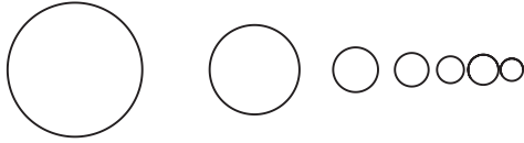
Figure 1: The set \mathcal{T} is a disjoint union of countably many shrinking balls.
