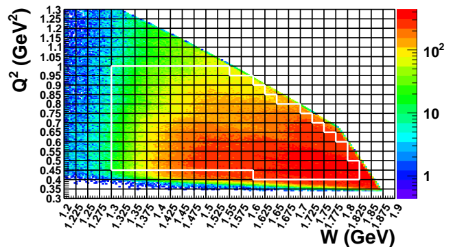
FIG. 13. (colors online) Q^2 versus W distribution populated with selected double-pion events. The cross section was calculated in 2D cells within the white boundaries.
