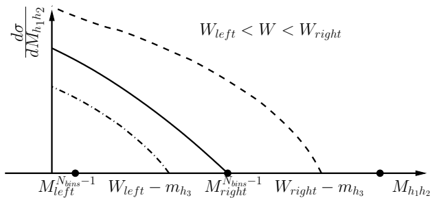
FIG. 14. Schematic representation of the invariant mass distributions ending in M_{\text{upper}} calculated according to Eq. (7) for three choices of W at W_{\text{left}} (dot-dashed), W_{\text{center}} (solid) and W_{\text{right}} (dashed). The black points at M_{\text{left}}^{N_{\text{bins}}-1} and M_{\text{right}}^{N_{\text{bins}}-1} show the left and right boundaries of the next to last bin, respectively.
