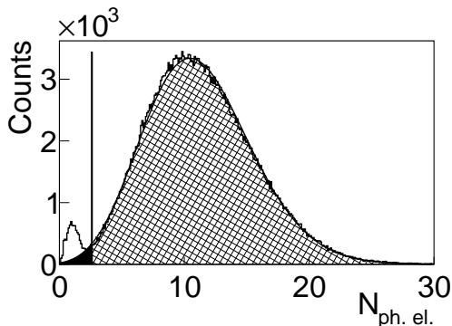
FIG. 5. Number of photoelectrons for the left side PMT in segment 10 of sector 1 of the CC. The black curve shows the fit by the function given by Eq. (2). The vertical line shows the applied cut. Regions that are needed to calculate the correction factor (see Eq. (3)) are shown in hatch and in black.
