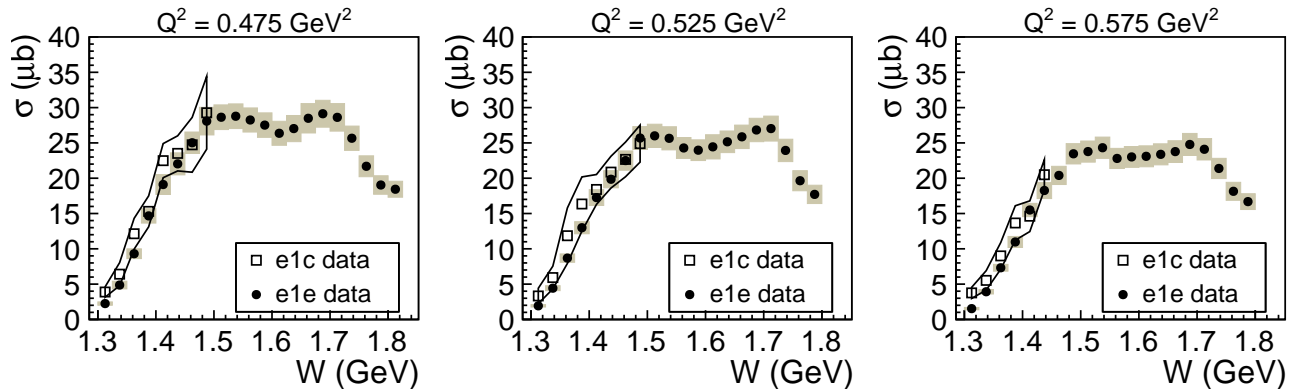
FIG. 21. The W -dependencies of the extracted cross sections (black circles) in comparison with the available data [8] (open squares) for three points in Q^2 . The total cross section uncertainty (which includes both systematic and statistical uncertainties) is shown by the gray shadowed area for the new results (“e1e”), while for the results from Ref. [8] (“e1c”), it is shown by the bands.
