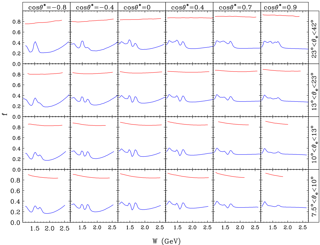
FIG. 7: (color online) Dilution factors as a function of W for the two \pi^+ topologies for Part 4p2o in six \cos(\theta^*) bins (from left to right) and four \theta_e bins (from bottom to top). The upper red curves within each panel correspond to topology ep \rightarrow e\pi^+n and the lower blue curves to topology ep \rightarrow e\pi^+(n) .
