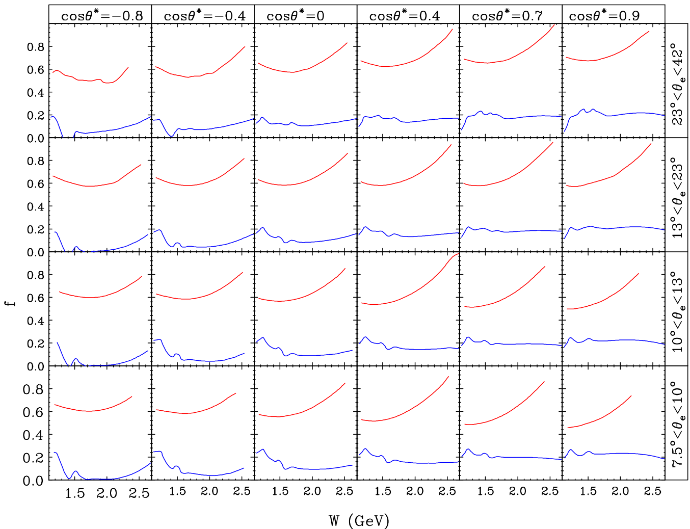
FIG. 8: (color online) Same as Fig. 7, except for the two \pi^- topologies: ed \rightarrow e\pi^-p(p) (upper red curves) and ed \rightarrow e\pi^-(pp) (lower blue curves).
