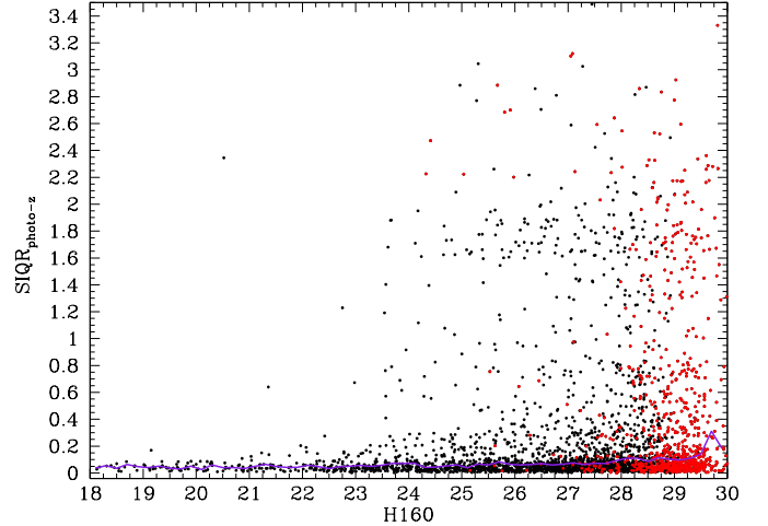
Fig. 1. Semi-interquartile range of the six different photo- z estimates as a function of the H -band magnitude (or upper limit) for H -detected (black circles) and IR-detected (red) sources in the A2744 cluster field. The median SIQR as a function of magnitude is shown as a purple line.
