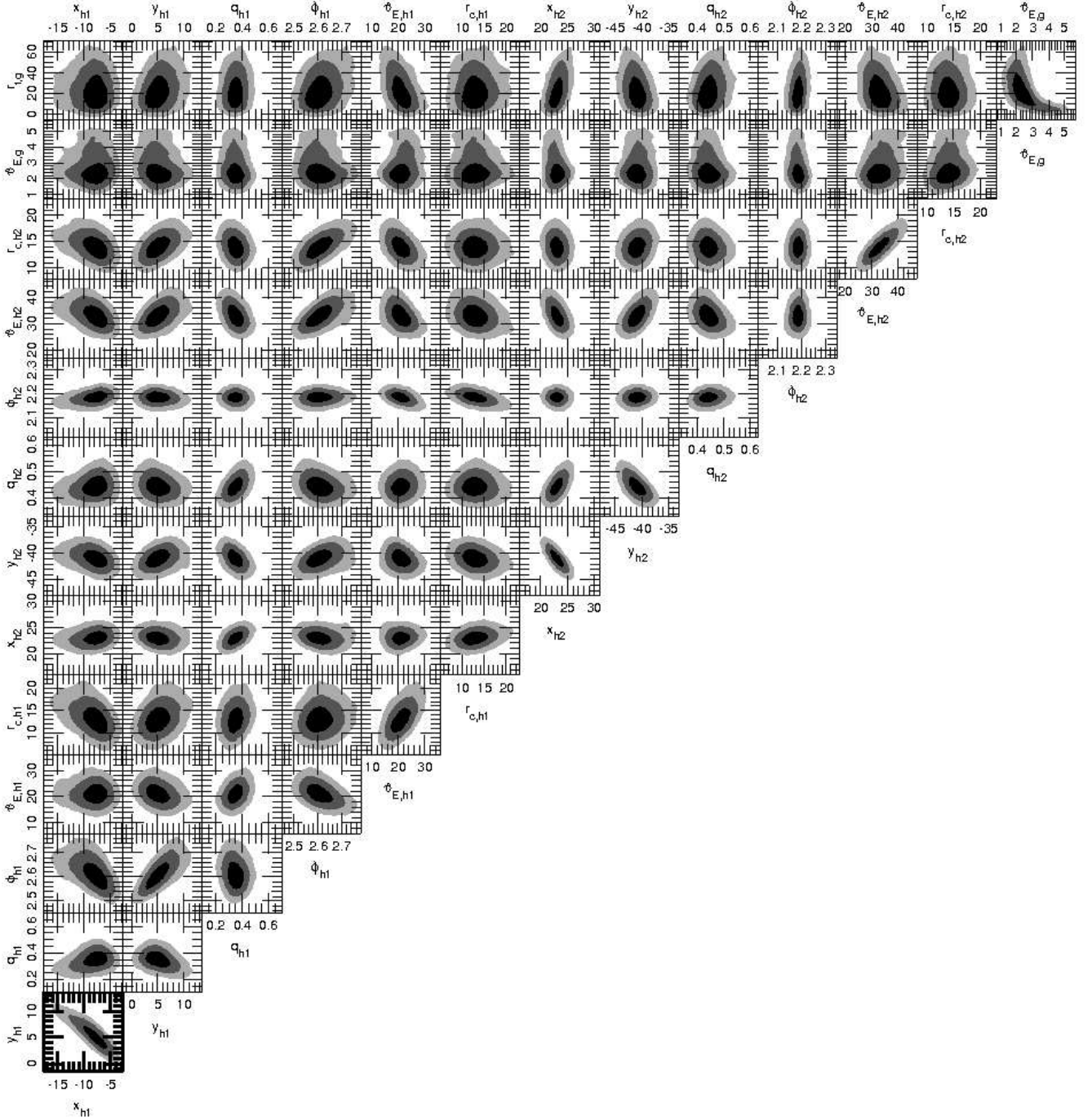
FIG. 13.— Estimates of the uncertainties and correlations of the parameters \eta of the 2PIEMD + 175(+1)dPIE ( M_{\text{T}}L^{-1} \sim L^{0.2} ) model. The gray contour levels on the planes represent the 1\sigma , 2\sigma , and 3\sigma confidence regions and are obtained from a MCMC chain with 2 \times 10^6 samples.
