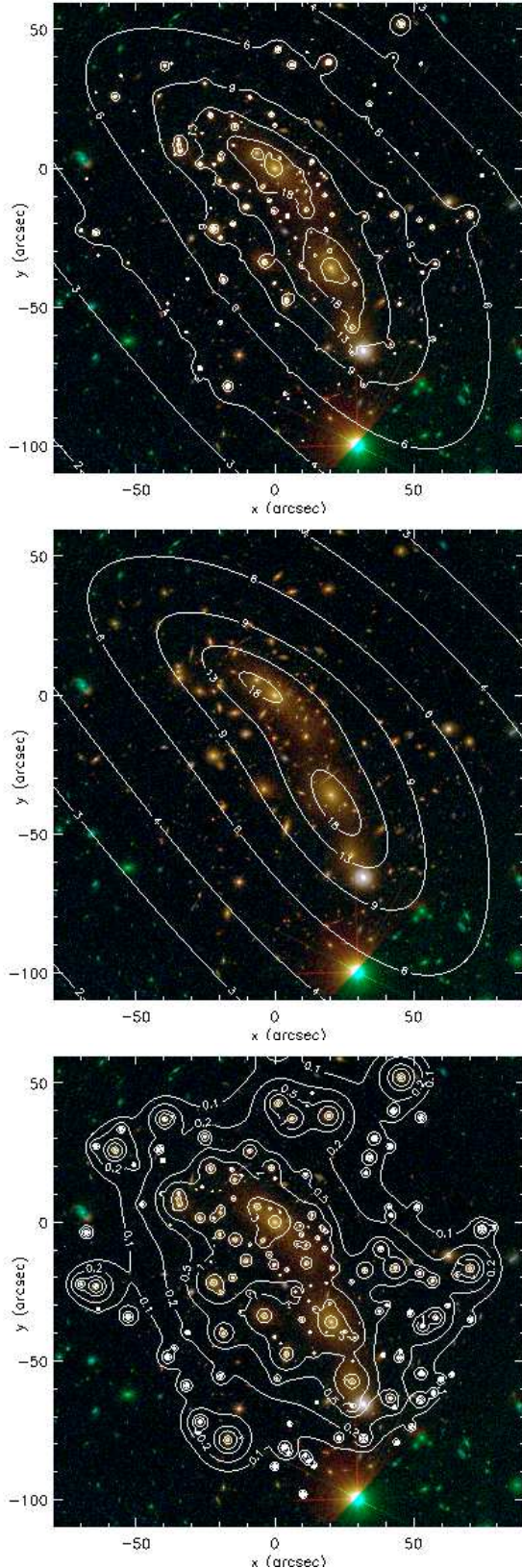
FIG. 10.— Decomposition of the reconstructed total surface mass density, \Sigma_T , ( on the top ) into the surface mass densities of the two extended cluster dark-matter halos, \Sigma_H , ( in the middle ) and many candidate cluster members, \Sigma_G ( on the bottom ). The contour levels on the lens plane are in units of 10^{14} M_{\odot} \text{Mpc}^{-2} .
