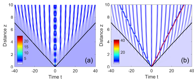
Fig. 6. Numerical solution of NLSE (1), input as in Eq. (2), q_0 = 1 : (a) Gaussian shape with parameters: a = 0.9 , \phi = 0 , t_0 = 1 , \omega = 0 . (b) sech shape with parameters: a = 5 , \phi = \pi/2 , t_0 = 0.4 , \omega = 4 . The IST analysis gives: (a) a single eigenvalue k = 1.468i ( R = 2.54 , \alpha = 0 ), i.e. a KM soliton with period z_p = 0.998 ; (b) a pair k = \pm 0.639 + 1.483i ( R = 3.035 , \alpha = 0.492 ), yielding breather velocities V_s = \pm 3.252 (dashed red line).
