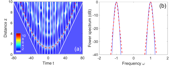
Fig. 3. (a) As in Fig. 2(a), input Gaussian envelope, a = 0.2 , \phi = 0 , t_0 = 16.5 , \omega = 1 . Red dashed curve indicates locus of peaks due to MI amplification: g(\omega)z - t^2/t_0^2 = \text{const.} (see text; here constant used as best-fit parameter). (b) Input power spectrum (log scale, CW suppressed for clarity) for Gaussian (solid blue curve) and sech-shape of Fig. 2 (dashed red curve).
