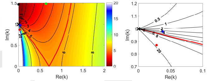
Fig. 4. False color plot and contour lines of breathers velocity V_s from Eq. (4) in the right half complex k plane. Red solid line stands for the asymptotic wedge velocity V_w = 4\sqrt{2} = 5.66 , q_0 = 1 . Right panel shows a zoom around point k = i (cross mark; corresponding to Peregrine rational soliton [2]). Dots indicate the breathers obtained via IST for the other figures: Red dot ( k = 0.029 + 0.870i ), SRBs with V_s > V_w , Fig. 2; Blue dot ( k = 0.0374 + 0.9784i ), SRBs with V_s < V_w , Fig. 5; Black dot ( k = 1.4678i ), KM soliton in Fig. 6(a); Green dot ( k = 0.6386 + 1.483i ), breather pair of Fig. 6(b).
