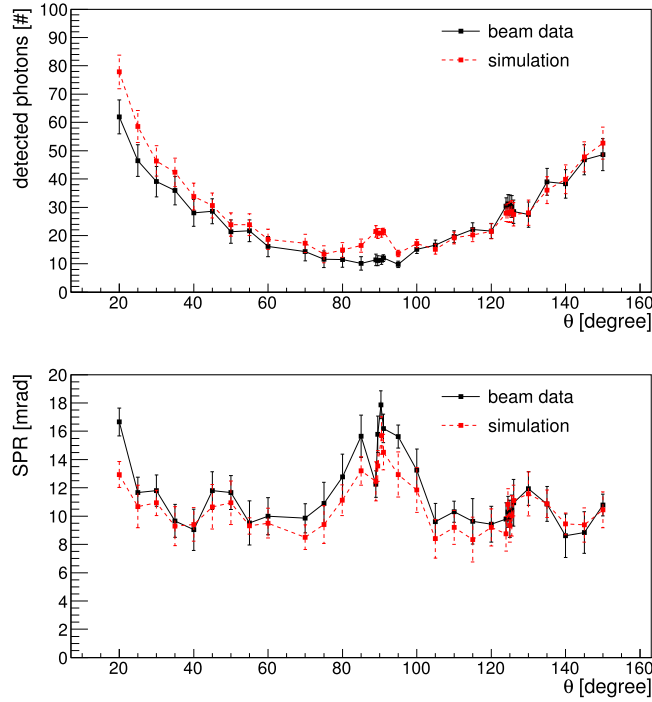
Figure 99. Photon yield (top) and SPR (bottom) as a function of the track polar angle for the narrow bar and the 2-layer spherical lens for tagged protons with 7 GeV/ c momentum in data (black) and Geant simulation (red). The error bars correspond to the RMS of the distribution in each bin.
