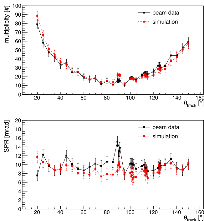
Figure 98. Photon yield (top) and SPR (bottom) as a function of the track polar angle for the narrow bar and the 3-layer spherical lens for tagged protons at 7 GeV/c beam momentum in data (black) and Geant simulation (red). The error bars correspond to the RMS of the distribution in each bin. Reproduced from 2018 JINST 11 C05013. © 2018 IOP Publishing Ltd and Sissa Medialab srl. All rights reserved.
