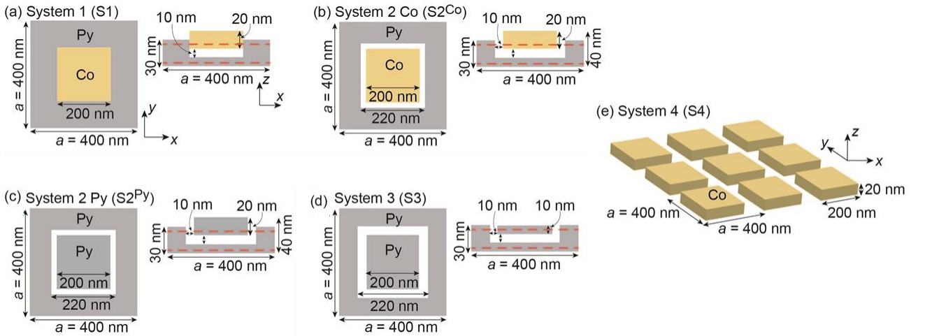
Fig. 1. (a) System 1: Top view of the primitive cell and its perpendicular cross-section in a bi-component MC consisting of Co square dots in square array partially immersed in Py. Non-magnetic spacer (white area) of 10 nm thick separates the bottom of Co dots from Py. (b) System 2-Co: similar to S1 but with full separation of Co dots (200 nm wide) from Py (10 nm of non-magnetic spacer from the bottom and lateral sides of Co). (c) System S2-Py: one component MC with geometry equals to S2 Co but with Py dot. (d) System 3: MC created by square array of square grooves in Py film partially filled with Py dots. Dots are separated from the matrix by 10 nm thick non-magnetic spacer. (e) System 4: square array of square Co dots. Red-dashed lines in the perpendicular cross-sections point at the planes ( z = 5 and 25 nm) used in Figs. 2(a), 2(b), 2(c), 2(d) and 2(e) to visualize the spatial profiles of SW modes.
