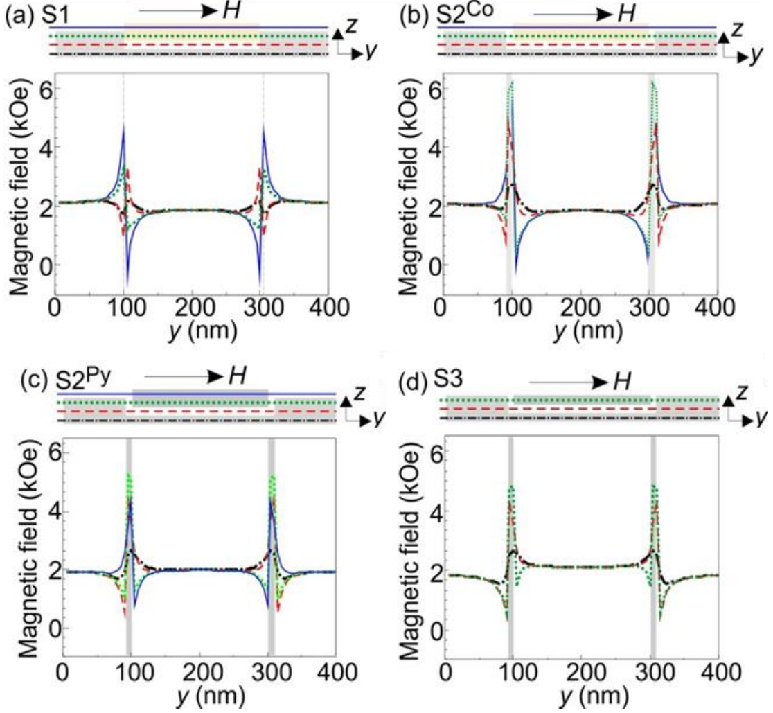
Fig. 5. The y component of the total magnetic field calculated for (a) S1, (b) S2 Co , (c) S2 Py and (d) S3 along the y -axis and averaged along x , for four different values of z : z = 5 \text{ nm} (in full Py film, black dot-dashed line), z = 15 \text{ nm} (crossing Py and spacer below the dots, red dashed line), z = 25 \text{ nm} (crossing Py matrix and middle of dots, green dotted line) and z = 35 \text{ nm} crossing Co dots (only in S1 and S2 Co , blue solid line). The gray vertical rectangles mark the non-magnetic spacer which separate the dot from the matrix. The insets on the top show a sketch of MCs with lines along which the total magnetic field is calculated.
