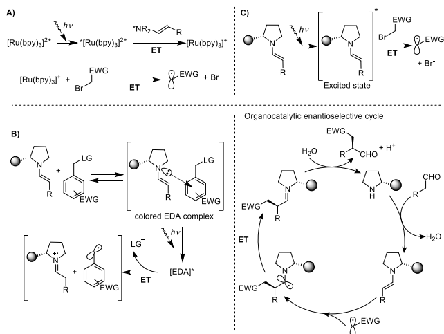
FIGURE 1. Strategies in stereoselective photocatalytic addition of bromo derivatives.
