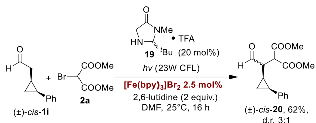
SCHEME 5. Alkylation reaction performed in the presence of a radical-clock.
