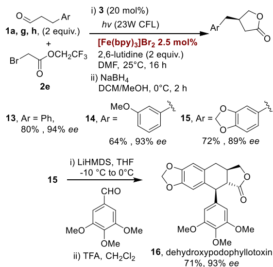
SCHEME 3. Preparation of enantioenriched lactones via alkylation of aldehydes and synthesis of dehydroxypodophyllotoxin.
