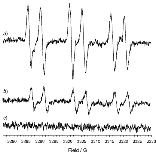
FIGURE 2. EPR spectra of spin adduct 17 generated in ACN in the presence of dimethyl bromomalonate 2a 0.5 M and PBN (0.1 M) as the spin trap at room temperature. Reaction conditions: a) [\text{Fe}(\text{bpy})_3]\text{Br}_2 10 mol%, irradiation with UV-visible light ( \lambda > 320 nm); b) [\text{Fe}(\text{bpy})_3]\text{Br}_2 10 mol%, irradiation with visible light ( \lambda > 420 nm); c) [\text{Fe}(\text{bpy})_3]\text{Br}_2 10 mol% no irradiation. No signals were observed when [\text{Fe}(\text{bpy})_3]\text{Br}_2 was irradiated with UV-visible light in the absence of bromomalonate.
