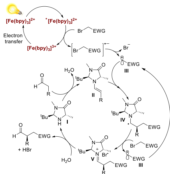
FIGURE 3. Suggested catalytic cycle for the Fe(II) alkylation.
