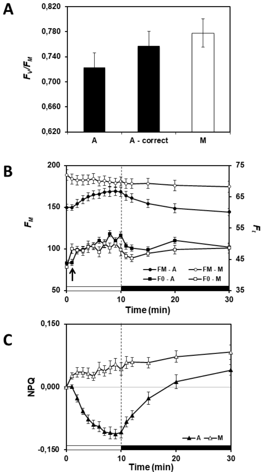
Figure 1. Effects of electron recycling in darkness in Ectlia oleoabundans grown autotrophically or mixotrophically. A. Maximum PSII quantum yield F_V/F_M in autotrophic cells (A), in autotrophic cells after correction for dark chlororespiration (A – correct) and in mixotrophic cells (M). Mean values with SE of N>40 . Student’s t -test indicated a
