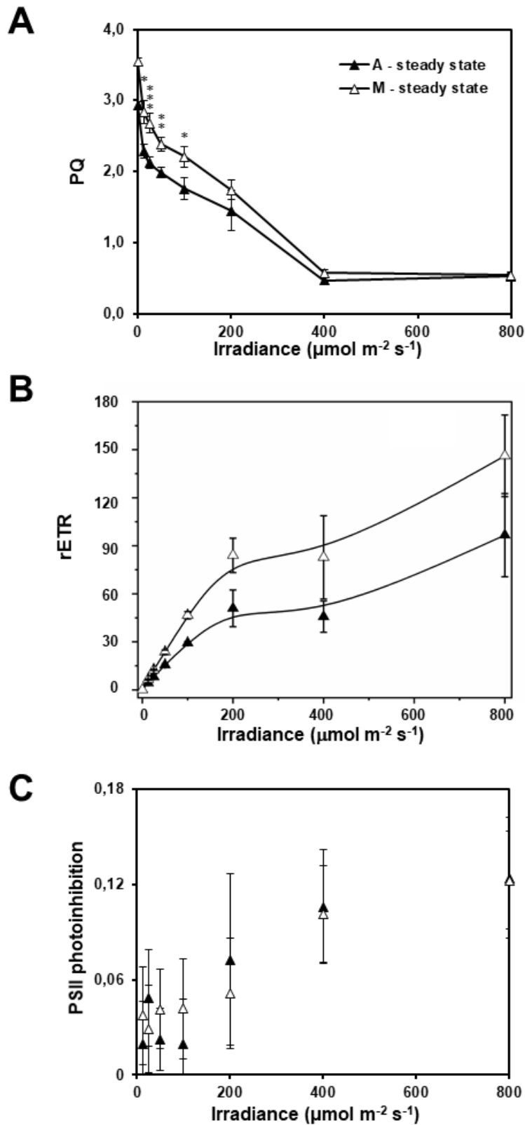
Figure 4. Light curves of fluorescence-derived parameters in Ectlia oleoabundans grown autotrophically (A) or mixotrophically (M). Mean values at the steady state with SE of N=3-9 .
