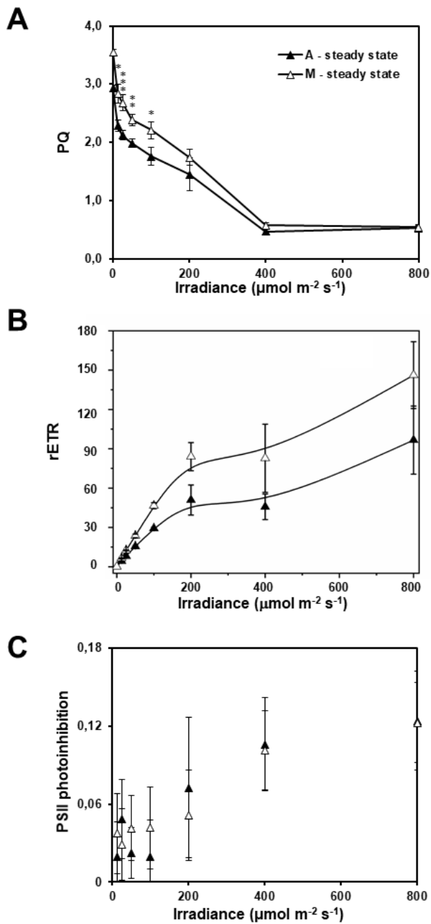
Figure 4. Light curves of fluorescence-derived parameters in Ectlia oleoabundans grown autotrophically (A) or
