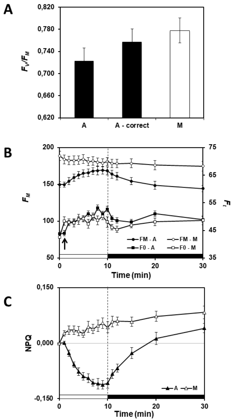
Figure 1. Effects of dark electron recycling in darkness in Ectlia oleoabundans grown autotrophically or mixotrophically.
