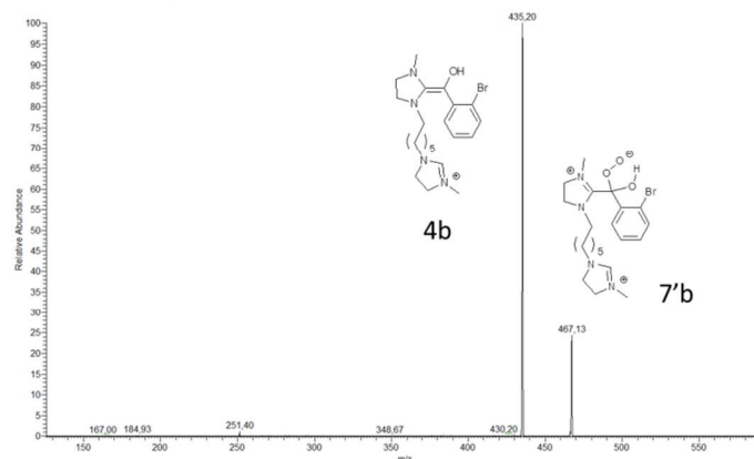
Figure 9. MS/MS spectrum of the peroxy Breslow 7'b at m/z 467 ( 79 Br)
