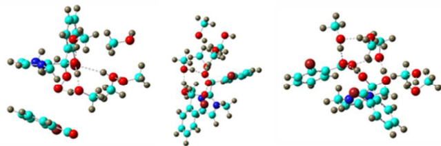
Figure 8. From left to right: Encounter complex between the ortho isomer of 7' and a second o -bromobenzaldehyde molecule 2' . –O–O– bridged intermediate (see Scheme 5, first row right), final complex (see Scheme 5, second row, right).
