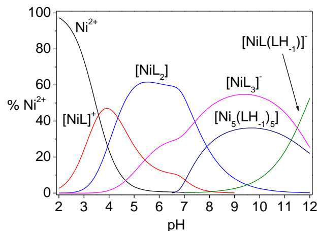
Figure 4. Representative distribution diagram for the system Ni(II) / Picha (HL). Ni:L = 1:2.2, C_{\text{Ni}} = 2.4 \times 10^{-3} \text{ mol L}^{-1} , I = 0.1 \text{ mol L}^{-1} (KCl), T = 298.16 \text{ K} .
