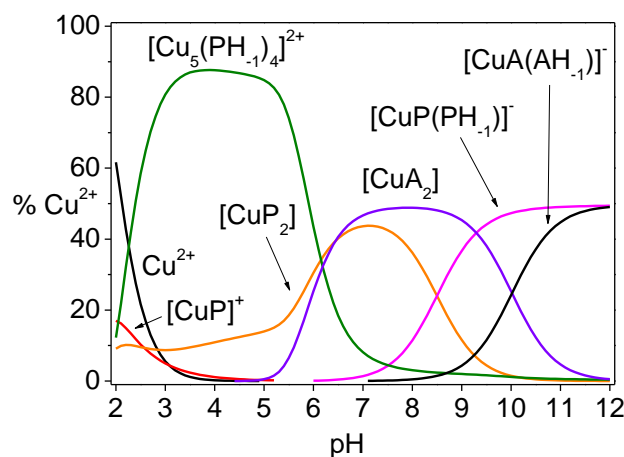
Fig. 9 Representative competition diagram for the system Cu(II) / Picha (HP) / Alaha (HA). Cu:P:A = 1:1:1, C_{\text{Cu}} = 2.8 \cdot 10^{-3} \text{ mol L}^{-1} . The \log \beta values of the species are reported in Table 1.
