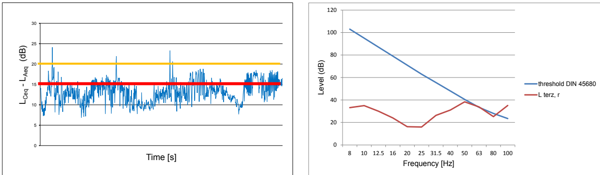
18 Figure 6 – (a) first step (time range 23.45 – 00.15) and (b) 1/3 octave band assessment
