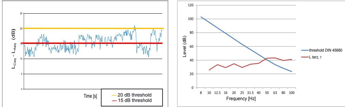
Figure 8 – (a) first step (time range 01.38 – 02.15) and (b) 1/3 octave band assessment
