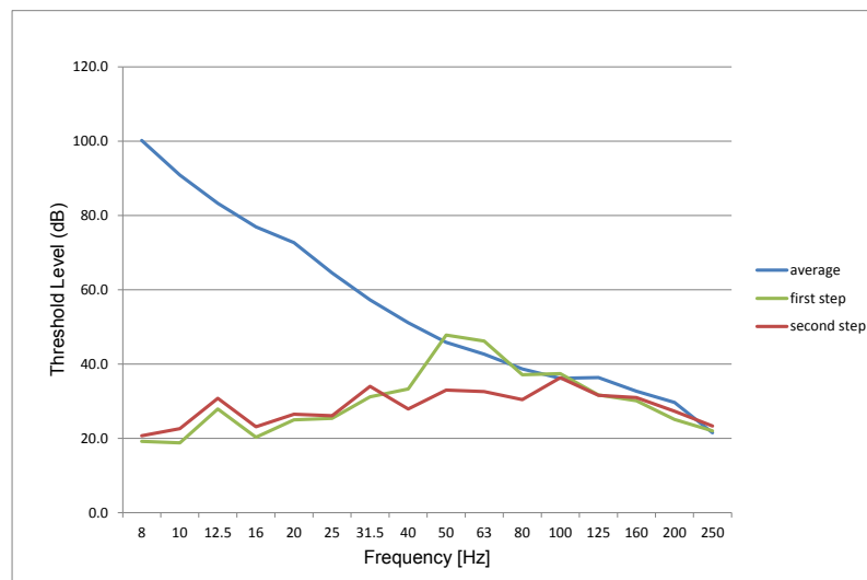
588 589 Figure 15 – the new method applied in real-life circumstances (see paragraph 3.4) 590
