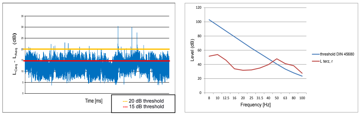
Figure 12 – (a) first step (time range: 20.30 – 22.00) and (b) 1/3 octave band assessment
