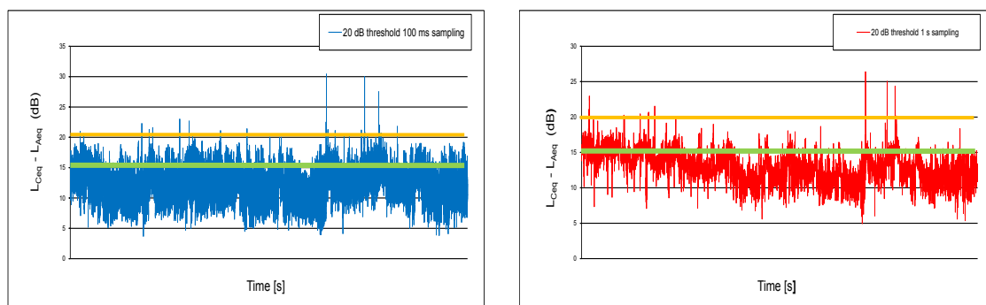
Figure 1 – Operability threshold (20 dB yellow line, 15 dB green line) according to DIN 45680 (time range 22.15 – 23.37).
