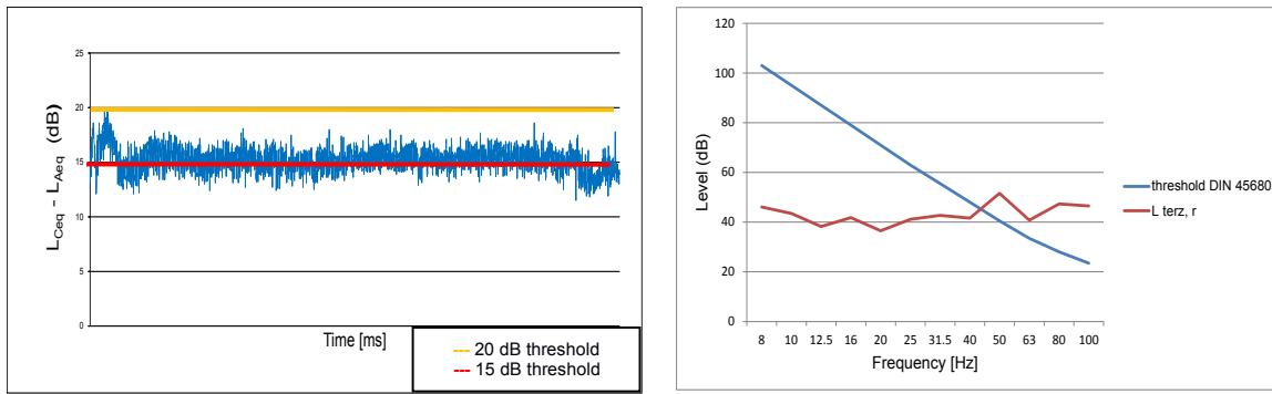
Figure 10 – (a) first step (time range 17.30 – 18.30) and (b) 1/3 octave band assessment
