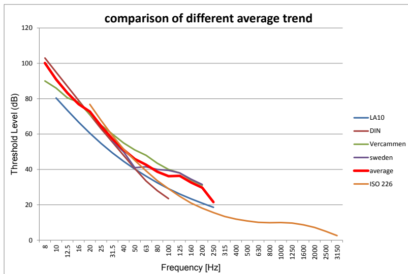
Figure 14 – literature standard and average of the averages trends
