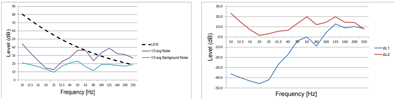
31 Figure 7 – Polish method trends, (a) noise and threshold; (b) defined parameters
