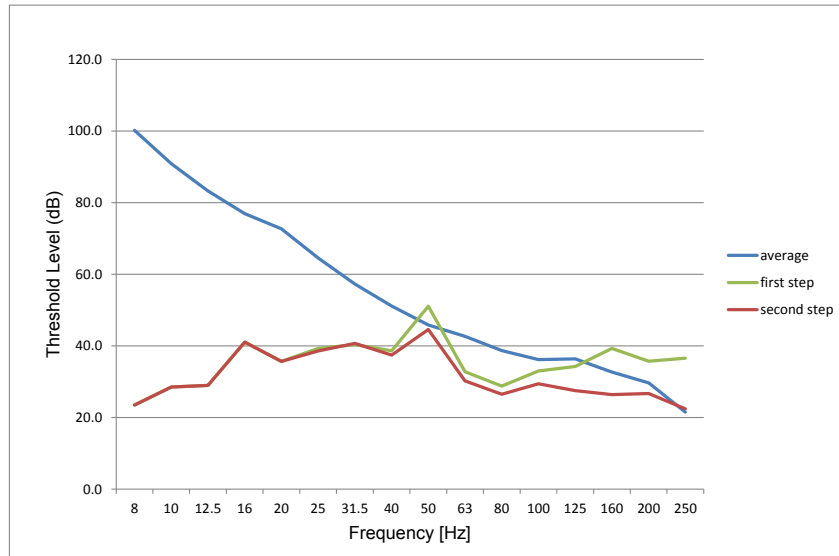
Figure 16 -- the new method applied in real-life circumstances (see paragraph 3.5)
