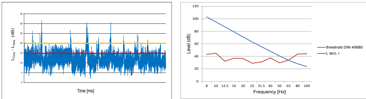
Figure 4 – (a) first step (time range 22.06 – 23.01) and (b) 1/3 octave band assessment
