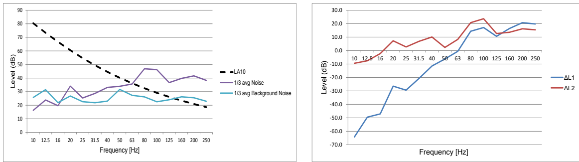
Figure 9 – Polish method trends, (a) noise and threshold; (b) defined parameters
