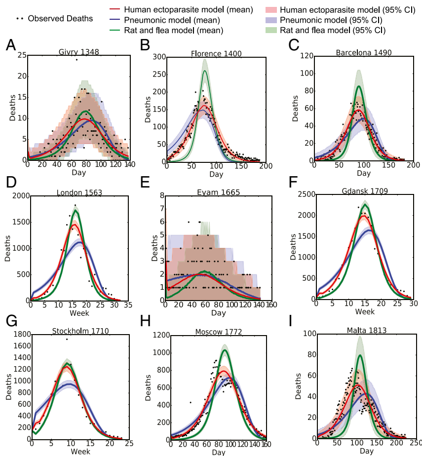
Fig. 1. Fit of three models of plague transmission to mortality during Second Pandemic outbreaks. The observed human mortality data (black dots) and the fit (mean and 95% credible interval) of three models for plague transmission [human ectoparasite (red), pneumonic (blue), and rat–flea (green)] for nine plague outbreaks: (A) Givry, France (1348), (B) Florence, Italy (1400), (C) Barcelona, Spain (1490), (D) London, England (1563), (E) Eyam, England (1665), (F) Gdansk, Poland (1709), (G) Stockholm, Sweden (1710), (H) Moscow, Russia (1772), and (I) Island of Malta, Malta (1813).
