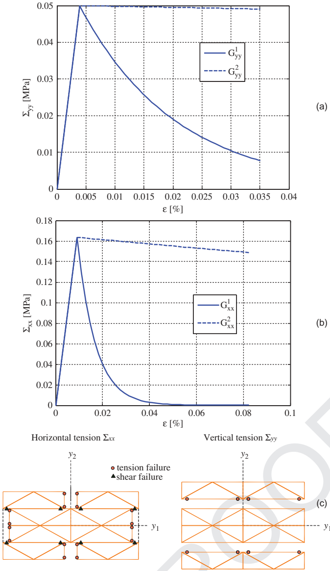
FIG. 19. a) and b) Uniaxial response of the homogenization model along vertical a) and horizontal b) tension for two values of fracture energy, c) representative element of volume (REV) deformed shape at collapse with indication of interface damage in horizontal tension (left) and vertical tension (right).
