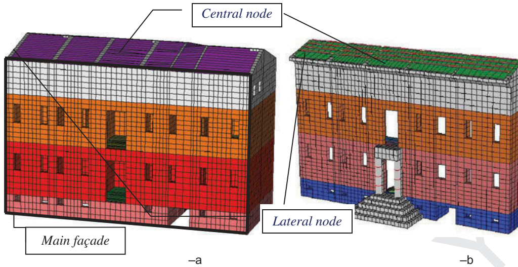
FIG. 12. Finite element model: a) discretization of the entire building (8,958 solid elements, 851 plate and shell elements, 19,526 nodes); b) discretization of the facade (2,776 solid elements, 590 plate and shell elements, 573 beam elements, 6,210 nodes). Different colors of the elements indicate different floors.
