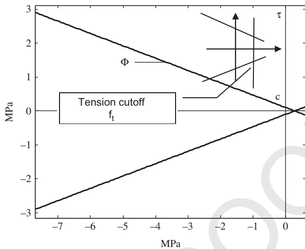
FIG. 18. Linearized failure surfaces adopted for mortar in the softening model with rigid elements and interfaces.
