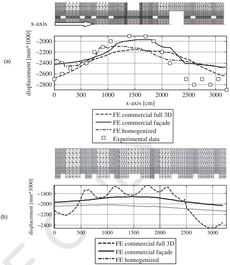
FIG. 25. Comparison among different finite element (FE) models and monitored displacements. Top: base of the building. Bottom: roof level.
