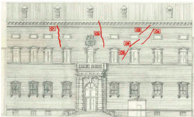
FIG. 7. Main facade with the surveyed crack pattern.
