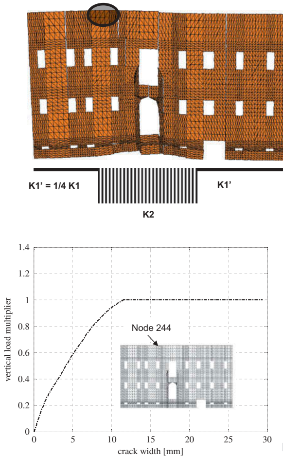
FIG. 23. Prosecution of numerical simulations decreasing linearly K_1 to 25% of its initial value: a) deformed shape of the facade at the end of the non-linear simulations. (6880 triangular elements), b) crack width versus vertical load multiplier.
