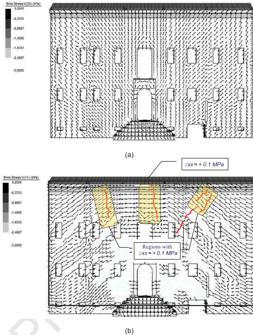
FIG. 15. Direction of the principal stresses, partial model: a) minimum principal stress directions, b) maximum principal stress directions with comparison of position of actual cracks and those provided by the numerical model.
