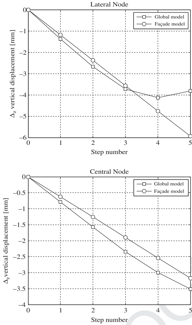
FIG. 16. Comparison between vertical displacements provided by the elastic-plastic global and partial models. Top: lateral node, last floor level. Bottom: central node, last floor level.
