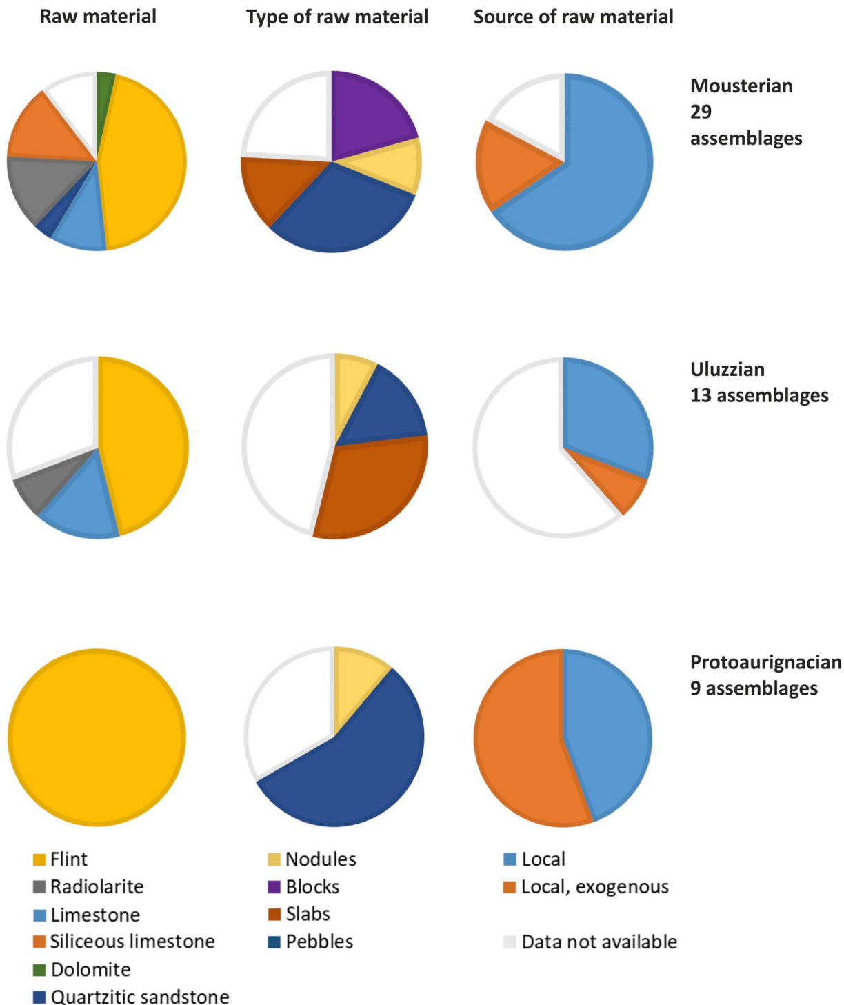
Fig. 5. Mousterian, Uluzzian and Protoaurignacian key sites according to the lithology, type and source of raw material. Raw data and reference in Table 1.
