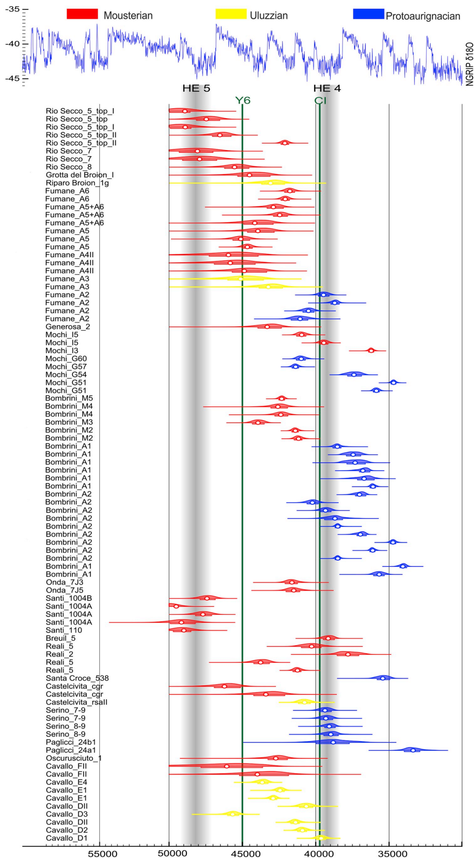
Fig. 3. 14C dates of Protoaurignacian, Uluzzian and Mousterian sites. OxCal v4.3.2 (Bronk Ramsey, 2017); r5Int Cal 13; 68.2% atmospheric curve (Reimer et al., 2013). Raw dates and bibliographic references in Table 1 SM.
