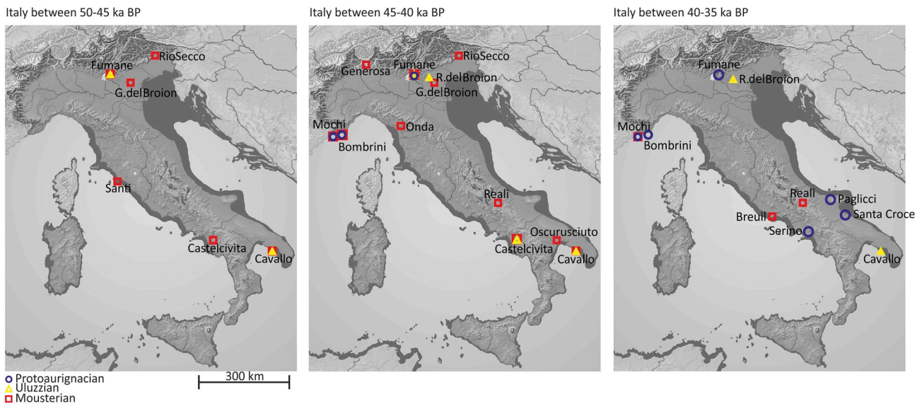
Fig. 4. Location of the Italian Mousterian, Uluzzian and Protoaurignacian key sites with MIS3 human occupations according to their 14C dates. Raw dates and bibliographic references in Table 1 SM.
