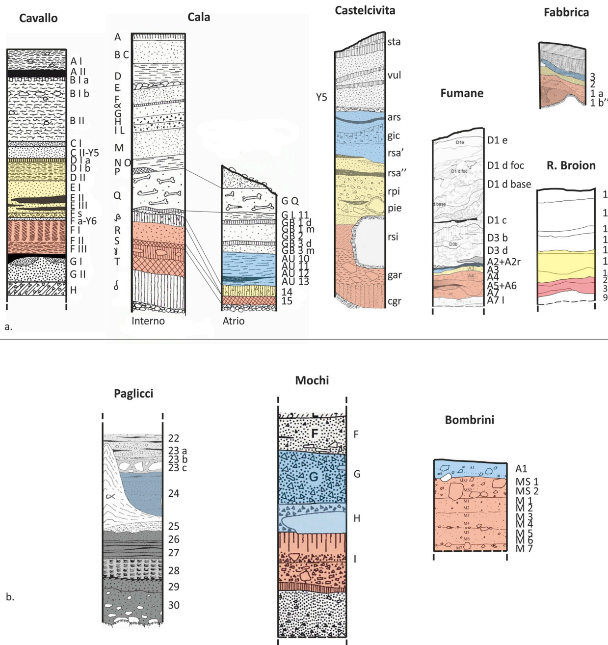
Fig. 2. Key stratigraphic sequences. a. Moustesian, Uluzzian and Protoaurignacian sequences (Cavallo modified from Palma di Cesnola, 1964; Cala, Castelcivita modified from Gambassini, 1982; Fumane modified from Tagliacozzo et al., 2013; R. Broion modified from Peresani et al., 2019; Fabbrica modified from Villa et al., 2018); b. Moustesian-Protoaurignacian sequences (Paglicci modified from Palma di Cesnola, 1992; Mochi modified from de Lumley, 1969; Bombrini modified from Riel-Salvatore and Negrino, 2010).
