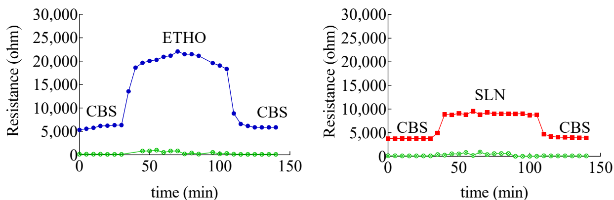
Figure 6. Variation of skin membrane resistance upon addition of SLN (red), ETHO (blue). The green profile refers to receiving phase solution. The skin membrane was assembled in a Franz cell equipped with four electrodes, as shown in Figure S1.
