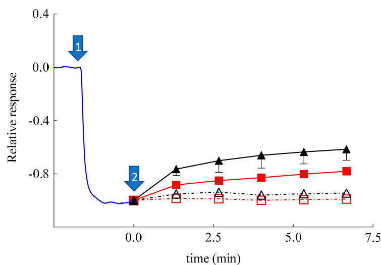
Figure 8. Relative, average amperometric current response on addition of H 2 O 2 (0.1 mM) (marked by arrow #1; n = 13 ) recorded by using a catalase/peroxidase enzyme-modified oxygen electrode. Arrow #2 marks the addition of Sol-CA (CA 0.03 mM, closed triangles, n = 3 ), SLN-CA (0.03 mM CA, closed squares, n = 3 ), SLN (open squares, n = 3 ), and EtOH: CBS (30/70 v/v , open triangles, n = 3 ).
