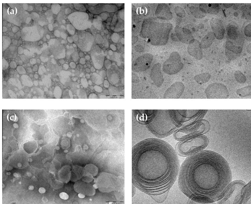
Figure 1. Caffeic acid containing solid lipid nanoparticles (SLN-CA) (a,b) and caffeic acid containing ethosomes (ETHO-CA) (c,d) obtained by transmission (a,c) or cryogenic transmission (b,d) electron microscopy. The bar corresponds to 150 nm in panels (a–c) and 50 nm in panel (d).
