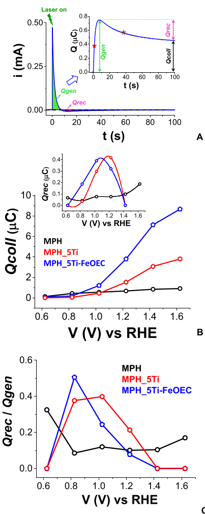
Figure 10. (A) Typical TPC decay and corresponding photo-generated charge trace (inset) obtained after its integration over time, illustrating the contributions due to Q_{\text{gen}} , Q_{\text{rec}} , and Q_{\text{coll}} . The values indicated with the red and purple stars correspond to the times at half-amplitude \tau_1 and \tau_2 ( vide infra ). In this specific case, the i-t trace corresponds to a MPH 5 Ti photoanode held at 1.02 V bias. (B and C) Applied bias dependence of Q_{\text{coll}} (B) and Q_{\text{rec}} (B, inset) and of Q_{\text{rec}}/Q_{\text{gen}} (C) for MPH, MPH 5 Ti, and MPH 5 Ti-FeOEC.
