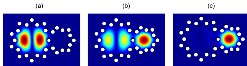
Fig. 6. Field intensities calculated at Z = 0 , L_c/2 , and L_c when the E_x polarization of the LP_{11a} mode of the large fiber core is launched.
