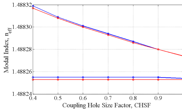
Fig. 4. Values of supermode effective indices n_{eff} as a function of the Coupling Hole Size Factor (CHSF) for Structure Scale Factor , SSF = 0.85. Blue and red lines refer to E_x and E_y , respectively.
