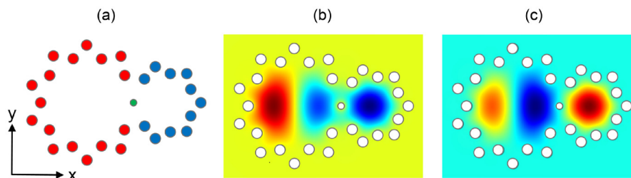
Fig. 2. (a) Geometry of the dual-core coupler. (b)-(c) Distribution of the E_x/E_y field components of the two supermodes with PMCS/PECS along the horizontal x axis.
