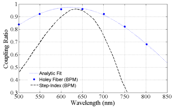
Fig. 8. Wavelength-dependence of coupling from the LP_{01} mode excited in the small fiber core to the LP_{11a} mode of the large core of the holey fiber coupler. Also shown is the spectral response of an analogous step-index fiber mode coupler. Results obtained using numerical BPM simulations.
