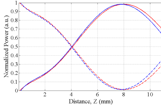
Fig. 7. Plot of the power in each fiber core for different excitations of the large core. Settings are identical to those of Fig. 5 except that CHSF = 0.4 . As before, the blue and red curves refer to the power evolutions in the two cores when the two polarizations of the LP_{11a} mode are launched. Dashed lines refer to power evaluated in the larger fiber core, whereas solid lines refer to power in the smaller core.
