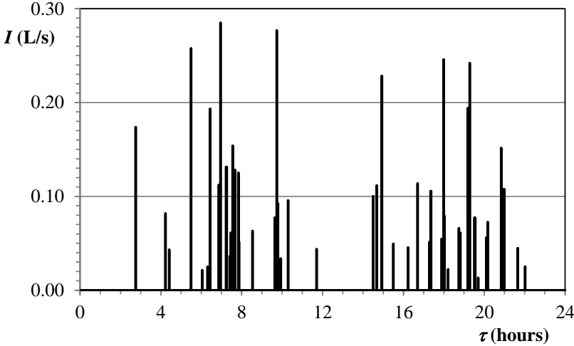
346 Figure 1. Model C - single realization of the simulated total demand for a typical day at the scale of 1 sec.
