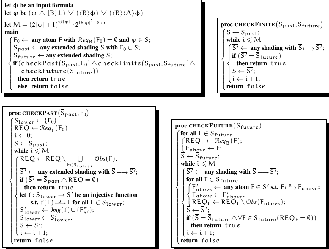
Figure 4: the procedure for checking the satisfiability of \phi over the integers.
