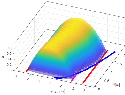
Fig. 4. Paraboloid-shaped CBFs defined on the set of ellipses that approximate the safe set.
