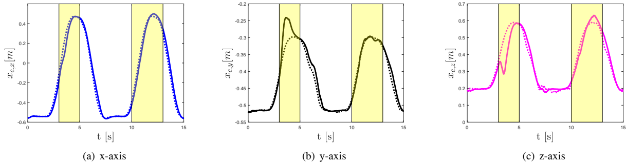
Fig. 6. Cartesian robot positions: nominal trajectory (dashed line) and ZCBF constrained trajectory (solid line).
