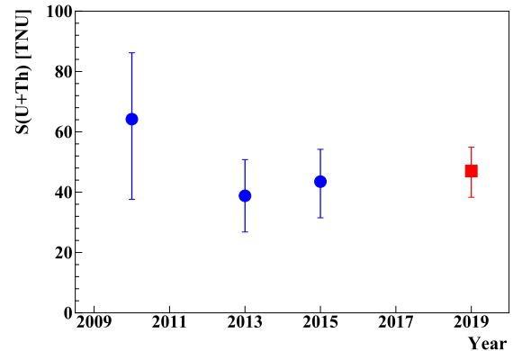
FIG. 51. Comparison of the geoneutrino signal S_{\text{geo}}(\text{U}+\text{Th}) at LNGS as measured by Borexino. Blue circles indicate the results from 2010 [16], 2013 [17], and 2015 [18], while the red square demonstrates the current analysis.
