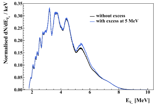
FIG. 19. Comparison of the spectral shapes “with and without the 5 MeV excess” for reactor antineutrinos expected to be detected in Borexino via the IBD interaction for the period December 2007 to April 2019. The spectra are normalized to one. We note that the expected number of events predicted by the spectrum “with 5 MeV excess” diminishes by about 6% with respect to the one “without 5 MeV excess”, consistently with the normalization factor R = 0.946 found in [101].
