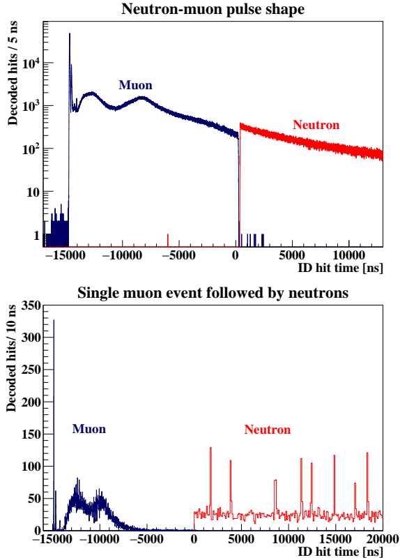
FIG. 5. Top: Event structure of TTI & BTB4 muons (blue) and the start of the follow-up 1.6 ms-long TTI28 neutron gates (red) collected in a typical 6 hour run. Due to the large amount of light for muon events, the detected hits at the end of TTI & BTB4 events are pre-scaled, causing the step between the two trigger types. Bottom: example of a TTI & BTB4 muon (blue) followed by a TTI28 event (red) with high neutron multiplicity.
