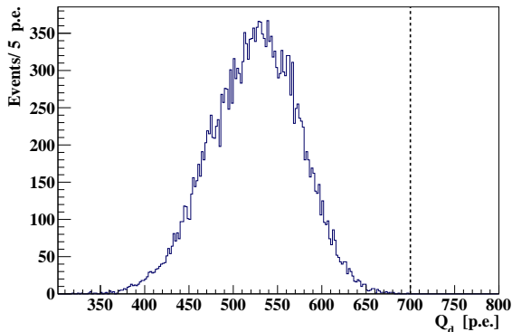
FIG. 42. Charge spectrum of MC generated ^{212}\text{Po} \alpha peak. The vertical line at 700 p.e. shows the optimized Q_d^{\text{min}} for IBD selection.
