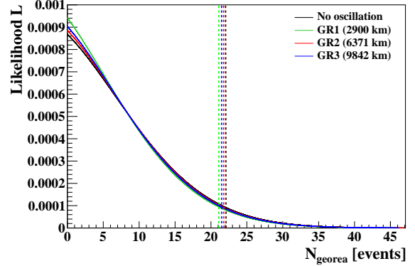
FIG. 57. Likelihood profiles for the number of georeactor events N_{georea} obtained in the spectral fits with the constrained number of reactor antineutrino events. The four profiles represent the fits that differ in the shape of the PDF used for the georeactor contribution (Fig. 34), corresponding to different source positions in the deep Earth (GR1, GR2, GR3, Fig. 21(a)) and to a no-oscillation hypothesis. The vertical dashed lines indicate the upper limit at 95% C.L. for N_{georea} as obtained in each of the four fits. In setting the upper limit on the power of the georeactor, that depends on the assumed location of the georeactor, we use conservatively the highest limit on N_{georea} equal to 21.7 events.
