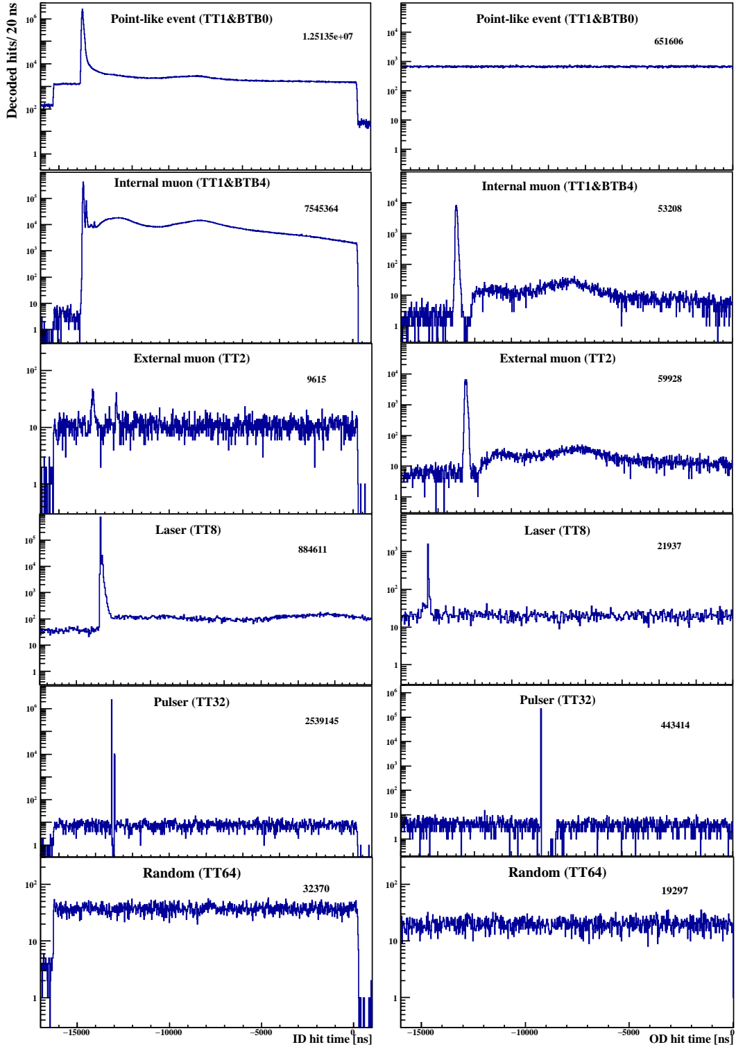
FIG. 3. Event structure, i.e. hit time distribution in a 16\mu\text{s} DAQ gate with respect to the trigger time, for different event types as acquired during a typical 6 hour run by the ID (left column) and the OD (right column). The hit times are negative, since the hits are detected before the trigger decision is made. Different rows represent, from top to bottom, the different trigger types: point-like events in the ID ( TT1 & BTB0 ); internal muons ( TT1 & BTB4 ); external muons ( TT2 ); and the three types of calibration triggers: laser ( TT8 ), pulser ( TT32 ), and random ( TT64 ). The total number of decoded hits detected for each trigger type is shown on the top right corner of the respective pads.
