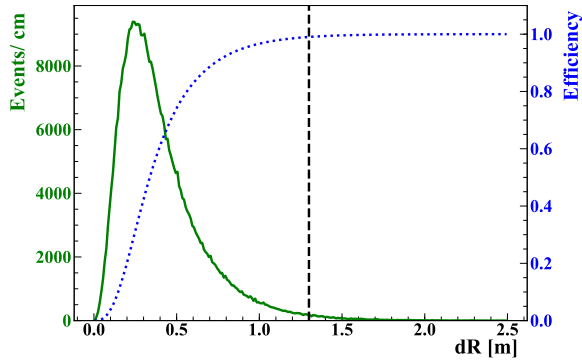
FIG. 27. Distribution of the prompt-delayed reconstructed distance dR (solid green line) shown for the geoneutrino MC sample and the corresponding efficiency (blue dotted line). The vertical dashed line shows the optimized dR cut at 1.3 m.
