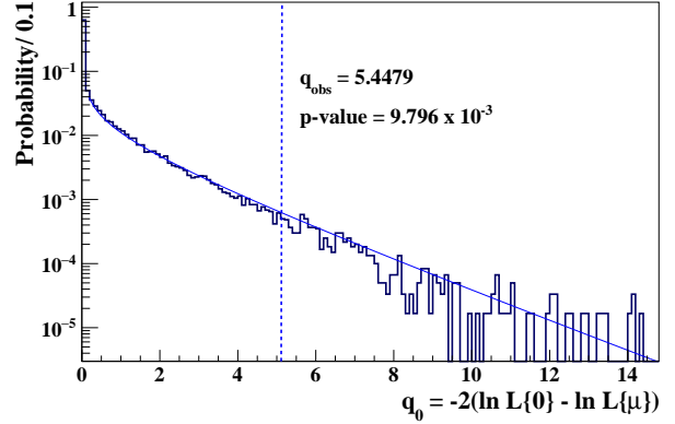
FIG. 53. The q_0 distribution for 1.2 million pseudo-experiments without any generated mantle signal fitted with f(q|0) (Eq. 39). The vertical dashed line represents q_{\text{obs}} obtained from the data. The indicated p -value, calculated following Eq. 41 by setting q_{\text{med}} = q_{\text{obs}} , represents the statistical significance of the Borexino observation of the mantle signal.
