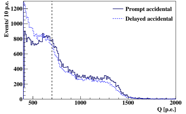
FIG. 37. The charge energy spectrum of the prompts (solid) of accidental coincidences selected in dt = [2 \text{ s}, 20 \text{ s}] time window with the optimized IBD selection cuts. For the delayed signals (dotted), we show the spectrum with Q_d^{\text{min}} lowered to 400 p.e. and scaled to the number of prompts in the solid-line spectrum. The dashed vertical line shows the chosen Q_d^{\text{min}} charge threshold of 700 p.e.
