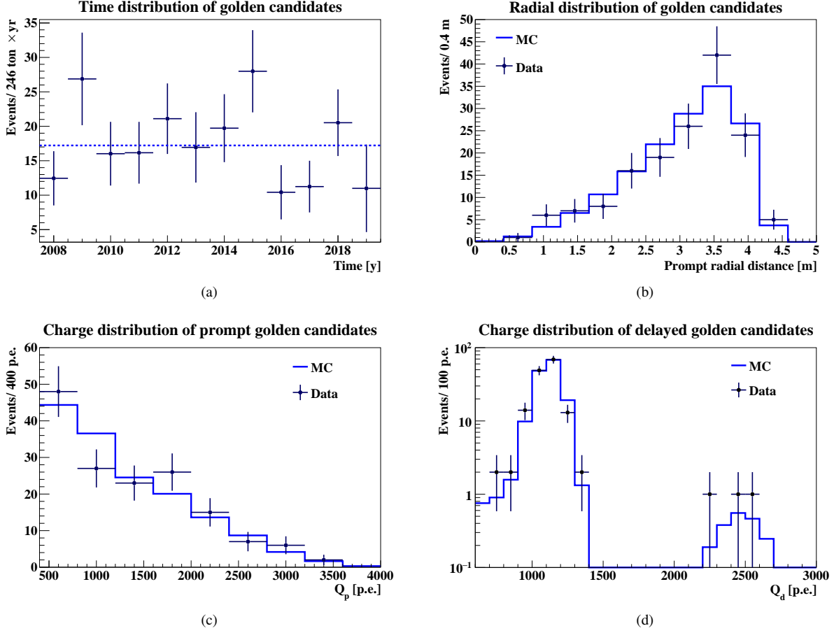
FIG. 46. Distributions for 154 golden IBD candidates (black data points). MC distributions (blue solid lines) are all normalized to the same number of events. (a) Observed IBD-rate (per average FV and one year) as a function of time in one year bins (December 2007 is included in 2008 data point). The dashed line represents the average IBD rate in the entire data set. (b) Radial distribution of the prompt signals compared to the MC expectation. (c) Charge distribution of the prompts compared to the MC, assuming the geoneutrino and reactor antineutrino events follow the expectations as in Table XIV. (d) Charge distribution of the delayed compared to MC. The two peaks due to the captures on proton and on ^{12}\text{C} are clearly visible.
