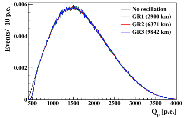
FIG. 34. MC-based PDFs of prompts for a georeactor (Sec. 5.5) after optimized IBD selection cuts, normalized to one. We show both the case of non-oscillated spectrum, as well as the oscillated spectra for the georeactor placed in three positions at different depths: GR1 ( d = 2900 km), GR2 ( d = 6371 km), and GR3 ( d = 9842 km), defined in Fig. 21(a).
