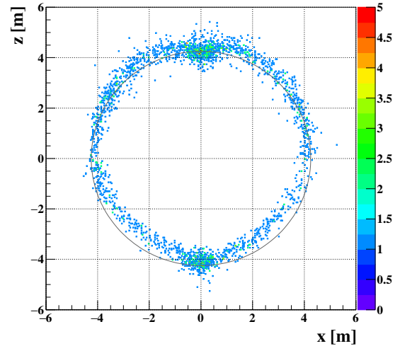
FIG. 9. A cross section ( z - x plane, |y| < 0.5 \text{ m} ) view of the distribution of 2478 events, acquired during a 3 week period, and selected for the IV shape reconstruction. The color axis represents the number of events per 0.0016 \text{ m}^3 , in a pixel of 0.04 \text{ m} \times 1.00 \text{ m} \times 0.04 \text{ m} ( x \times y \times z ). This distribution reveals the IV shift and deformation with respect to its nominal spherical position shown in solid black line.
