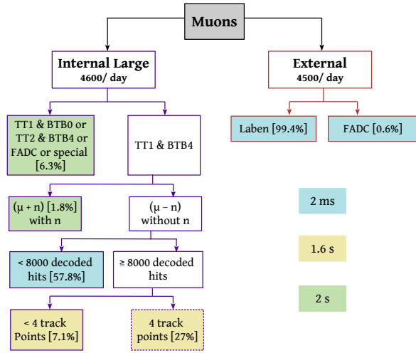
FIG. 23. Scheme of different types of vetoes applied after various muon categories. The relative fraction of each muon category is given by the numbers in brackets. Different colours represent different durations of the time veto. The dashed line around the box at the bottom of the plot represents the only muon category when the cylindrical veto around the muon track is applied. For other categories, the whole detector is vetoed.
