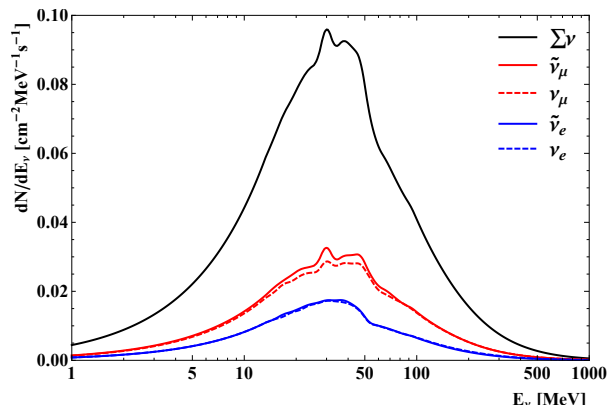
FIG. 20. Energy spectra of atmospheric neutrinos as created in the atmosphere by cosmic rays, obtained with the HKKM2014 and FLUKA simulations.
