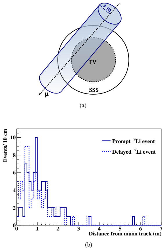
FIG. 25. Top (a): A schematic representation of the cylindrical veto applied around the muon track for 1.6 s after the (\mu - n)_{\geq 8000} muons with reliable track reconstruction. Bottom (b): Distributions of the distances of 85 {}^9\text{Li} IBD-like events from reliably reconstructed tracks of (\mu + n) muons: solid and dashed lines represent the prompt and delayed candidates, respectively.
