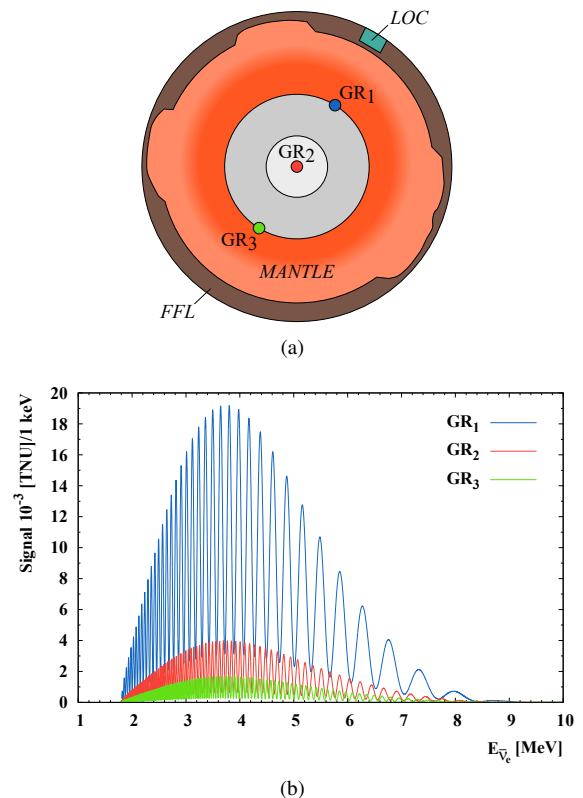
FIG. 21. Hypothetical georeactor: (a) schematics of the three studied locations: the Earth’s center (GR2) and the core-mantle-boundary (GR1 and GR3). The green area labeled LOC shows the position of the local crust around LNGS. Not to scale. (b) The oscillated antineutrino spectra expected at LNGS from 1 TW georeactor positioned at the three locations.
