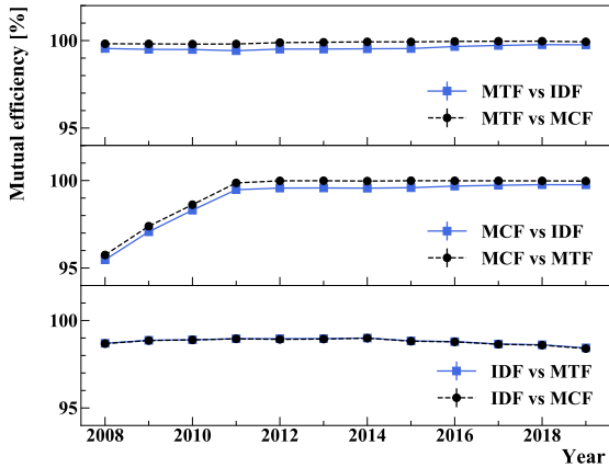
FIG. 7. Mutual efficiencies of the three strict muon flags MTF (top), MCF (middle), and IDF (bottom) for events with N_h > 80 calculated for calendar years (2019 contains data up to end of April).
