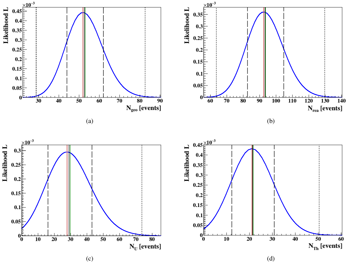
FIG. 49. The likelihood profiles for the number of geoneutrino events N_{\text{geo}} (a) and reactor antineutrino events N_{\text{rea}} (b) obtained from the fit assuming the chondritic Th/U ratio. The lower row shows the likelihood profiles for the number of ^{238}\text{U} (c) and ^{232}\text{Th} (d) events obtained from the fit assuming the ^{238}\text{U} and ^{232}\text{Th} contributions as the two independent free fit components. In each plot, the vertical solid red line indicates the best fit, while the vertical solid black and green lines indicate the median and mean values of the distributions, respectively. The vertical dashed/dotted lines show the 68%/99.7% confidence intervals of the distributions, corresponding to the signal values given in Table XVII.
