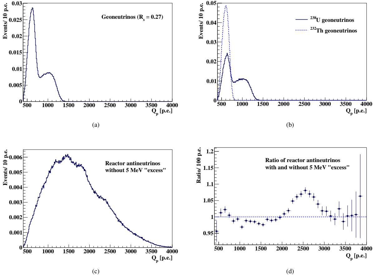
FIG. 32. The MC-based PDFs normalized to one, i.e. the expected shapes of prompts for geoneutrinos and reactor antineutrinos, after optimized geoneutrino selection cuts, that include the detector response. Top-left: geoneutrinos with Th/U ratio fixed to the chondritic value ( R_s = 0.27 ). Top-right: ^{238}\text{U} and ^{232}\text{Th} PDFs shown separately. Bottom-left: reactor antineutrinos “without 5 MeV excess”. Bottom-right: ratio of reactor antineutrino spectra “with/without 5 MeV excess” (Sec. 5.3), normalized to the same number of events each, in order to demonstrate the difference in shape only.
