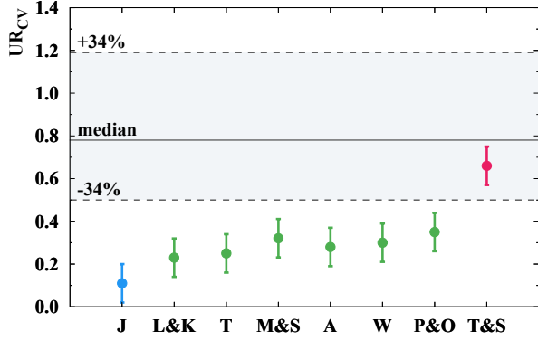
FIG. 56. Comparison of Borexino constraints (horizontal band) with predictions of the BSE models (points with \pm 3\sigma error bars, Table VII) for the convective Urey ratio UR_{CV} (Eq. 6), assuming the total heat flux H_{tot} = (47 \pm 2) TW and the radiogenic heat of the continental crust H_{rad}^{CC} = 6.8_{-1.1}^{+1.4} TW (Table V). The blue, green, and red colours represent different BSE models (CC, GC, and GD; Table VII, respectively).
