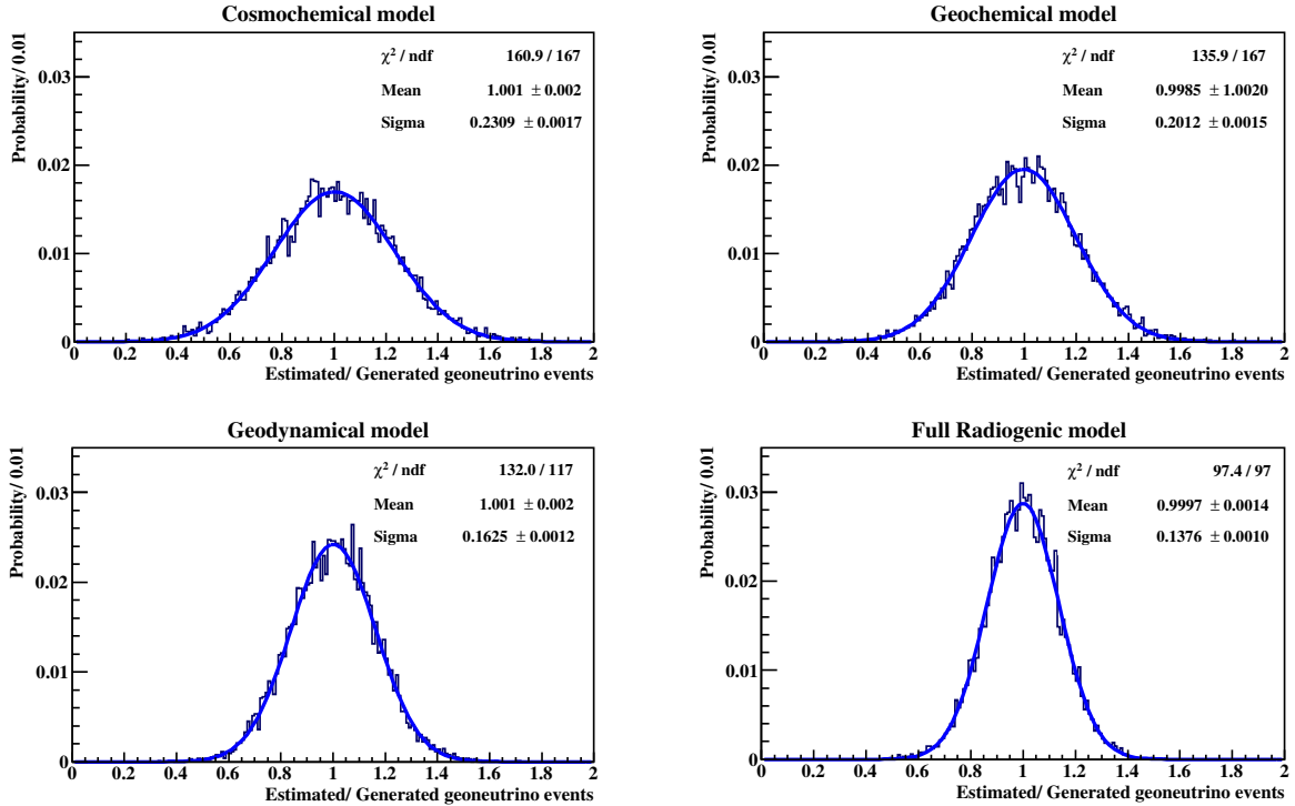
FIG. 43. Results of the sensitivity study for geoneutrinos considering the conditions of the presented analysis: the PDFs for the ratio Estimated / Generated geoneutrino events for the CC, GC, GD, and FR Earth models and corresponding fits. Each PDF is based on 10,000 generated spectra. The Gaussian fits are all centered at one, so no systematic bias is expected; their \sigma 's vary from (13.76 \pm 0.10)\% to (23.09 \pm 0.17)\% , depending on the expected geoneutrino signal for different BSE models (Table XIV) and represent the expected statistical uncertainty of the measurement.
