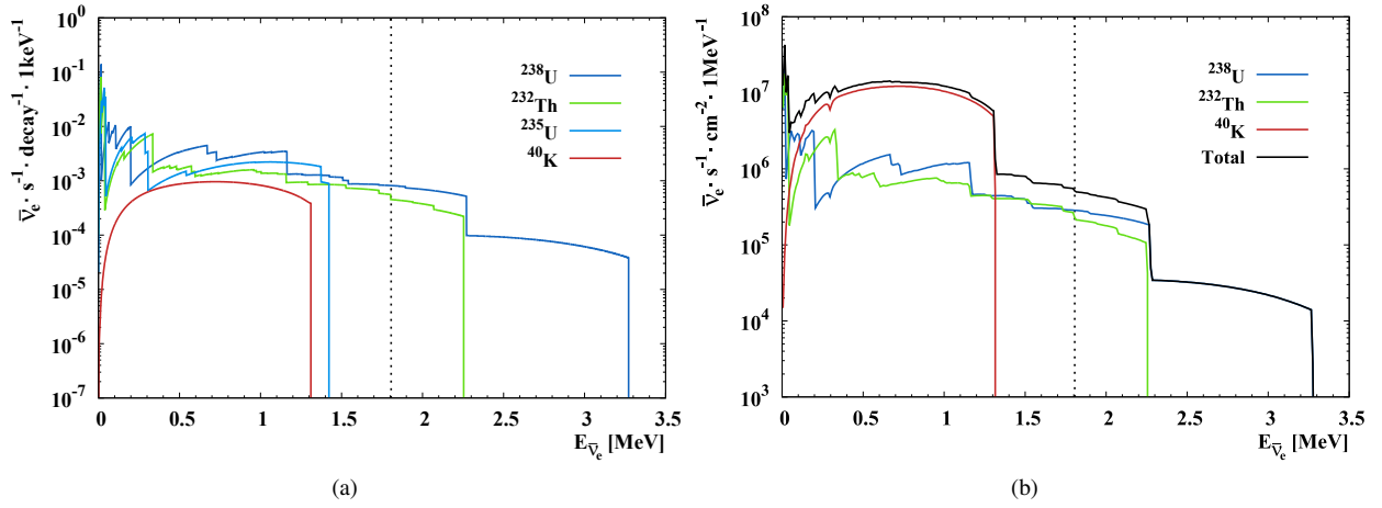
FIG. 14. (a) Geoneutrino energy spectra from the decays of ^{40}\text{K} and of the ^{238}\text{U} , ^{235}\text{U} , and ^{232}\text{Th} chains. All spectra are normalized to one decay of the head element of the chain. The integral from zero to the end point of the total spectrum is 6 for ^{238}\text{U} , 4 for ^{235}\text{U} and ^{232}\text{Th} , and 0.89 for ^{40}\text{K} . Data are from [85]. (b) Geoneutrino fluxes from different isotopes and their sum at LNGS as a function of geoneutrino energies calculated adopting geophysical and geochemical inputs from [35] for the far-field lithosphere and from [65] for the local crust. The flux from the mantle is calculated assuming a two-layer distribution (Fig. 16b) and adopting HPEs' abundances in BSE according to the GC model. The vertical dashed lines in both plots represent the kinematic threshold of the IBD interaction.
