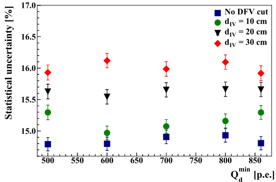
FIG. 31. The expected precision of the geoneutrino measurement for different DFV cuts. For a given DFV cut, the choice of Q_d^{\min} , shown on the x -axis, does not strongly influence the geoneutrino expected precision. Also note, that for d_{IV} = 10 cm (final choice) and no DFV cut, the sensitivity to geoneutrinos is nearly the same.
