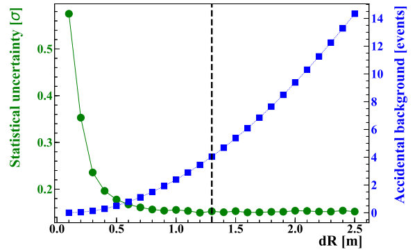
FIG. 28. The expected statistical uncertainty of the geoneutrino measurement using the MC study (filled green circles) and the accidental background (filled blue squares) for different values of dR cut, while the other cuts were set to the optimized values. The vertical dashed line shows the selected value for the dR cut at 1.3 m.
