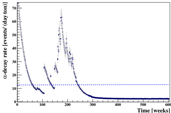
FIG. 38. The evolution of the weekly ^{210}\text{Po} \alpha -decay rates in the DFV of geoneutrino analysis, in the period from December 2007 to April 2019. The horizontal line shows the mean rate \overline{R}_{\text{DFV}}(^{210}\text{Po}) = (12.75 \pm 0.08) events/(day-ton).
