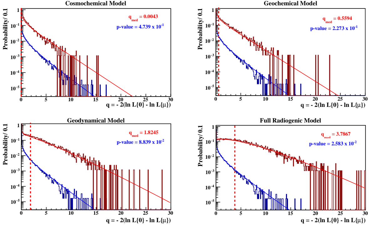
FIG. 45. Distributions of the test statistics q = -2(\ln L\{0\} - \ln L\{\mu\}) , where L\{0\} and L\{\mu\} are likelihoods of the best fits obtained with the mantle contribution fixed to zero and left free, respectively. Brown solid represents the q values obtained from 10,000 pseudo-experiments with the generated mantle geoneutrino signal, based on the predictions of the different geological models (CC, GC, GD, and FR) and fit with f(q|\mu) according to Eq. 40. The dark blue points show q = q_0 test statistics obtained using 1.2M pseudo-experiments without any generated mantle signal and fit with f(q|0) (Eq. 39). The vertical dashed lines represent the medians q_{med} of the q distributions. The corresponding p -values are also shown. From the top left to the bottom right panels, the q_{med} values are increasing because of increasing expected mantle signal (i.e. increasing predicted U and Th masses in the mantle).
