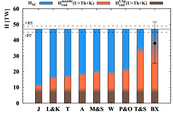
FIG. 55. Decomposition of the Earth's total surface heat flux H_{\text{tot}} = (47 \pm 2) \text{ TW} (horizontal black lines) into its three major contributions - lithospheric (brown) and mantle (orange) radiogenic heat H_{\text{rad}}^{\text{LSp}} and H_{\text{rad}}^{\text{mantle}} , respectively, and secular cooling H_{\text{Sc}} (blue). The labels on the x axis identify different BSE models (Table VII), while the last bar labeled BX represents the Borexino measurement. The lithospheric contribution H_{\text{rad}}^{\text{LSp}} = 8.1^{+1.9}_{-1.4} \text{ TW} (Table V) is the same for all bars. The amount of HPEs predicted by BSE models determines the mantle radiogenic heat (Table VII), while for Borexino the value of 30.0^{+13.5}_{-12.7} \text{ TW} is inferred from the extracted mantle signal. The difference between H_{\text{tot}} and the respective total radiogenic heat is assigned to the heat from secular cooling of the Earth.
