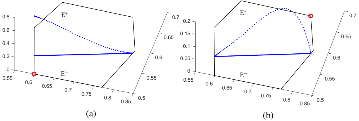
Figure 1: Trace of the approximation N_j of \varphi_j along the crack on a hexagonal element, where \varphi_j is the virtual shape function associated with the node j that is marked by the circle in (a) and (b).
