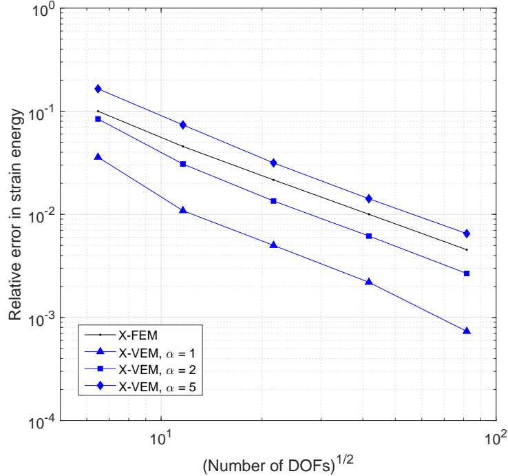
Figure 18: Influence of the stabilization parameter \alpha on the relative error in the strain energy for the inclined crack problem.
