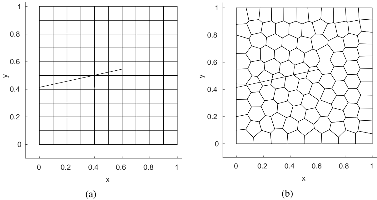
Figure 15: Representative meshes made of (a) square elements and (b) polygonal elements for the inclined crack problem.
