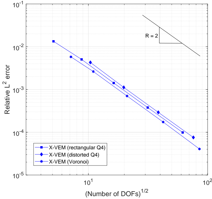
Figure 11: Convergence in terms of relative L^2 error using geometric enrichment ( r_e = 0.5 ). Extended virtual element computations are done with the elliptic projector \Pi_X^V on quadrilateral and polygonal meshes. All methods converge with a rate close to 2.
