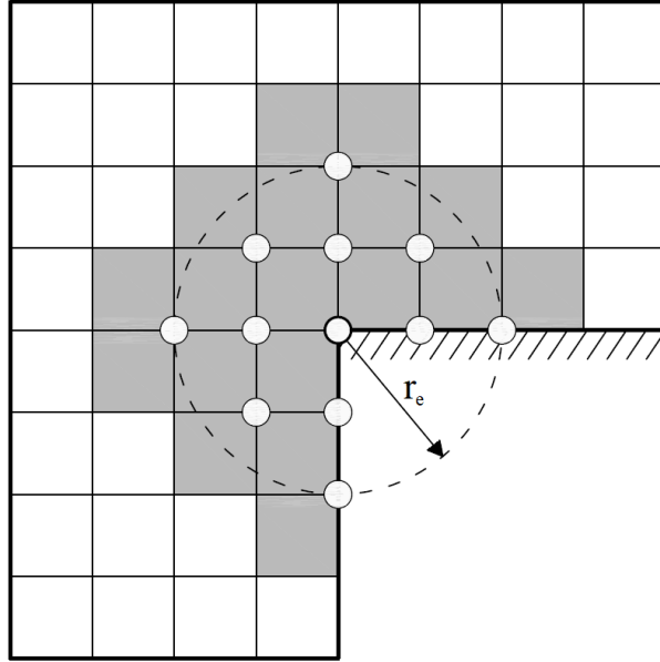
Figure 9: L -shaped domain problem where nodes that lie within the ball of radius r_e = 0.5 are enriched (geometric enrichment).
