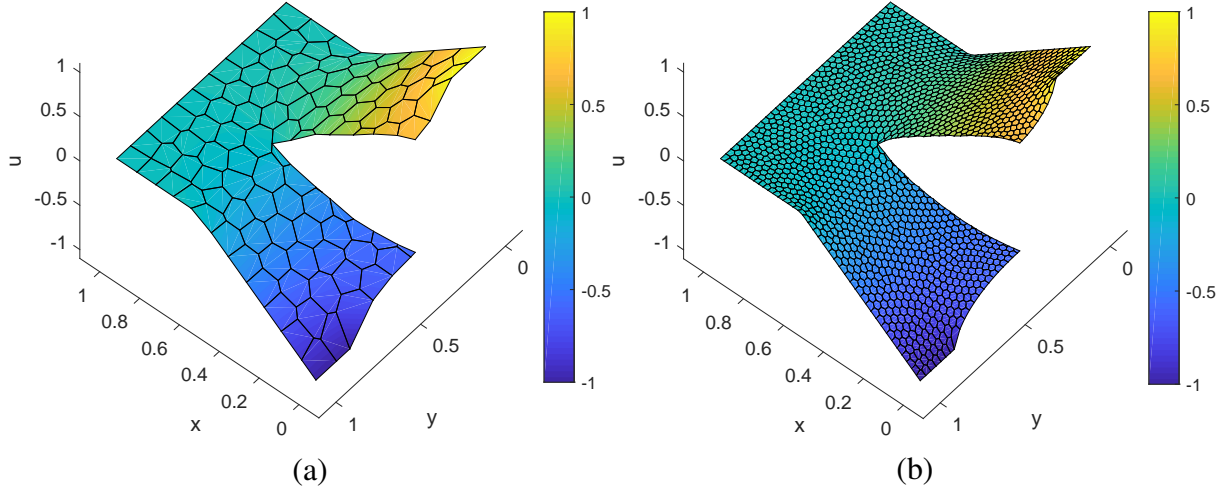
Figure 16: X-VEM contour plots of the deformed cracked membrane under mode III loading obtained from polygonal meshes with respectively (a) 100 elements and (b) 1600 elements.
