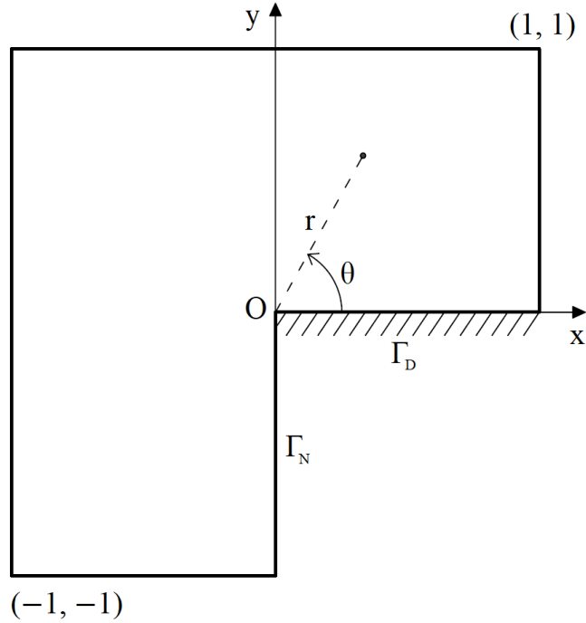
Figure 3: Geometry and boundary conditions for the L-shaped domain Laplace problem.
