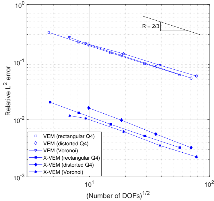
Figure 7: Convergence in terms of relative L^2 error for the L -shaped domain problem where only the node at the re-entrant corner is enriched (topological enrichment). Comparisons are made with the standard VEM on quadrilateral and polygonal meshes. All methods converge with a rate close to 2/3 .
