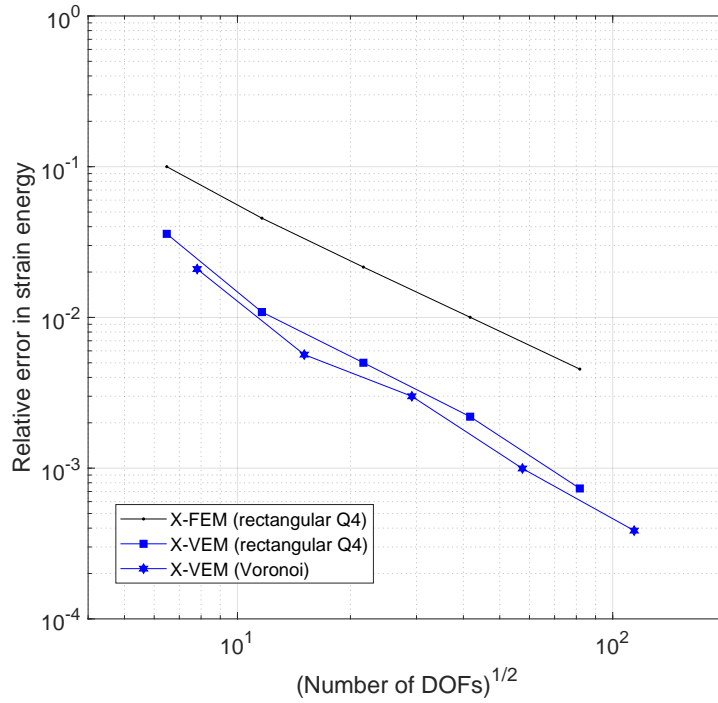
Figure 17: Convergence in terms of relative error in strain energy for the inclined crack problem using \alpha = 1 .
