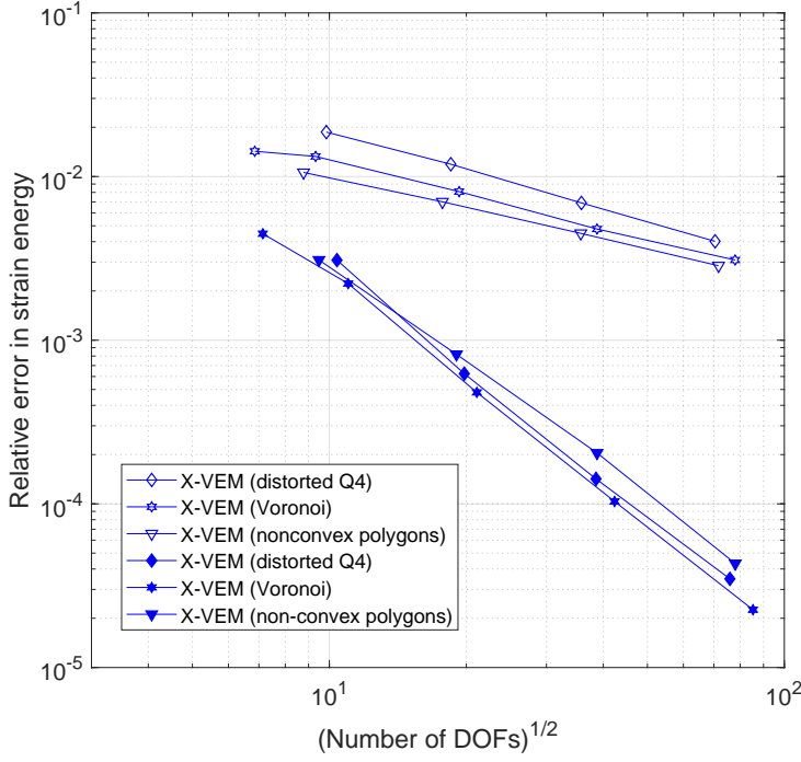
Figure 12: Comparison between convergence plots in terms of relative error in strain energy using topological enrichment (hollow markers) and geometric enrichment with r_e = 0.5 (solid markers). Extended virtual element computations are performed with the elliptic projector \Pi_X^\nabla on distorted quadrilateral, polygonal and non-convex polygonal meshes.
