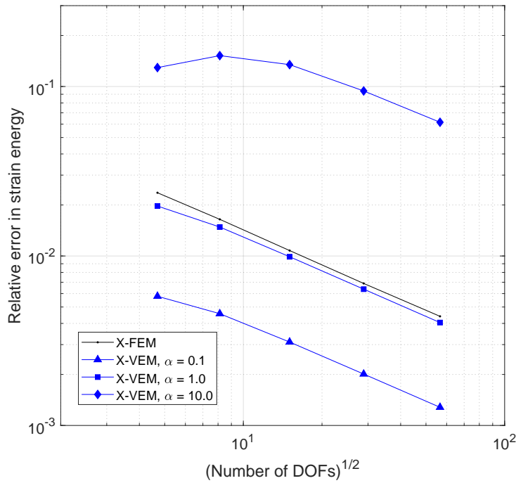
Figure 8: Sensitivity of the convergence to the stabilization parameter \alpha for the L -shaped domain problem where only the node at the re-entrant corner is enriched (topological enrichment).
