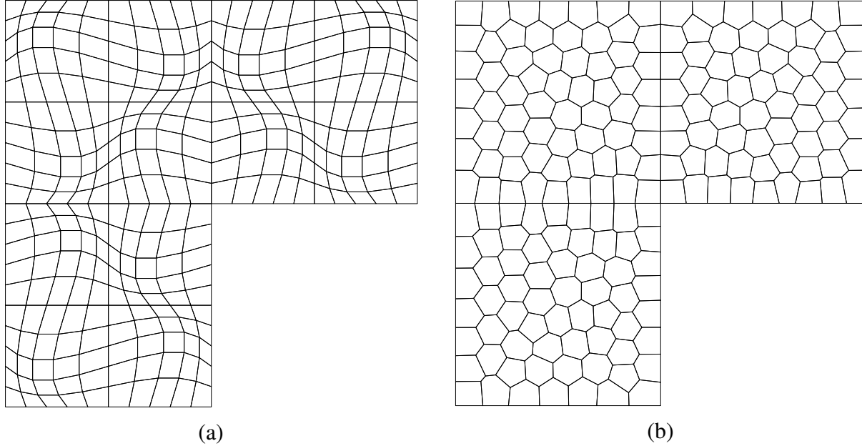
Figure 4: Representative meshes made of (a) distorted quadrilaterals and (b) convex polygons for the L -shaped domain problem.
