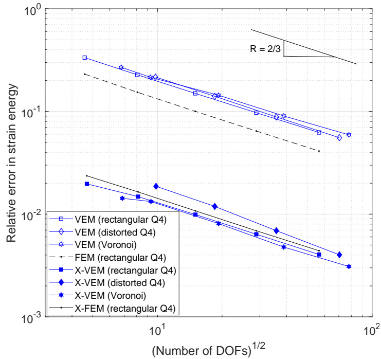
Figure 6: Convergence in terms of relative error in strain energy for the L -shaped domain problem where only the node at the re-entrant corner is enriched (topological enrichment). Comparisons are made with both the standard VEM and standard FEM/X-FEM (from [33]) on quadrilateral and polygonal meshes. All methods converge with a rate close to 2/3 .
