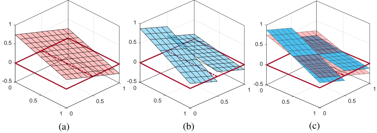
Figure 2: (a) Projection onto \mathbb{P}_1(E) of one of the virtual basis functions \varphi_j of a square element. (b) Separate projections of \varphi_j^+ and \varphi_j^- onto \mathbb{P}_1(E^+) and \mathbb{P}_1(E^-) , respectively. (c) Superposition of the three projections.
