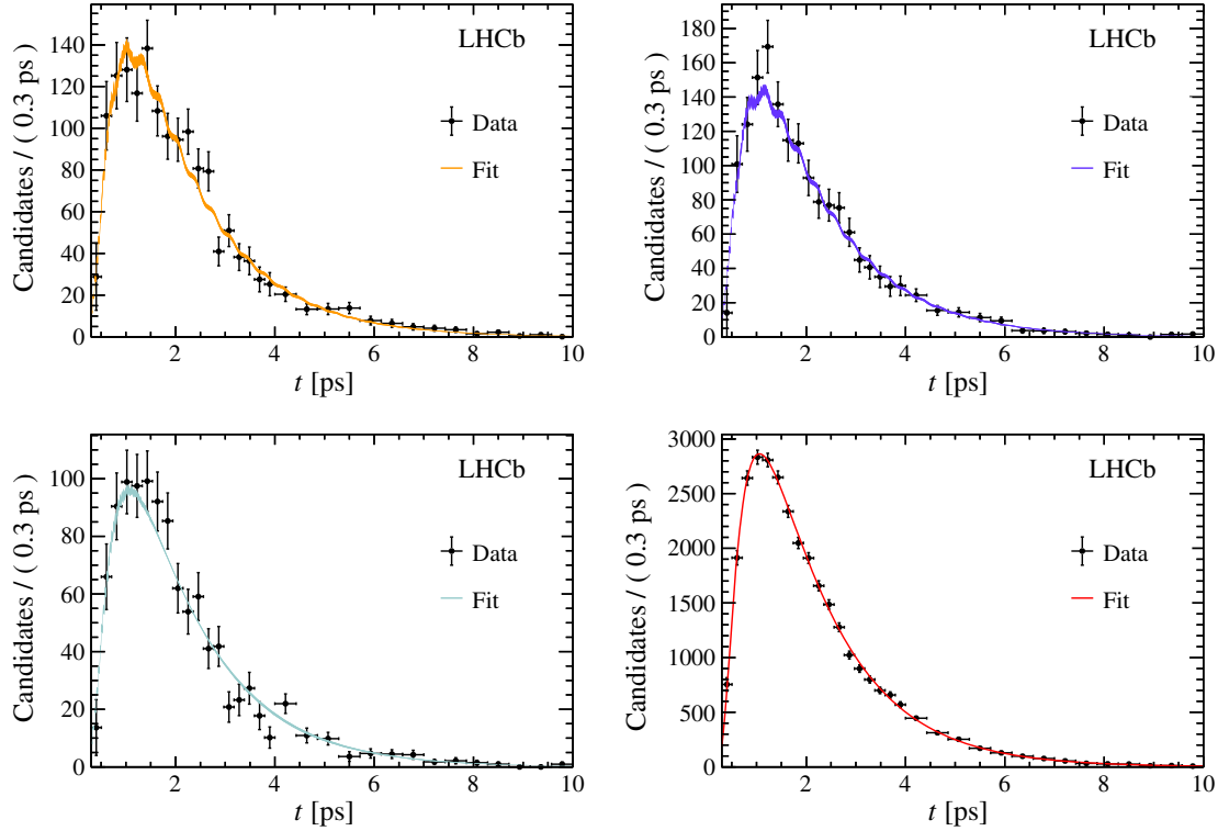
FIG. 2. Decay-time fit projections. The top row corresponds to the tagged (left) B_s^0 \rightarrow \phi\gamma and (right) \bar{B}_s^0 \rightarrow \phi\gamma candidates, while the bottom plots show the (left) untagged B_s^0 \rightarrow \phi\gamma and (right) B^0 \rightarrow K^{*0}\gamma candidates. The line is the result of the fit described in the text, including statistical uncertainties.
