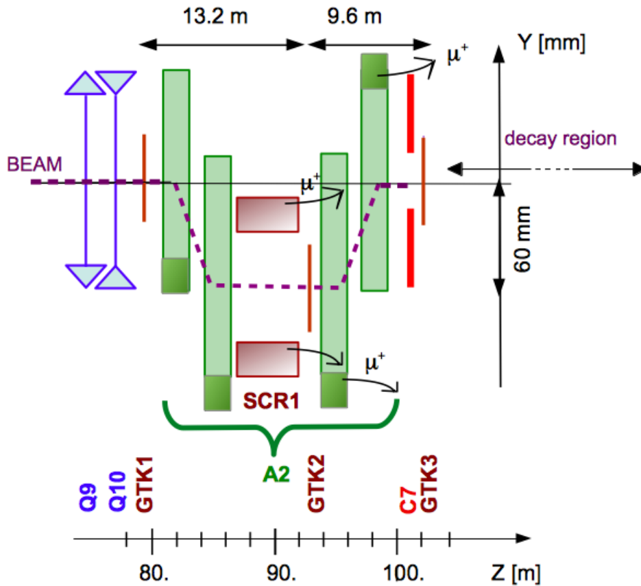
Figure 5. Schematic layout of the beam tracking and momentum measurement in the second achromat (A2). The beam is deflected vertically by 60 mm and returned to its nominal direction after the momentum measurement. Muons are swept away by the scraper SCR1 and the return yokes of the last two C-shaped magnets of the achromat (dark shaded areas).
