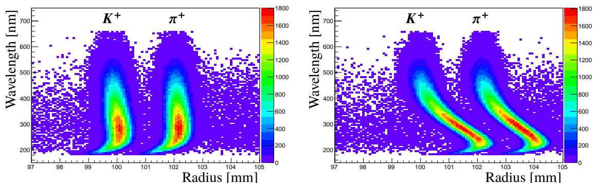
Figure 11. Simulated distributions of wavelength vs radius at the CEDAR diaphragm plane for Cherenkov photons produced by the K^+ and \pi^+ beam for N_2 (left) and H_2 (right) radiator, weighted with the quantum efficiency [18].
