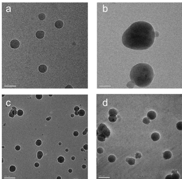
Fig. 6 Cryo-TEM images recorded for 90/10 H 2 O:dioxane samples of nanosized aggregates of complex 1 (a, b) and 3 (c, d) at concentration of 1.0 \times 10^{-4} M. Scale bar is 50 and 100 nm for a, b and c, d, respectively.
