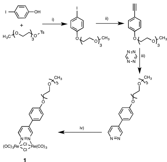
Scheme 1 General schematic synthetic pathway followed for the preparation of the luminescent rhenium metallo-amphiphile 1 . Reaction conditions: (i) K_2CO_3 , Bu_4NBr , 90\text{ }^\circ\text{C} ; (ii) ethynyltrimethylsilane, Pd(PPh_3)_4 , CuI , iPr_2NH , 90\text{ }^\circ\text{C} ; (iii) NH_2NH_2 \cdot H_2O , formamidine acetate, room temperature; (iv) [Re(CO)_5Cl] , toluene, reflux.
