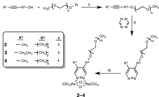
Scheme 2 General schematic synthetic pathway followed for the preparation of the luminescent rhenium metallo-amphiphiles 2–4 . Reaction conditions: (i) NaH , THF , 0\text{ }^\circ\text{C} → room temperature; (ii) NH_2NH_2 \cdot H_2O , formamidine acetate, room temperature; (iii) [Re(CO)_5Cl] , toluene, reflux.
