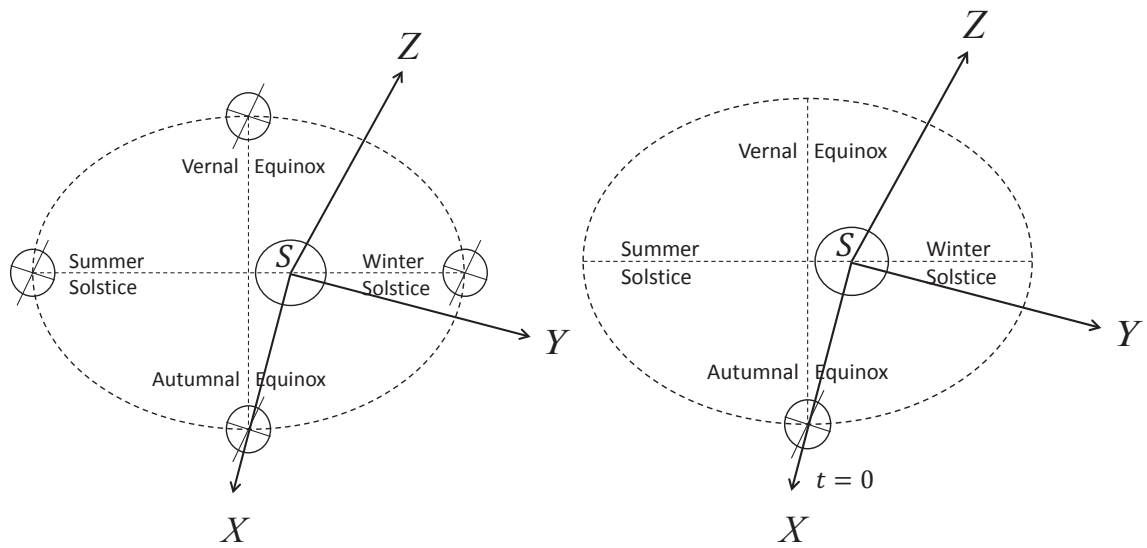
Figure 12-6: The definition (left panel) of the sun-centered system [444, 445], and definition (right panel) of t = 0 in the sun-centered system.
