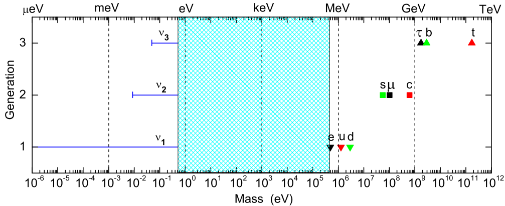
Figure 1-1: A schematic illustration of the “flavor hierarchy” and “flavor desert” in the fermion mass spectrum at the electroweak scale [30]. Here the neutrino masses are assumed to have a normal ordering.
