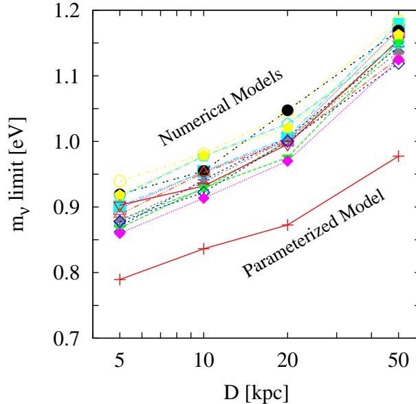
Figure 4-9: The upper bounds on the absolute scale of neutrino masses at the 95% CL for a SN at a distance of D = 5 kpc, 10 kpc, 20 kpc and 50 kpc in the parameterized model from Ref. [204], and a series of numerical models from Ref. [183], in which simulations have been performed for a progenitor-star mass M = 13, 20, 30 or 50 solar masses, a metallicity Z = 0.02 or 0.004, and a shock revival time t_{\text{revive}} = 100 ms or 300 ms. In our calculations, we have chosen fourteen numerical models, since a black hole is formed 842 ms after bounce in two models with M = 30 solar masses and Z = 0.02 . See Ref. [183] for more details about the numerical models, and the SN neutrino data are publicly available at the website http://asphwww.ph.noda.tus.ac.jp/snn/ . This figure is taken from Ref. [207]
