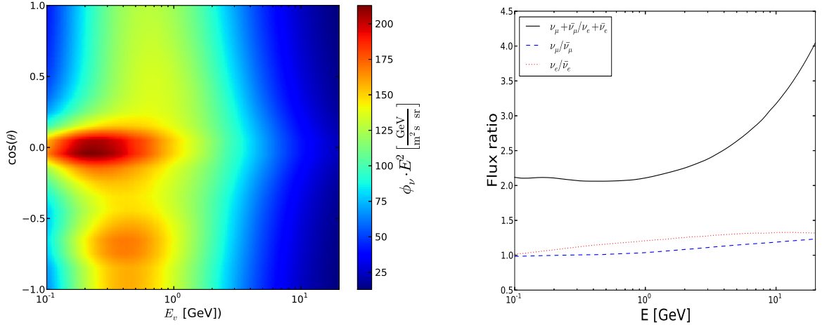
Figure 7-1: The differential \nu_\mu flux density multiplied with E^2 versus energy and zenith angle (left) and flux ratios of different flavors versus energy averaged over all zenith angles (right).
