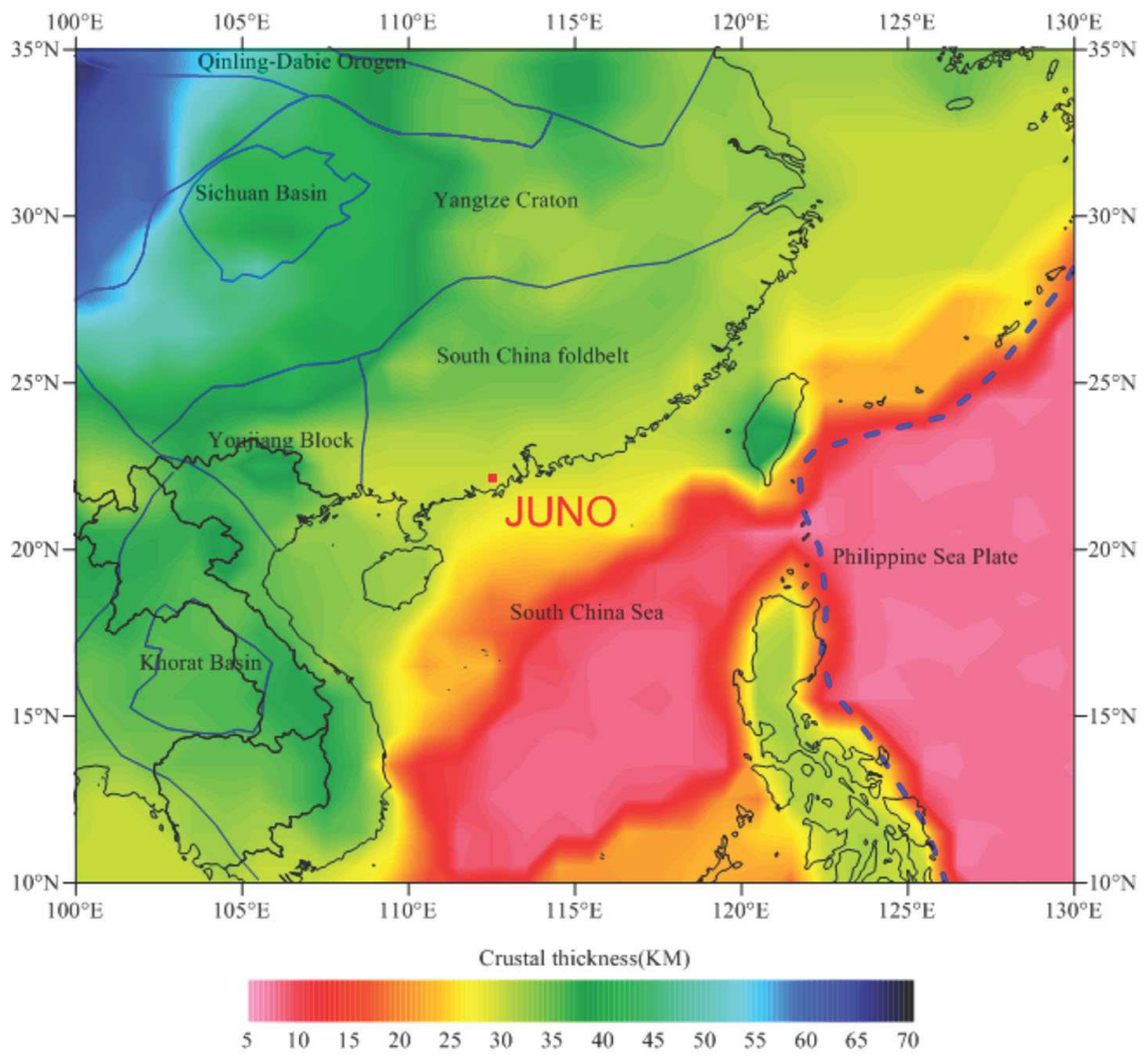
Figure 8-3: Crustal thickness (exclusive water) in the surrounding area of JUNO from CRUST 1.0 model, 1° degree [340]. Dashed thick blue line is plate boundary [341]. Thin blue lines denote the main tectonic units.
