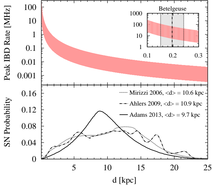
Figure 4-7: Maximum IBD rate at JUNO as a function of the distance to a galactic SN. In the upper panel, the shaded range has been obtained by considering a class of SN models from the Basel [180], Garching [181, 182] and Nakazato [183] groups. The insert refers to the SN candidate Betelgeuse with a distance of 0.197 \pm 0.045 kpc [136]. In the lower panel, the SN probability in our galaxy has been given according to three different evaluations [133–135].
