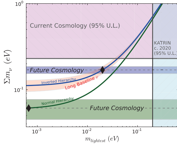
Figure 2-3: The current constraints and forecast sensitivity of cosmology to the neutrino mass in relation to MH [87]. In the case of an inverted MH in the upper curve, future combined cosmological constraints would have a very high-precision detection, with 1\sigma error shown as the blue band. In the case of a normal MH in the lower curve, future cosmology would detect the lowest \sum m_{\nu} at a level of \sim 4\sigma .
