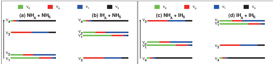
Figure 9-1: Four different scenarios of neutrino mass spectra in the (3+1) scheme, depending on the neutrino mass hierarchies of three active and one sterile neutrino mass eigenstates.
