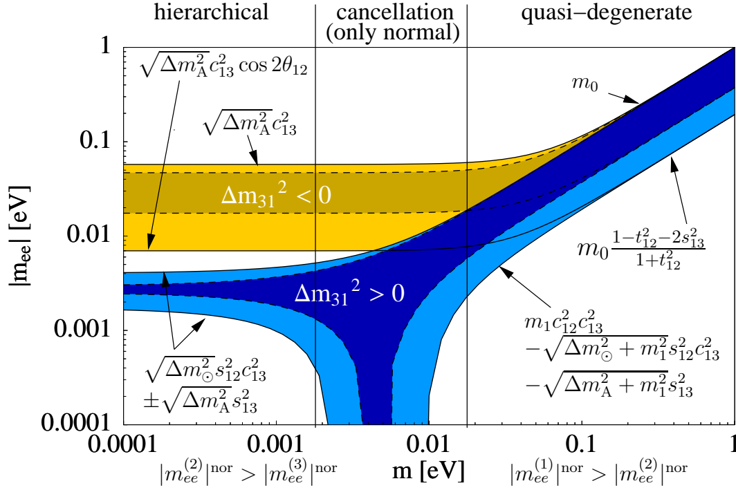
Figure 3-2: The main properties of the effective mass |m_{ee}| as a function of the smallest neutrino mass [113]. Here m denotes the common mass for the quasi-degenerate region and t_{ij} = \tan \theta_{ij} , s_{ij} = \sin \theta_{ij} , c_{ij} = \cos \theta_{ij} . Furthermore, \Delta m_A^2 and \Delta m_\odot^2 stands for the atmospheric mass-squared difference and the solar mass-squared difference, respectively.
