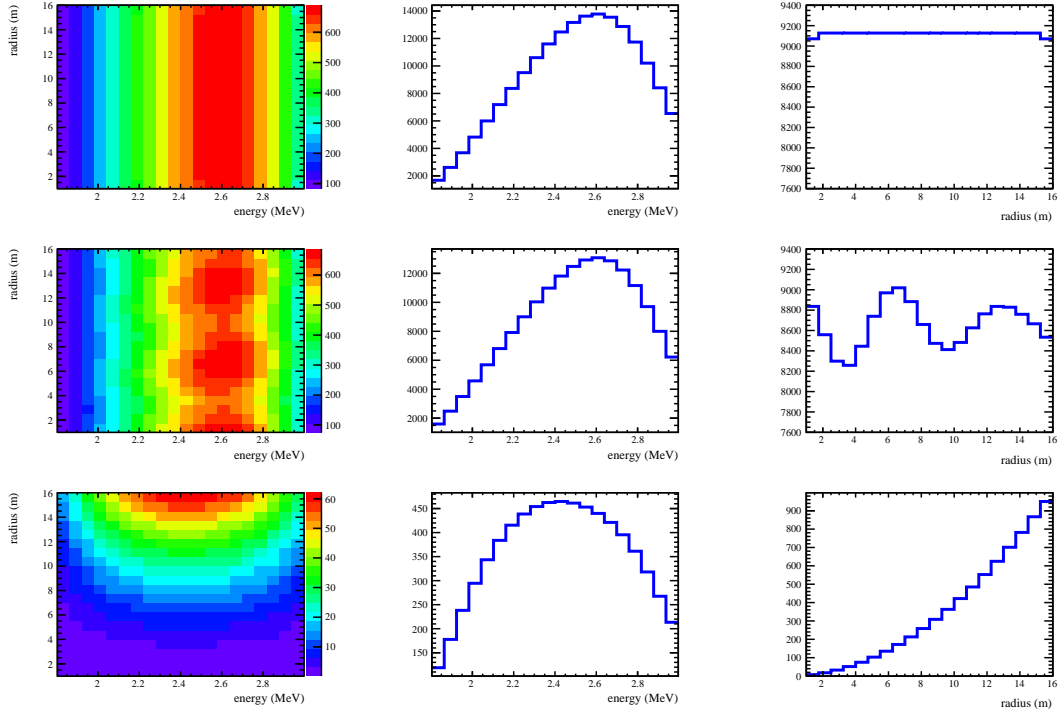
Figure 9-2: Energy and position dependence of the event numbers expected for a ^{144}\text{Ce} \bar{\nu}_e source (50 kCi, 900 days) at the center of the detector. While the top row of panels shows the signal of the antineutrino source without oscillations, the middle row illustrates the effect of \bar{\nu}_e \rightarrow \bar{\nu}_s oscillations. The bottom row illustrates the event distribution expected for the reactor antineutrino background. In each row, the left panel shows the 2-dimension distribution of the event rates as a function of signal energy, and distance from the source. The middle panels are 1-dimension projections of the energy spectrum, while right panels show the distance distributions.
