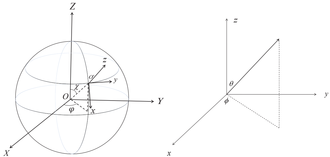
Figure 12-7: The definition of the earth-centered system (left panel) [444, 445], and definition of the local coordinate system (right panel).
