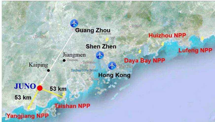
Figure 1-3: Location of the JUNO site. The distances to the nearby Yangjiang NPP and Taishan NPP are both 53 km. Daya Bay NPP is 215 km away. Huizhou and Lufeng NPPs have not been approved yet. Three metropolises, Hong Kong, Shenzhen, and Guangzhou, are also shown.
