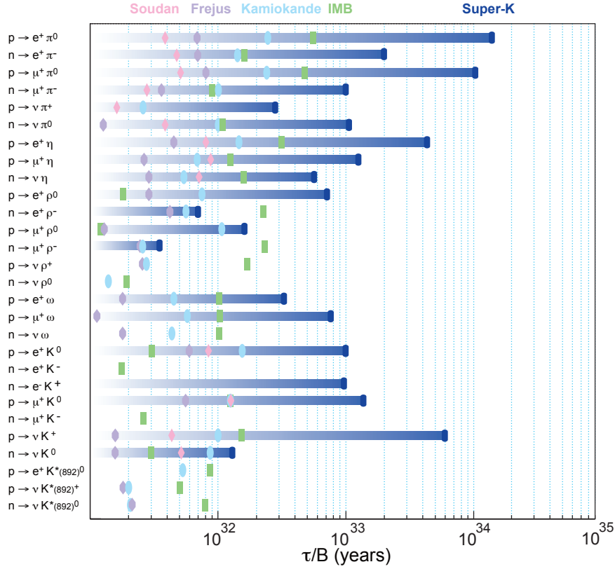
Figure 10-1: The 90% C.L. limits on the nucleon lifetimes in a variety of two-body decay modes of the nucleons [390]. Today’s best limits are mostly from the Super-Kamiokande experiment using the water Cherenkov detector.
