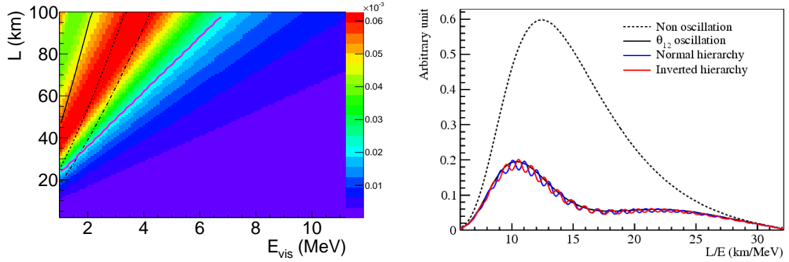
Figure 2-4: (left panel) The effective mass-squared difference shift \Delta m_\phi^2 [73] as a function of baseline (y-axis) and visible prompt energy E_{\text{vis}} \simeq E_\nu - 0.8 \text{ MeV} (x-axis). The legend of color code is shown in the right bar, which represents the size of \Delta m_\phi^2 in \text{eV}^2 . The solid, dashed, and dotted lines represent three choices of detector energy resolution with 2.8%, 5.0%, and 7.0% at 1 MeV, respectively. The purple solid line represents the approximate boundary of degenerate mass-squared difference. (right panel) The relative shape difference [56, 57] of the reactor antineutrino flux for different neutrino MHs.
