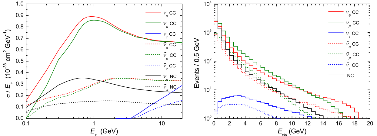
Figure 7-5: Left panel: the neutrino and antineutrino per nucleon cross sections for the LS target [311]. Right panel: the expected spectra as a function of E_{vis} for the 200 kton-years exposure.
