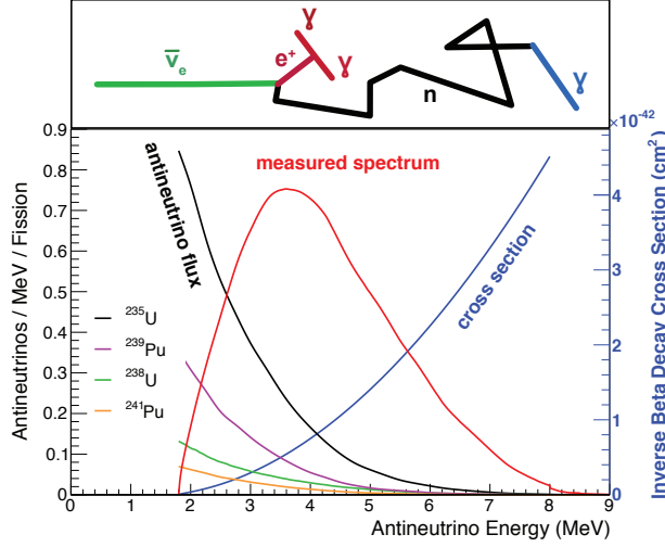
Figure 2-6: The observable \bar{\nu} spectrum (red line) is a product of the antineutrino flux from reactor and the cross section of inverse beta decay (blue line). The contributions of four fission isotopes to the antineutrino flux are shown for a typical pressurized water reactor. The steps involved in the detection are schematically drawn on the top of the figure [102].
