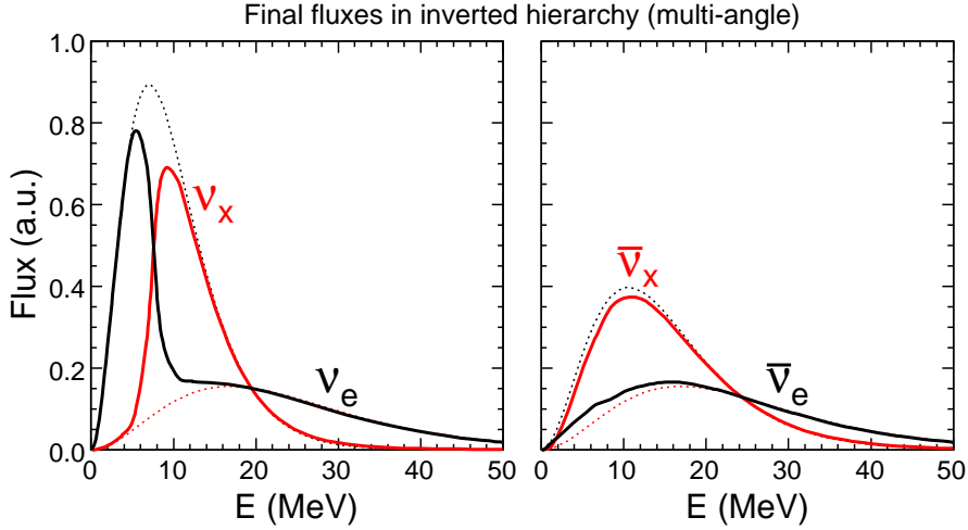
Figure 4-10: Numerical illustration for the splits in neutrino energy spectra after collective oscillations in the case of inverted mass hierarchy [209]. The initial spectra are indicated by dotted curves in the same color as the final ones, where one can observe a complete swap of the antineutrino spectra and a sharp split in the neutrino spectra.
