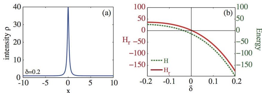
Figure 1 | (a) Density distribution \rho(x, t = 0) at fixed perturbation \delta = 0.2 , and (b) Reduced energy functional H_r = H - M \frac{\partial F}{\partial \rho} \Big|_{\rho_0} (solid line) and energy H (dashed line) vs. perturbation parameter \delta , for the perturbed antidark soliton of CQNLS equation, expressed by Eq. (22) with \alpha = 0.1 and \rho_0 = 1 .
