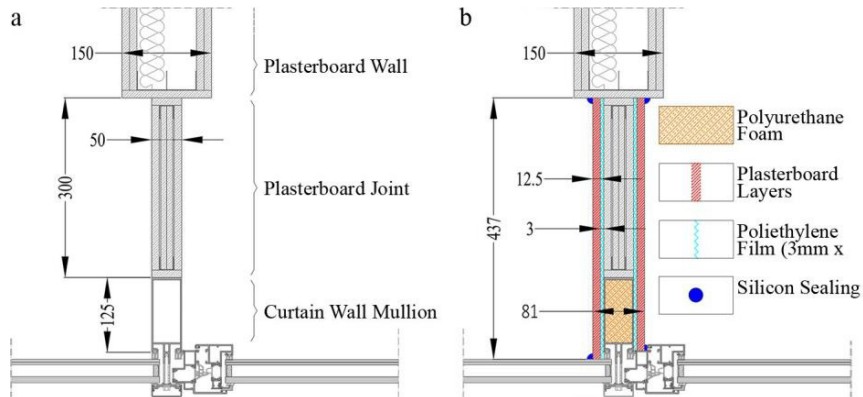
Fig. 4. The junction between the separating wall and the curtain wall before (a) and after (b) the improvement intervention. Dimensions are in mm. The main wall has a 5 cm mineral wool layer and an air gap of 5 cm.
