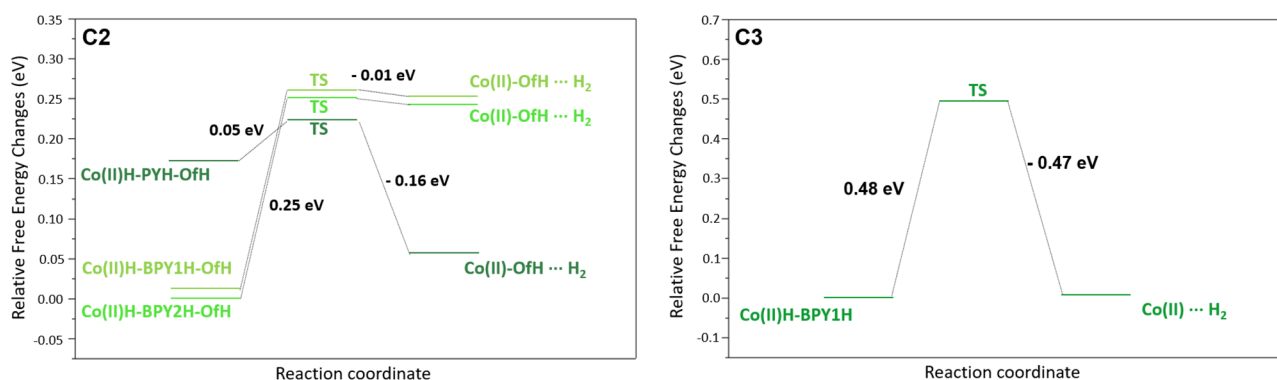
Fig. 10 Calculated free energy profiles ( \Delta G ) starting from the second protonation step until formation of H 2 , for C2 (left) and C3 (right). At this step, once formed, H 2 is still in interaction with the complex (see structures in Fig. ES26†). The structures corresponding to stationary points (minima and transition states, TS) are given in Fig. ES26,† including the imaginary frequency of the most relevant TSs.
