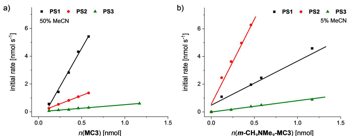
Figure 4. Catalytic performance of Ru(bda) macrocycles MC3 (a) and m -CH 2 NMe 2 - MC3 (b) in light-driven water oxidation using PS1–3 as photosensitizers. The catalytic activity was analyzed by the initial rates of catalysis at variable WOC concentrations. Measurements were performed in (a) 1:1 or (b) 5:95 MeCN/H 2 O mixtures (50 mM phosphate buffer, pH 7). Experiment conditions: (a) c(PS) = 1.5 mM, c(Na 2 S 2 O 8 ) = 37 mM; (b) c(PS) = 0.2 mM, c(Na 2 S 2 O 8 ) = 37 mM.
