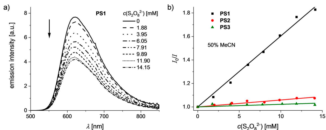
Figure 5. a) Emission spectra ( \lambda_{\text{ex}} = 453 \text{ nm} ) of PS1 in MeCN/H 2 O 1:1 (phosphate buffer, pH 7) at varying concentrations of \text{Na}_2\text{S}_2\text{O}_8 . The arrow indicates changes of emission spectra with increasing concentration of the persulfate quencher. b) Stern-Volmer plots showing linearly fitted curves for sensitizers PS1–3 in buffered MeCN/H 2 O 1:1 (pH 7). In all experiments, the concentration of the respective sensitizer was 50 \mu\text{M} .
