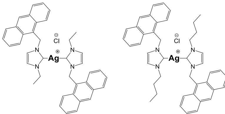
Figure 1. Molecular structure of the studied Ag(I)-bisNHC complexes.
