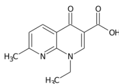
Figure 1. 1-Ethyl-7-methyl-4-oxo-[1,8]naphthyridine-3-carboxylic acid (NAL).
