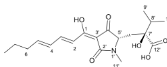
Structure of harzanic acid
