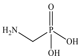
Fig. 1. Structures of aminomethylphosphonic acid (AMPA).
