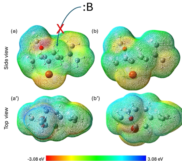
Figure 4. Potential map analysis of two possible rotamers of B around bond \text{C}_4\text{--C}_{1'} -isopropenyl. (a, a') Double bond of the isopropenyl group directed above the plane that includes the ring. (b, b') Double bond of the isopropenyl group directed below the plane that includes the ring. Geometry was optimized with a WB97XD/SMD/6–311G+(d,p) at 203 K.
