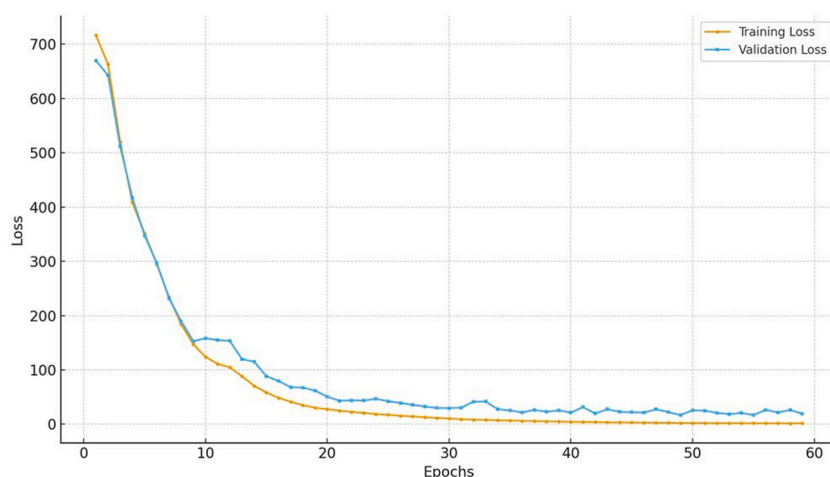
Fig 3. Training and validation loss over epochs.
