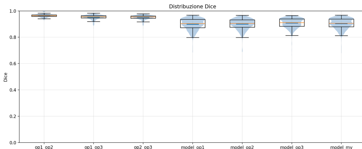
Fig 5. Distribution of Dice similarity coefficient between pairs of human raters and between the neural network and each rater. Higher values indicate better overlap.
