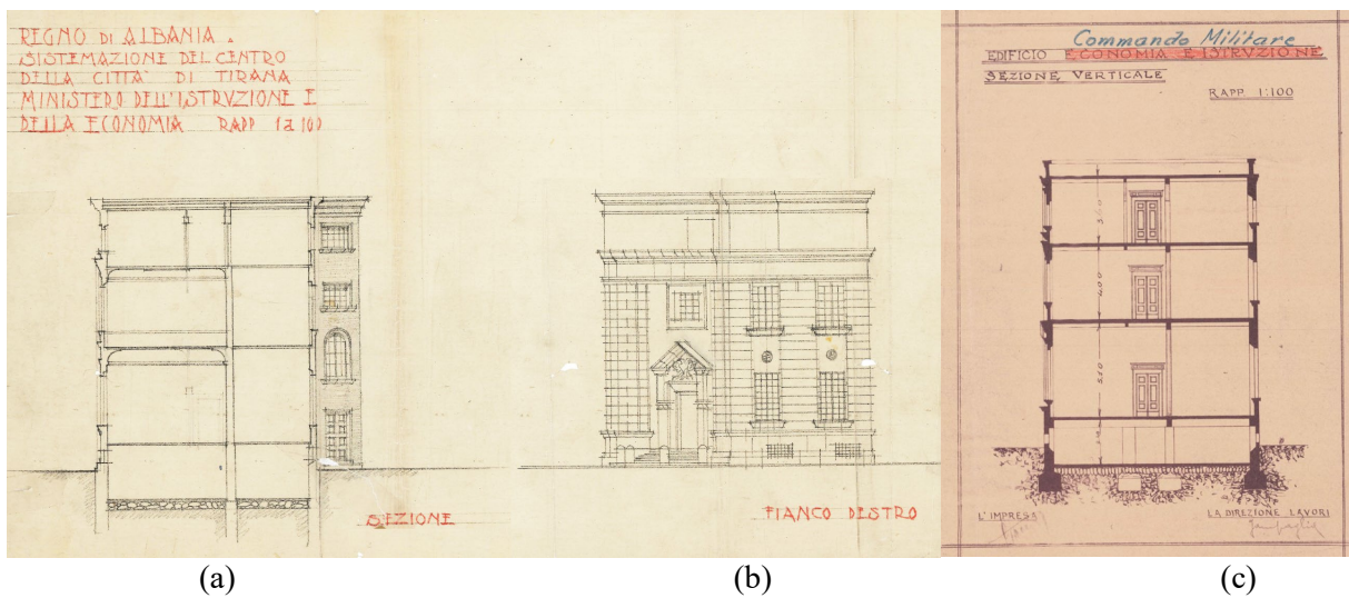
Figure 40. (a), (b) Section cut and the south façade behind, from the “F. De Fausto project idea 1929”, (c) Section cut from the implementing project 1941 (Source: AQTN)
