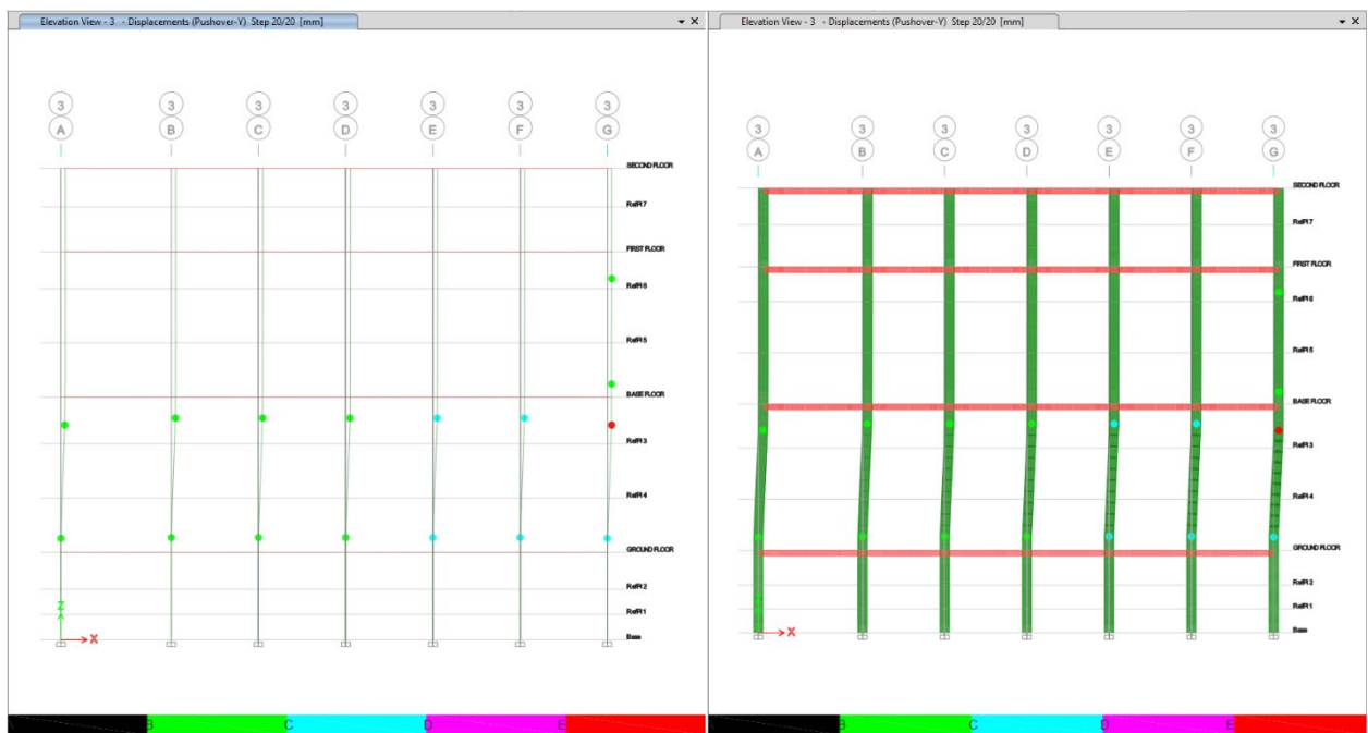
Figure 119. Appearance of plastic hinges in step-20, Axis-3, push-y loading in nonlinear analysis
