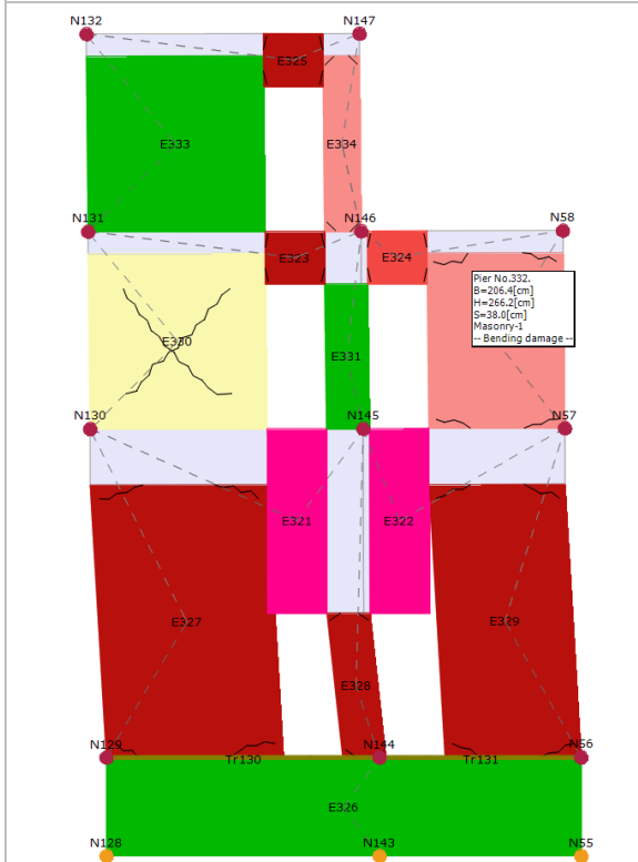
Analysis-24/Mechanism P.22 /Internal masonry /seismic dir.-Y/seismic load =static
