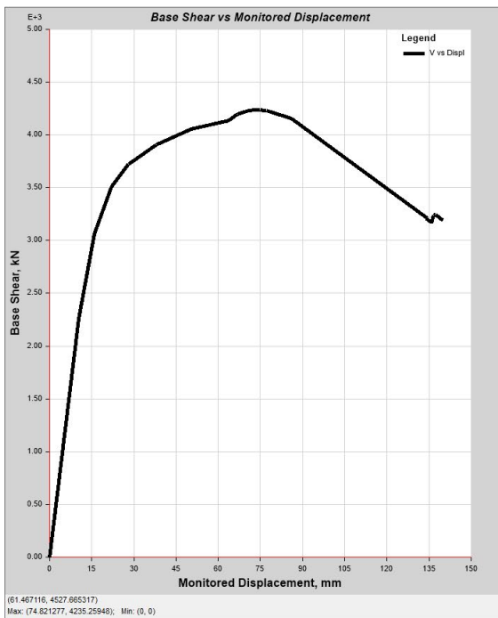
Figure 121. Generation of capacity curve in V-Δ format according to push-Y load, captured in etabs.v19
