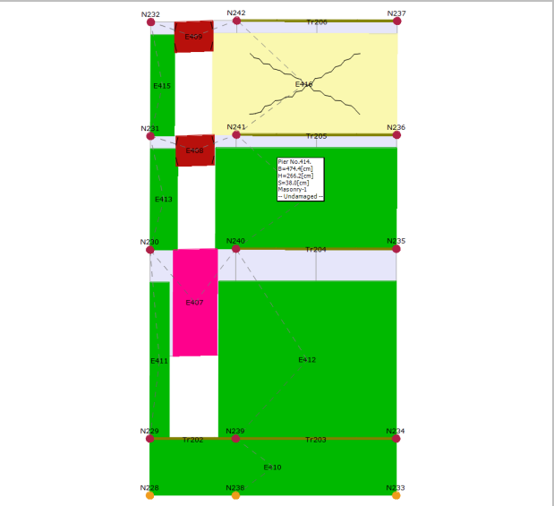
Analysis-02/Mechanism P.34 /Internal masonry /seismic dir.+X/seismic load =static
