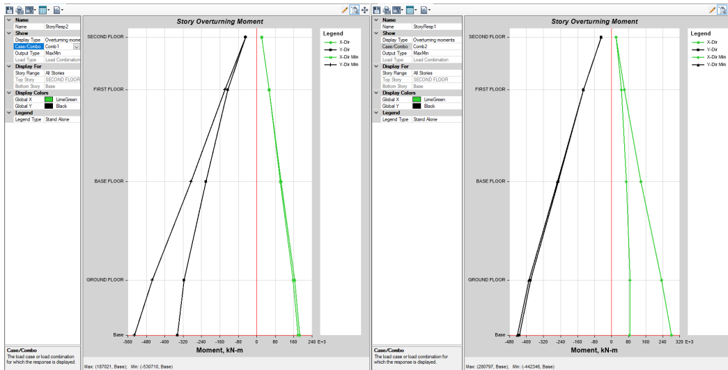
Figure 111. Story overturning moment of the building related to seismic combinations (Etabs v.19)
