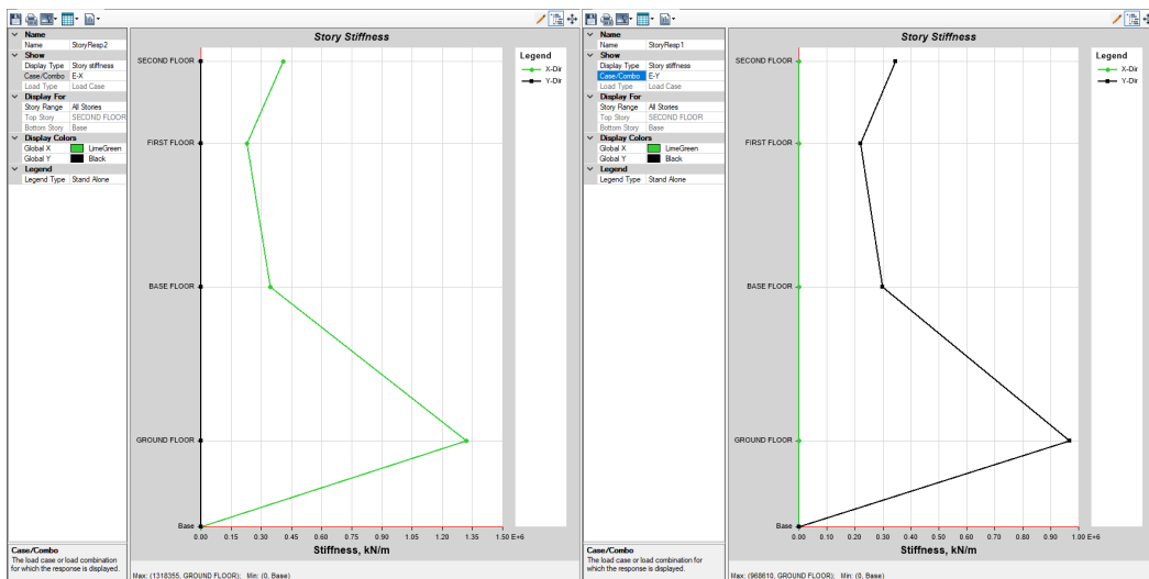
Figure 112. Story stiffness related to seismic actions x-y (Etabs v.19)
