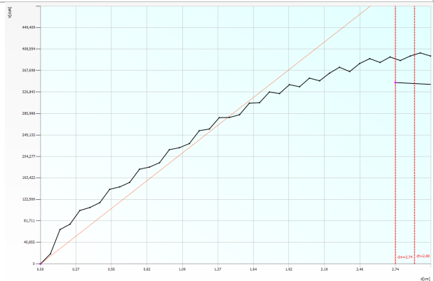
Analysis-04/Mechanism P.17 /Internal hall masonry /seismic dir.-X/seismic load =static
