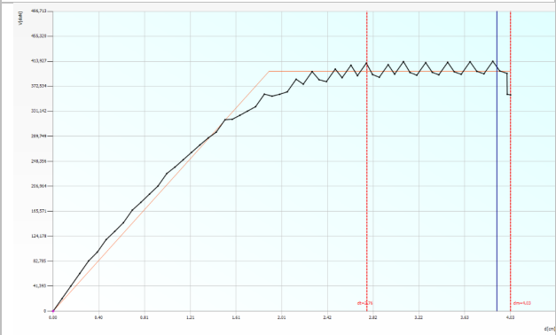
Analysis-08/Mechanism P.17 /Internal hall masonry /seismic dir.-Y/seismic load =static
