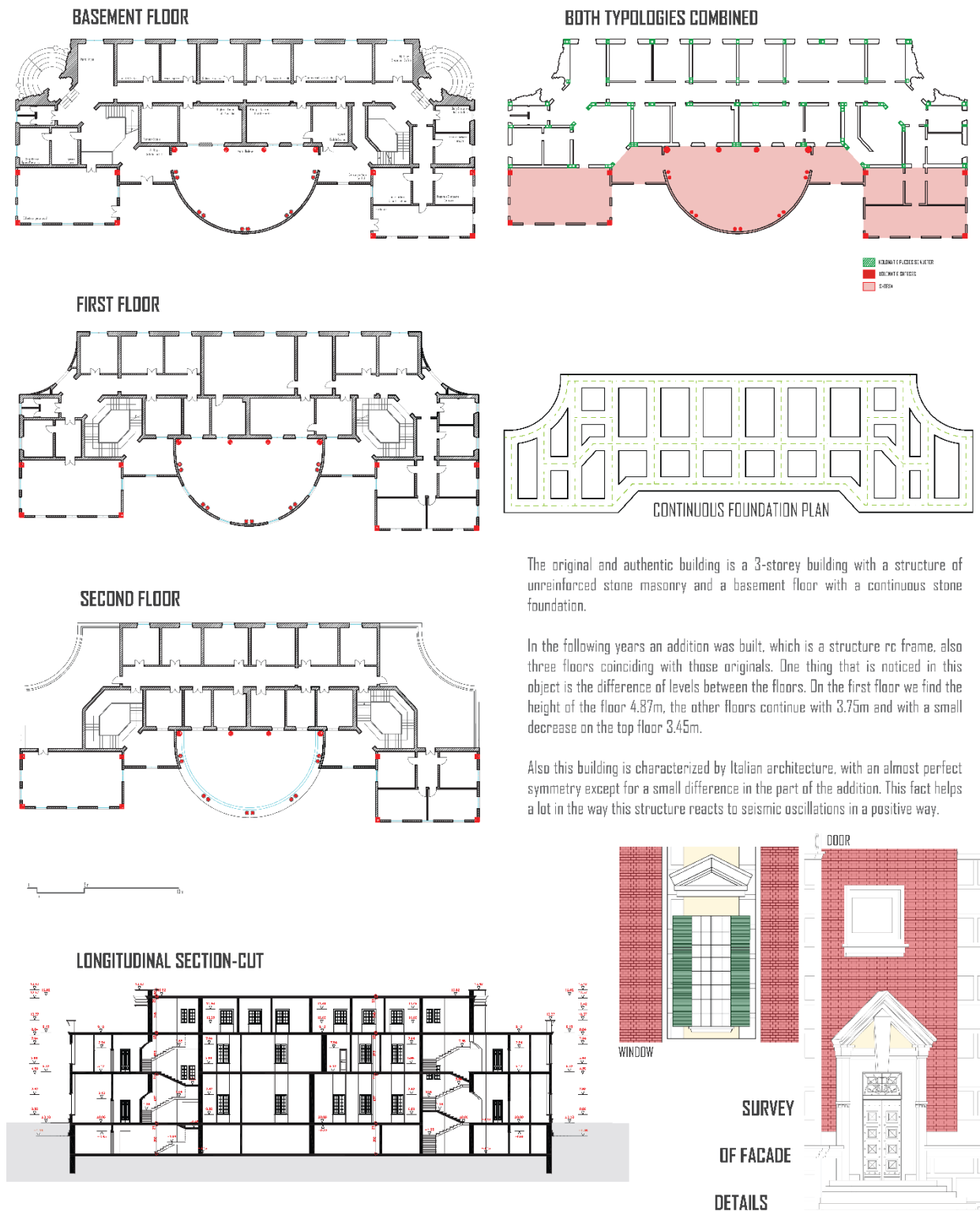
Figure 47 Parts of architectural survey process, all plans, main section cut, reports between two different typologies of structures in plan, foundation plan combined by architectural details analysed
