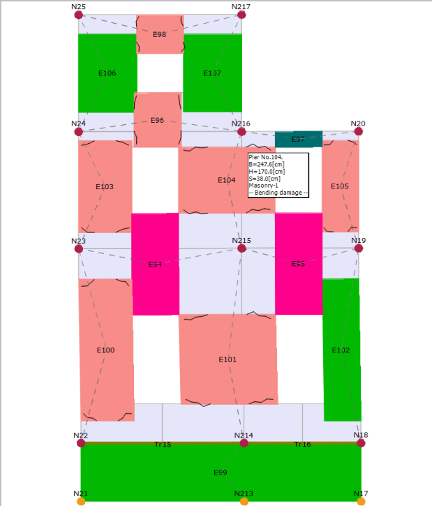
Analysis-24/Mechanism P.32 /Internal masonry /seismic dir.-Y/seismic load =static
