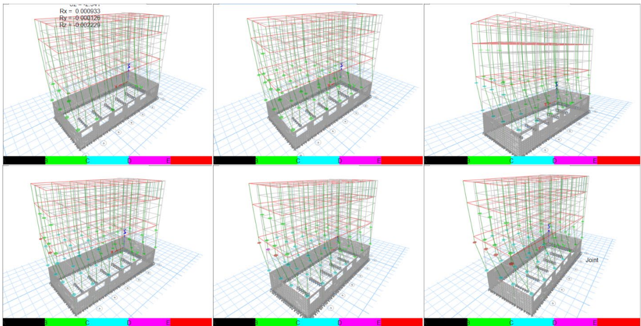
Figure 120. Combination of basic steps according to push-y loading and investigations into possible scenarios of collapse mechanisms
