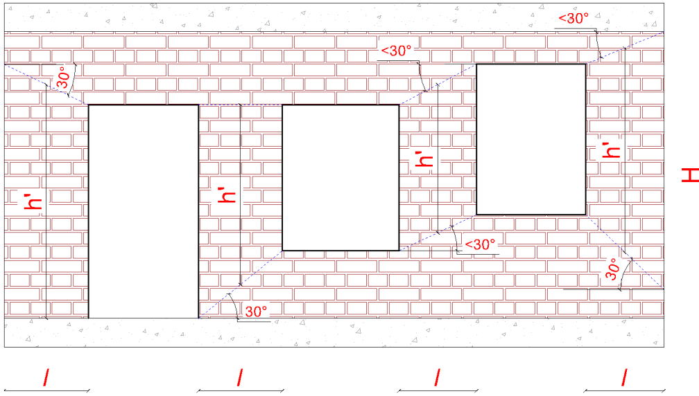
Figure 25. Experimental model with openings (Dolce, 1989/ Graphically processed by author)
