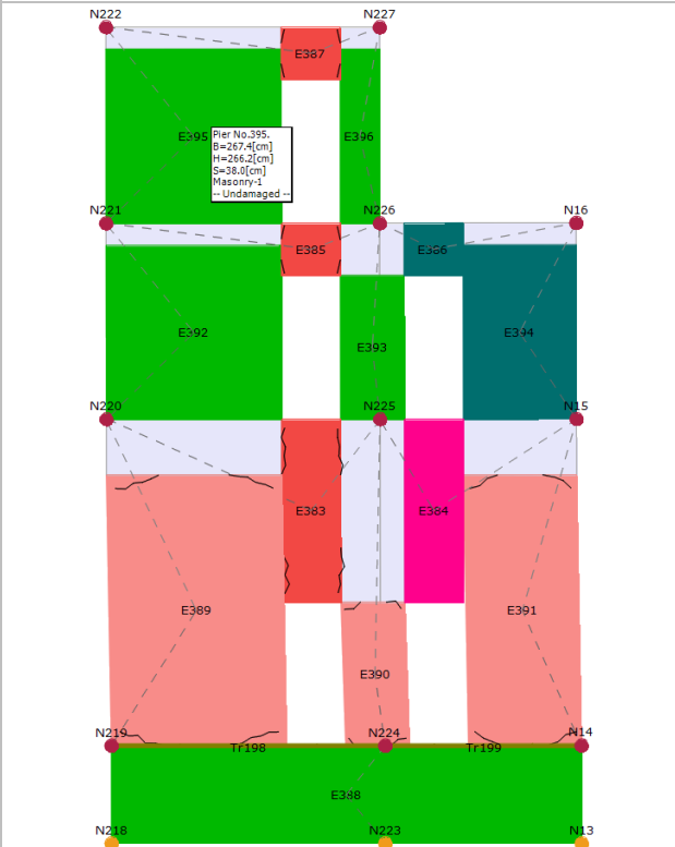
Analysis-24/Mechanism P.32 /Internal masonry /seismic dir.-Y/seismic load =static
