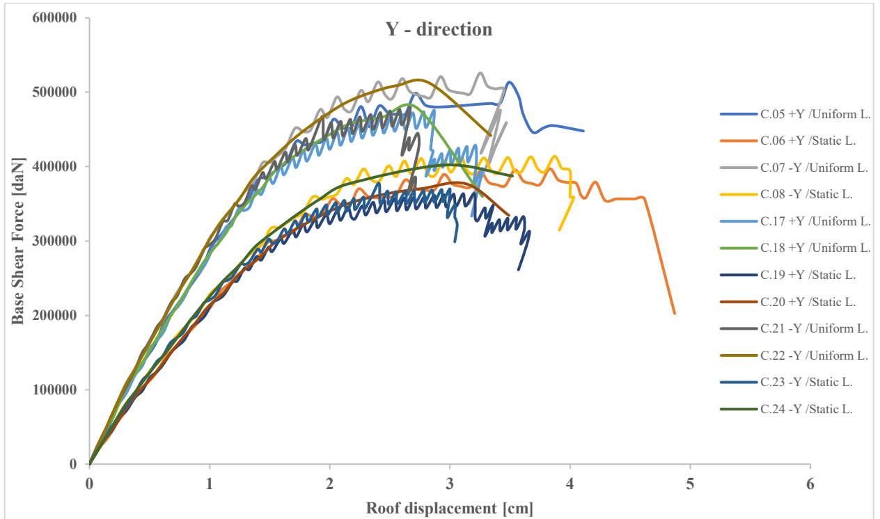
Figure 82. +Y and -Y direction combined capacity diagrams, processed from 3Muri numerical data
