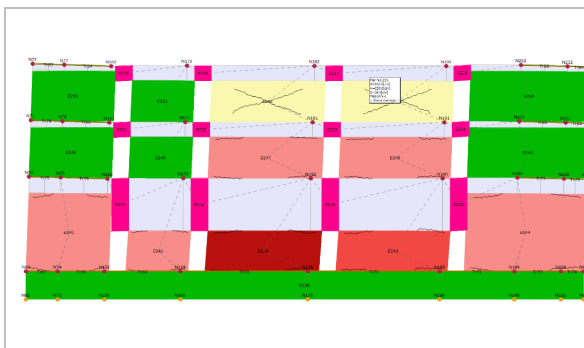
Analysis-02/Mechanism P.11 /South side façade masonry /seismic dir.+X/seismic load =static
