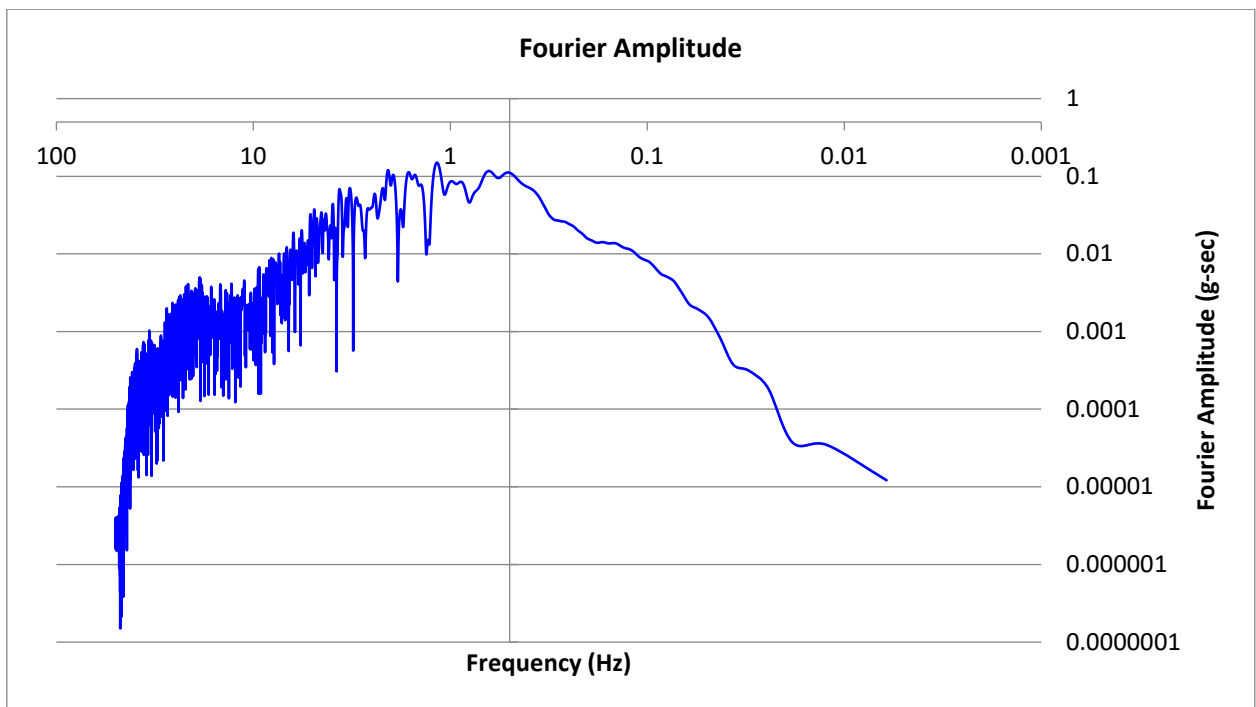
Figure 20. Data related to M.6.4 Durres earthquake fourier amlitude based on frequency and amplitude (Source: IGJEUM)
