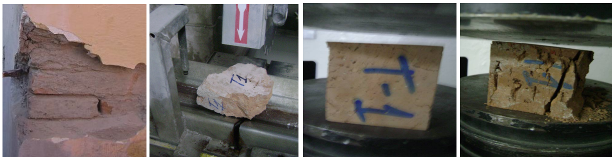
Figure 51. (a) Photo taken while sampling red brick on a perimeter wall panel, inside the basement; (b) sample of red brick preparing for laboratory test, (c) Sample of red brick during the laboratory test in printing, (d) Sample of red brick after completion of the test in compression, at the point of destruction (Altea & geostudio, 2019)
