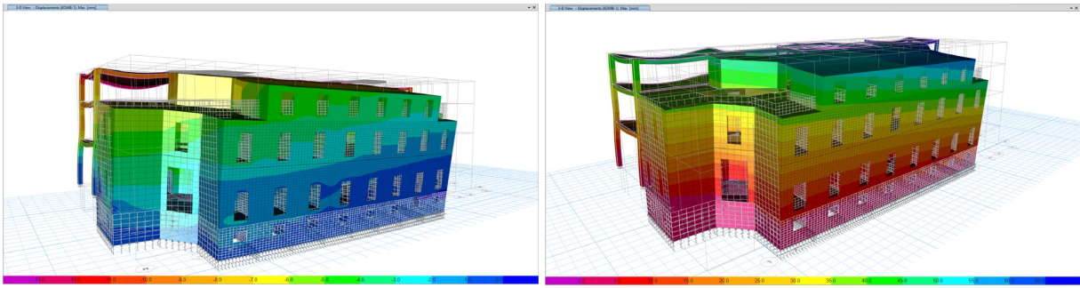
Figure 64. Seismic Displacements according to Combination 1, \Delta x-x and \Delta y-y (ETABS, v.2019)
