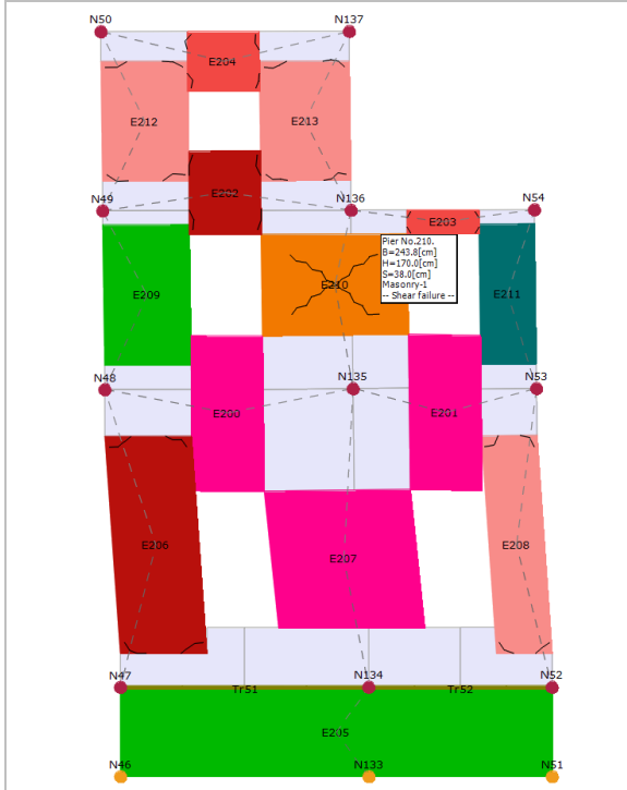
Analysis-24/Mechanism P.22 /Internal masonry /seismic dir.-Y/seismic load =static
