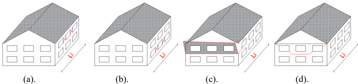
Figure 33. (a) Failure mechanism of Storey shear located on Upper storey, (b) Failure mechanisms related to Storey shear, (c) the failure mechanisms of whole wall overturning, (d) the failure mechanisms related to partial wall overturning.
