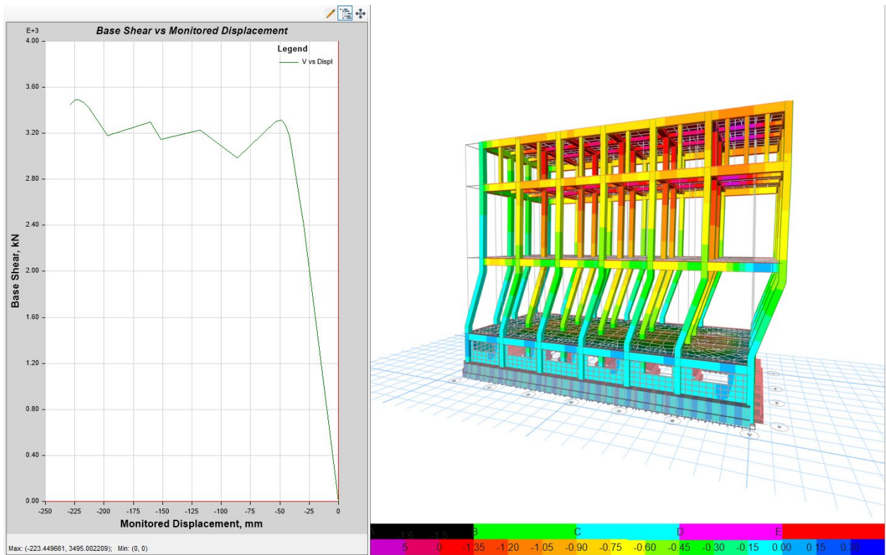
Figure 116. Generation of capacity curve in V- \Delta format according to push-x load, captured in etabs.v19
