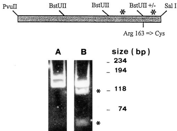
Figure 8. BstU1 restriction endonuclease digestion of the RYR1 PvuII 96–SalI 546-bp cDNA fragment. Lane 1, RYR1 cDNA carrying the Arg163Cys point mutation; lane 2, wild-type RYR1. *The bands of 120 and 54 bp which are replaced by a band of 174 bp in the mutated RYR cDNA. The other two fragments of 144 and 146 bp migrated as a single band ( top ) in this gel.
