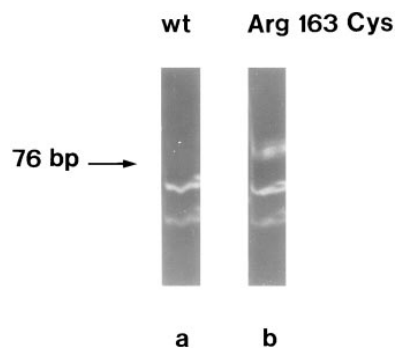
Figure 1. Detection of the RYR1 Arg163Cys mutation in DNA from MHS patient 1. PCR amplification of a 76-bp product was achieved using the primer pairs 457F, 532R. 20% acrylamide gel of (a) digestion of the 76-bp product from a normal control (MHN) and (b) from MHS patient 1 with the restriction endonuclease BstU1. The presence of the mutation Arg163Cys abolishes a BstU1 site. wt, wild-type.
