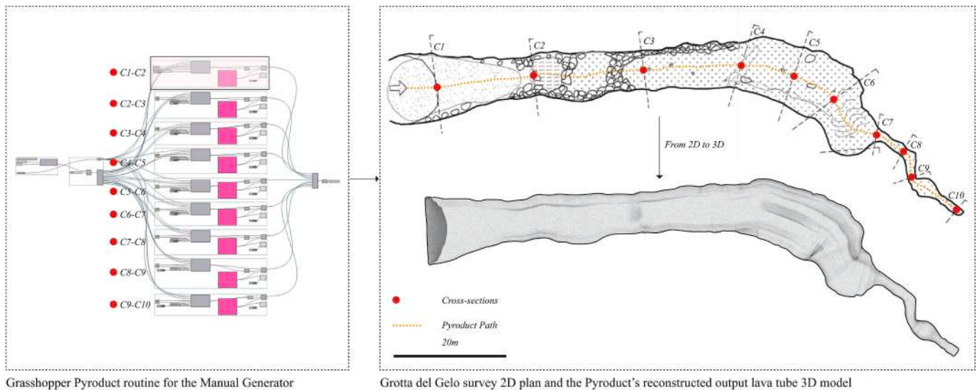
Grasshopper Pyroduct routine for the Manual Generator
