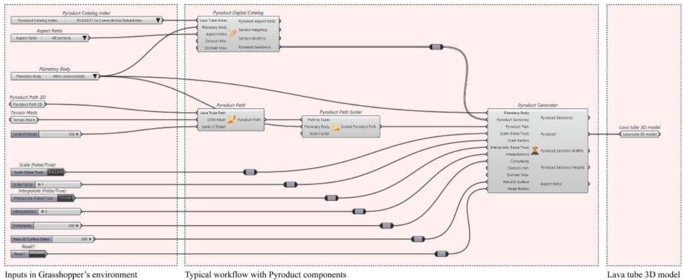
Fig. 6. Above: the complete workflow for turning RS observation into realistic 3D models, through the optional use of GIS software - such as JMARS (Christensen et al., 2009) or QGIS - and Blender to convert .shp format to .dxf, to import it into Rhinoceros, Grasshopper, and Pyproduct, for the generation of the lava tube 3D models. Otherwise, lava tubes can also be generated through lava tube paths directly drawn in Rhinoceros as curves. Below: a typical workflow in Grasshopper with the use of the Pyproduct plug-in. Left: the geometries imported from Rhinoceros and directly defined in the Grasshopper environment are the inputs for Pyproduct, which then can perform its operations and produce as output a lava tube 3D model.
