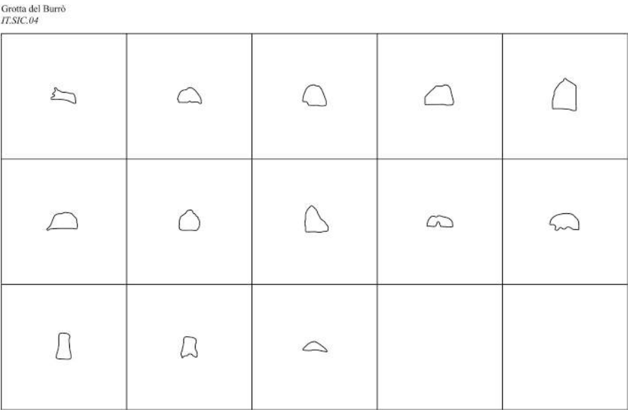
Fig. 4. Example of lava tube cross-sections in the Pyroduct Digital Catalog, Grotta del Burro survey (Giudice and Santi, 1999). Each cell is 35x35m.
