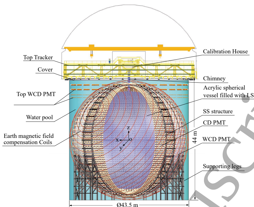
Figure 1: Schematic view of the JUNO detector. The spherical Central Detector (CD) contains 20 ktons of organic Liquid Scintillator (LS) enclosed in an acrylic vessel, serving as neutrino target. It is surrounded by a cylindrical Water Cherenkov Detector (WCD) filled with ultra-pure water. The Top Tracker (TT) positioned above the setup measures crossing muon tracks with high precision.
