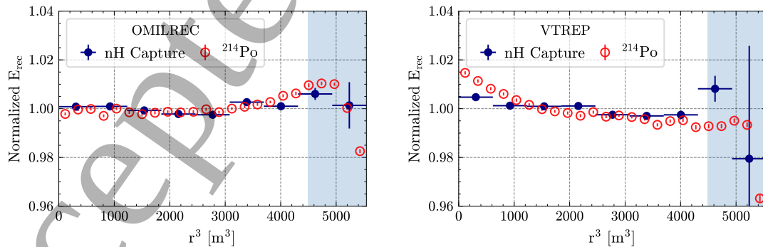
Figure 15: The residual spatial dependence of reconstructed energies for OMILREC (left) and VTREP (right). Reconstructed energy is uniform to better than \pm 1\% in the R < 16.5 m region for OMILREC, while slightly worse for VTREP.
