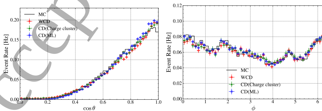
Figure 22: Left: Single muon \cos \theta distribution. Right: Single muon \phi angle distribution. Good agreement between different reconstruction algorithms and simulation is visible.
